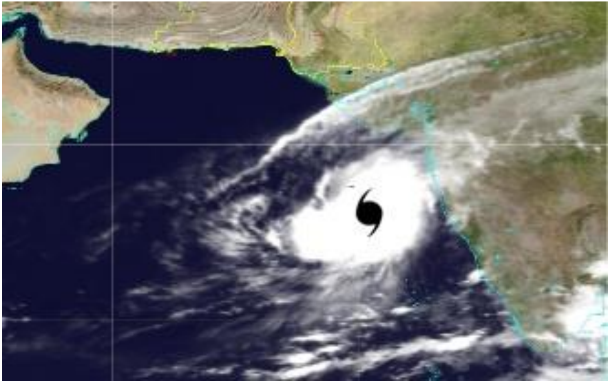
IR Satellite imagery at 1000 PST on 26 October 2019
