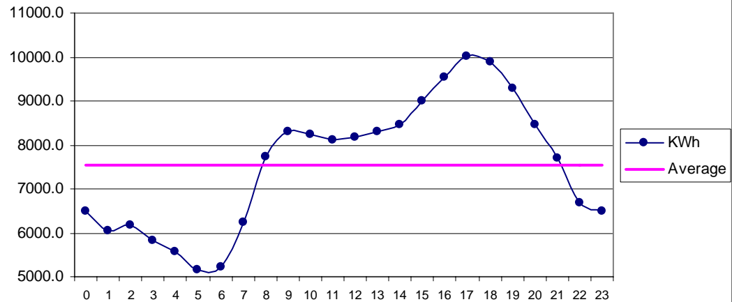
Fig 29 ThanoBula Khan Jun: Diurnal Variation of Wind Genrated Electric Energy Output
