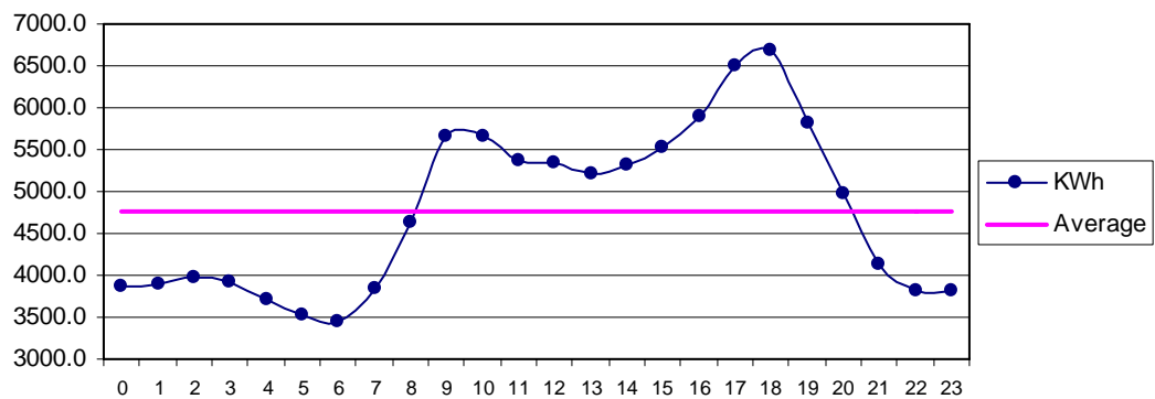
Fig 32 ThanoBula Khan Sep: Diurnal Variation of Wind Genrated Electric Energy Output
