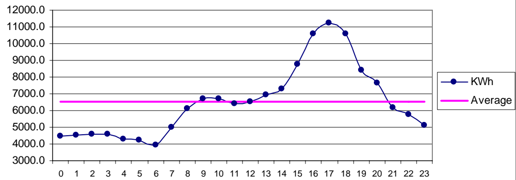
Fig 28 ThanoBula Khan May: Diurnal Variation of Wind Genrated Electric Energy Output
