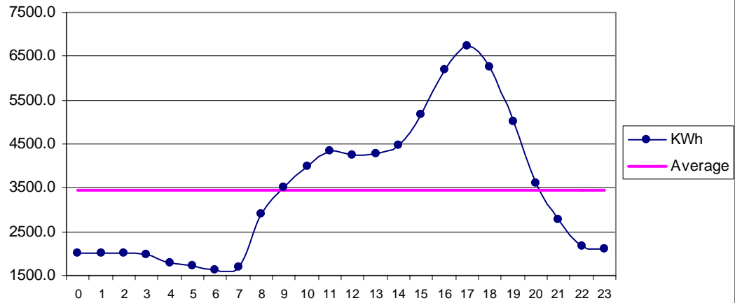
Fig 27 ThanoBula Khan Apr: Diurnal Variation of Wind Genrated Electric Energy Output
