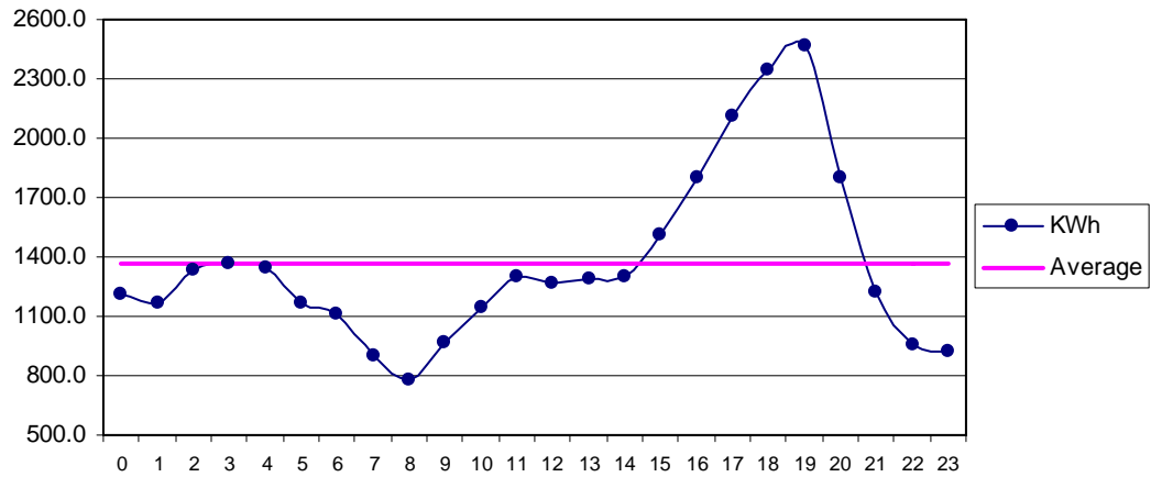
Fig 33 ThanoBula Khan Oct: Diurnal Variation of Wind Genrated Electric Energy Output
