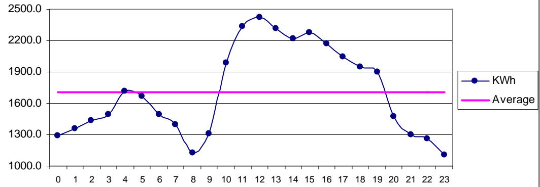
Fig 24 ThanoBula Khan Jan: Diurnal Variation of Wind Genrated Electric Energy Output
