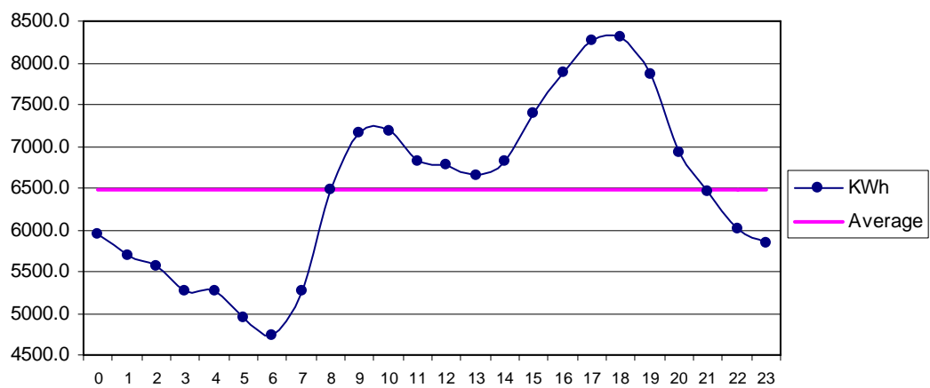
Fig 31 ThanoBula Khan Aug: Diurnal Variation of Wind Genrated Electric Energy Output
