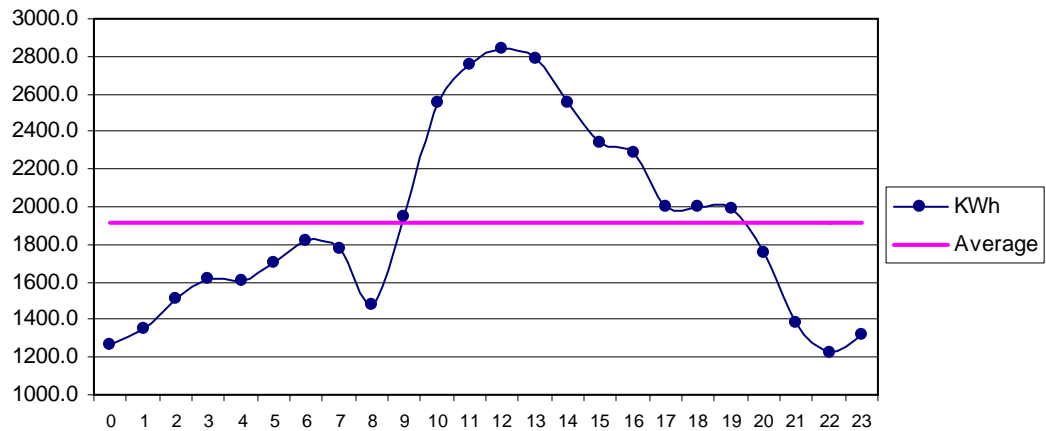
Fig 35 ThanoBula Khan Dec: Diurnal Variation of Wind Genrated Electric Energy Output
