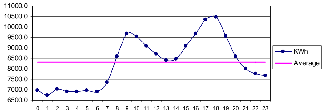
Fig 30 ThanoBula Khan July: Diurnal Variation of Wind Genrated Electric Energy Output
