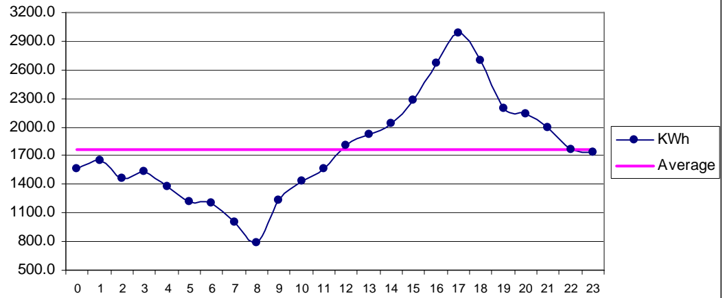
Fig 25 ThanoBula Khan Feb: Diurnal Variation of Wind Genrated Electric Energy Output
