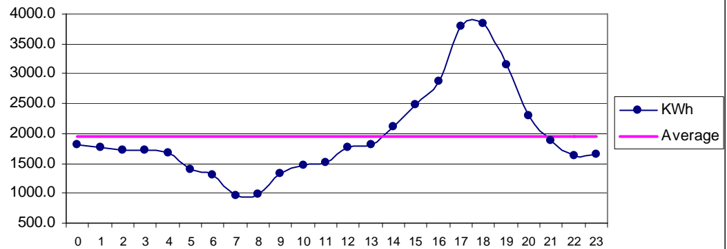
Fig 26 ThanoBula Khan Mar: Diurnal Variation of Wind Genrated Electric Energy Output
