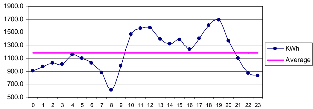
Fig 34 ThanoBula Khan Nov: Diurnal Variation of Wind Genrated Electric Energy Output
