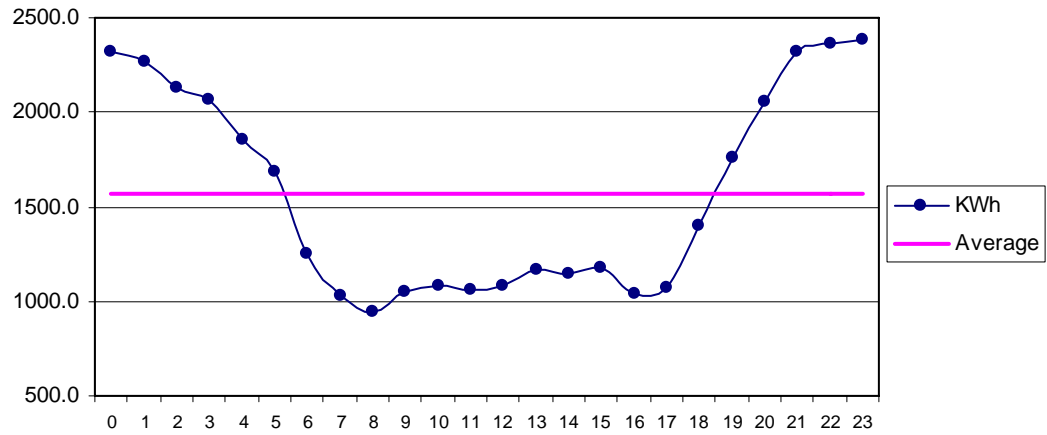
Fig 33 Talhar Oct: Diurnal Variation of Wind Genrated Electric Energy Output
