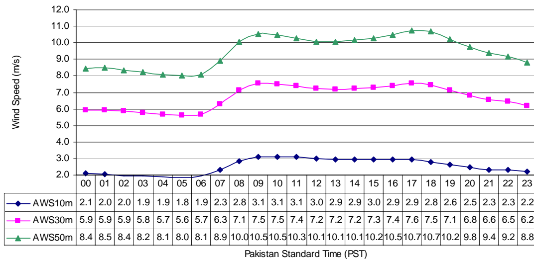
Diurnal Variation of Wind Speed at Talhar (Jun to Aug) in three Years
