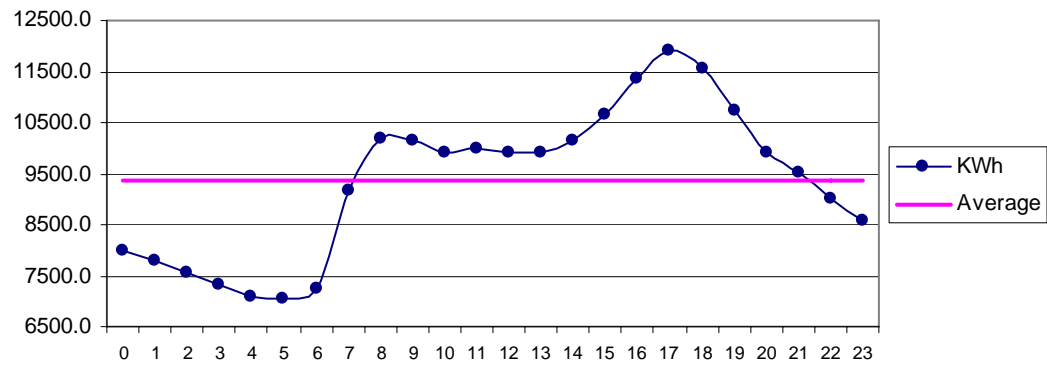
Fig 28 Talhar: Diurnal Variation of Wind Genrated Electric Energy Output
