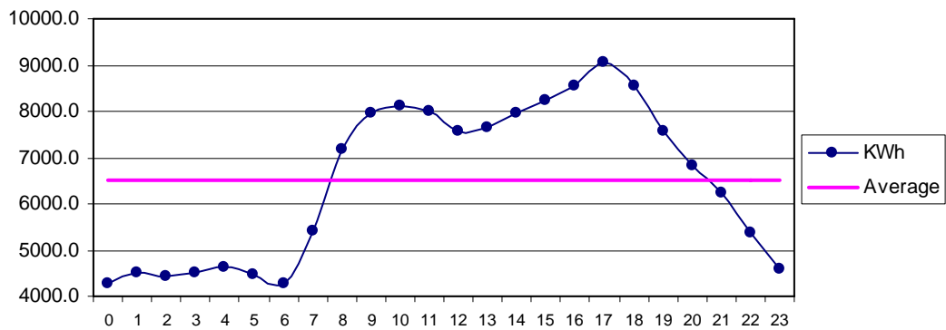
Fig 30 Talhar July: Diurnal Variation of Wind Genrated Electric Energy Output
