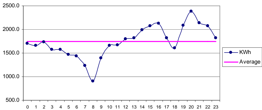
Fig 25 Talhar Feb: Diurnal Variation of Wind Genrated Electric Energy Output
