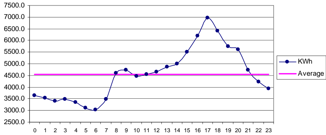
Fig 27 Talhar Apr: Diurnal Variation of Wind Genrated Electric Energy Output
