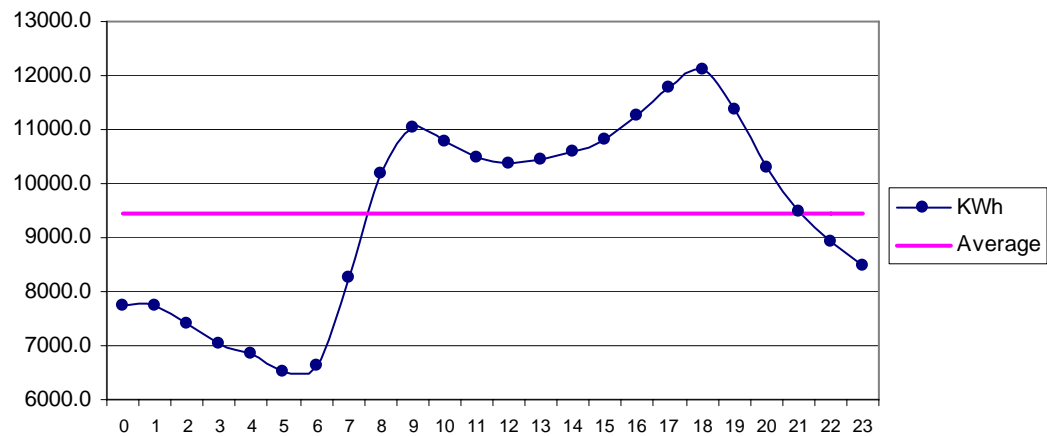
Fig 29 Talhar Jun: Diurnal Variation of Wind Genrated Electric Energy Output
