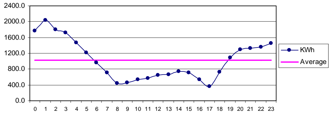
Fig 34 Talhar Nov: Diurnal Variation of Wind Genrated Electric Energy Output
