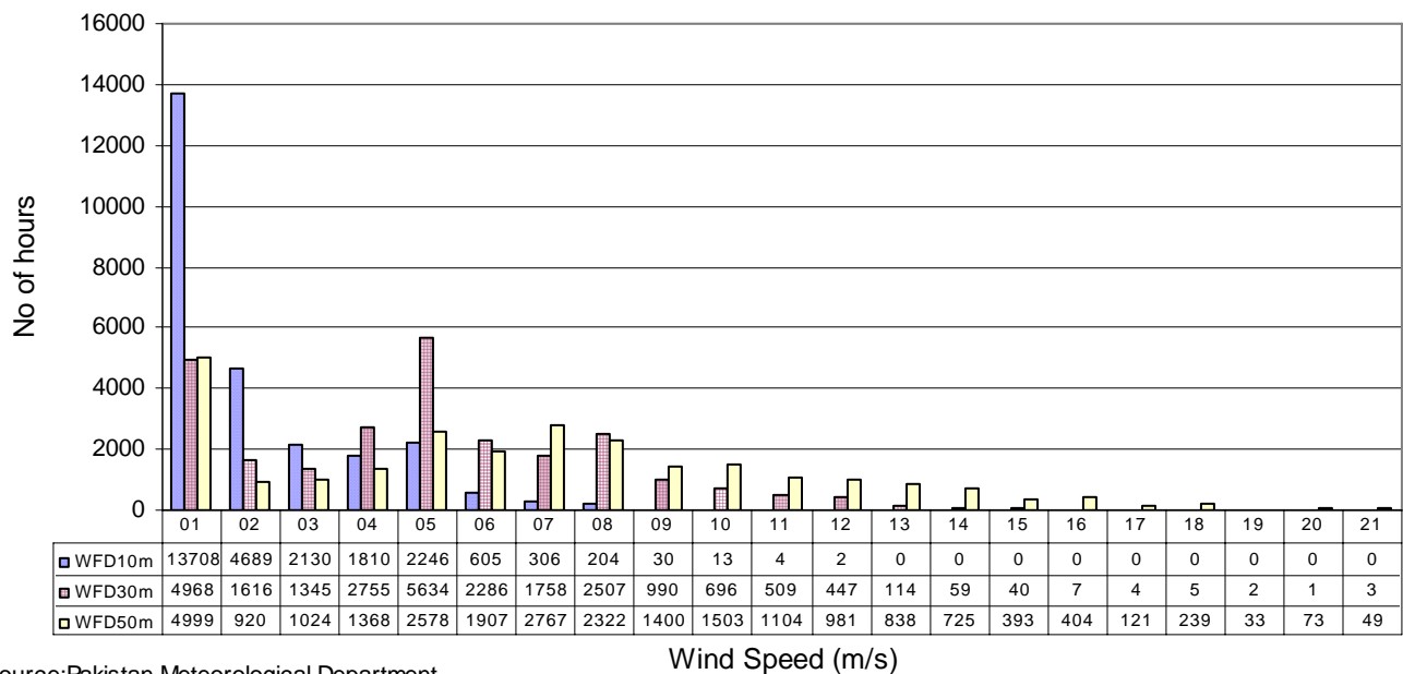
Annual Wind Frequency Distribution at Talhar in three years
