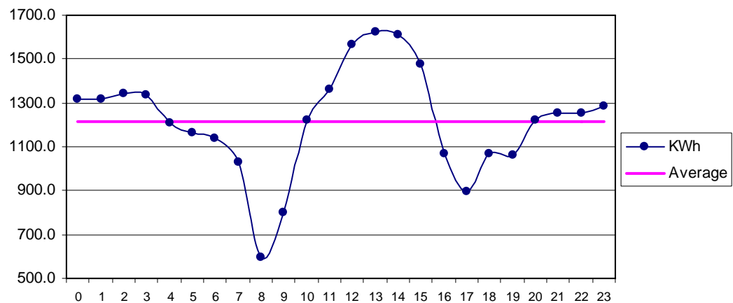
Fig 35 Talhar Dec: Diurnal Variation of Wind Genrated Electric Energy Output
