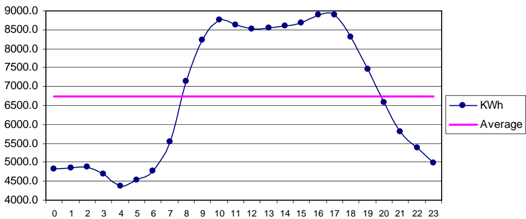
Fig 31 Talhar Aug: Diurnal Variation of Wind Genrated Electric Energy Output
