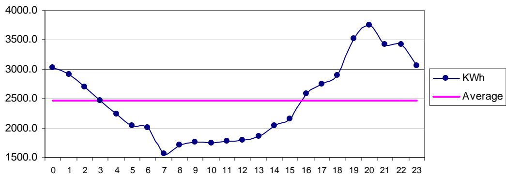
Fig 26 Talhar Mar: Diurnal Variation of Wind Genrated Electric Energy Output
