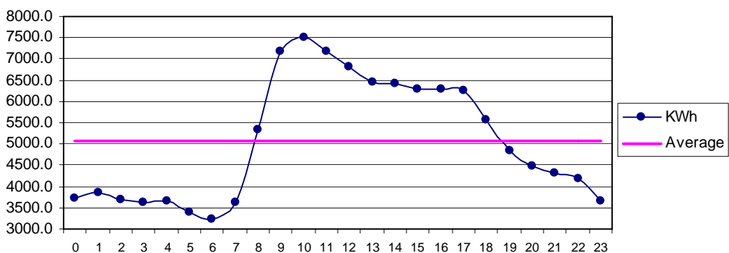
Fig 32 Talhar Sep: Diurnal Variation of Wind Genrated Electric Energy Output
