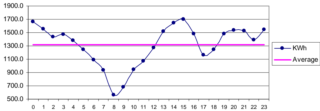
Fig 24 Talhar Jan: Diurnal Variation of Wind Genrated Electric Energy Output
