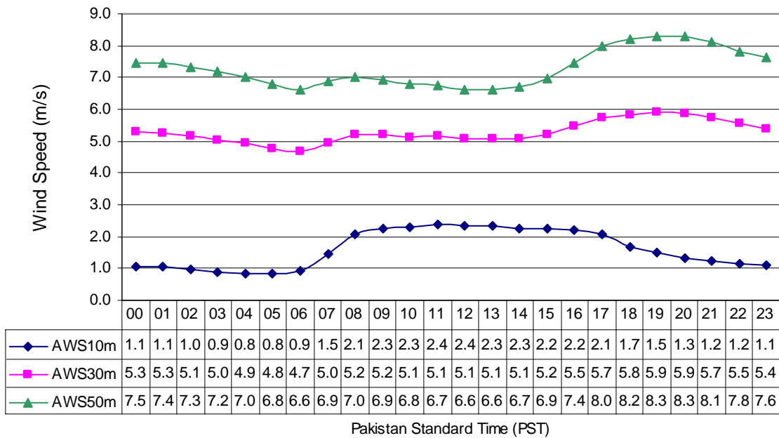
Diurnal Variation of Wind Speed at Talhar (Mar to May) in three Years
