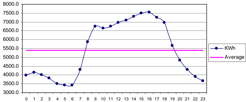
Fig 31 Sajawal Aug: Diurnal Variation of Wind Genrated Electric Energy Output
