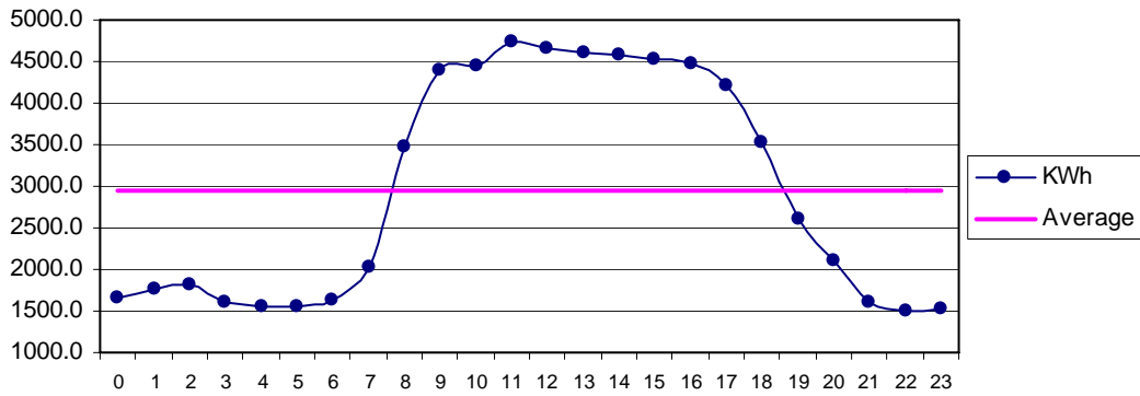
Fig 32 Sajawal Sep: Diurnal Variation of Wind Genrated Electric Energy Output
