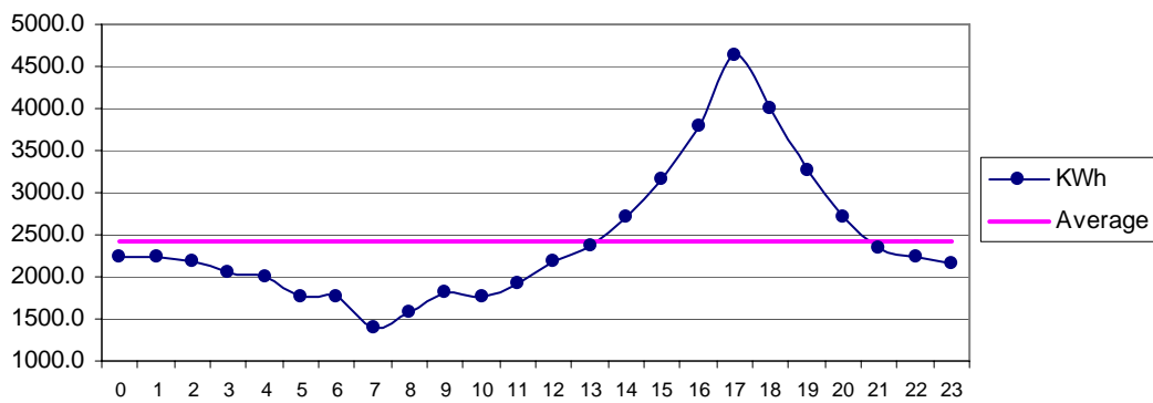
Fig 26 Sajawal Mar: Diurnal Variation of Wind Genrated Electric Energy Output
