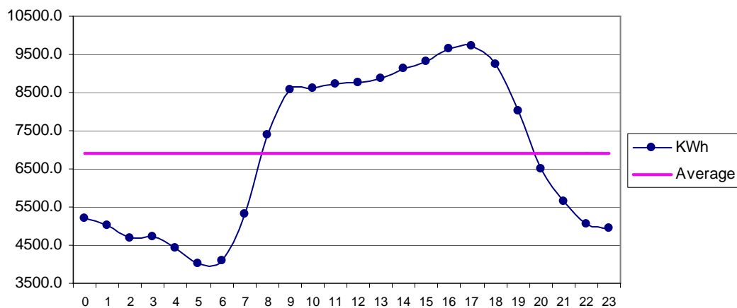
Fig 29 Sajawal Jun: Diurnal Variation of Wind Genrated Electric Energy Output
