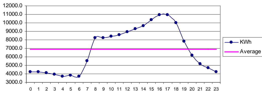
Fig 28 Sajawal May: Diurnal Variation of Wind Genrated Electric Energy Output
