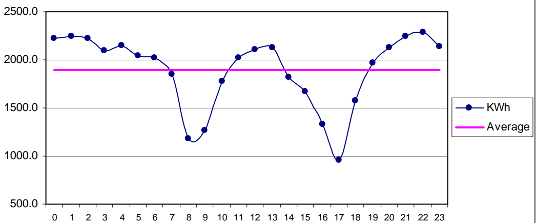
Fig 35 Sajawal Dec: Diurnal Variation of Wind Genrated Electric Energy Output
