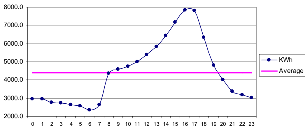
Fig 27 Sajawal Apr: Diurnal Variation of Wind Genrated Electric Energy Output
