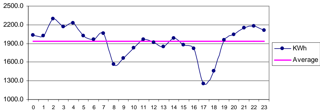
Fig 24 Sajawal Jan: Diurnal Variation of Wind Genrated Electric Energy Output
