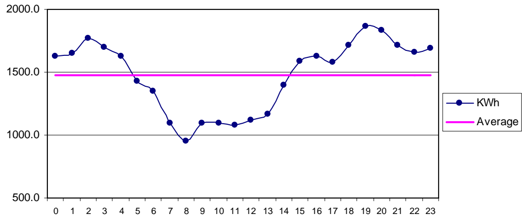
Fig 33 Sajawal Oct: Diurnal Variation of Wind Genrated Electric Energy Output
