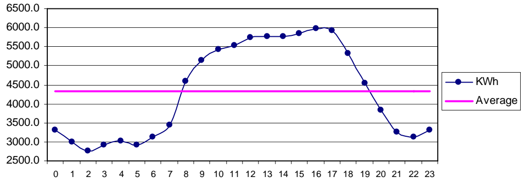
Fig 30 Sajawal July: Diurnal Variation of Wind Genrated Electric Energy Output
