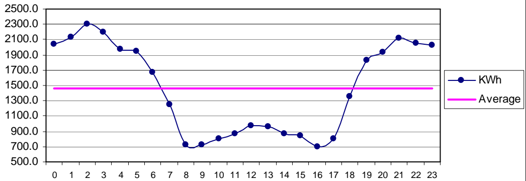
Fig 34 Sajawal Nov: Diurnal Variation of Wind Genrated Electric Energy Output
