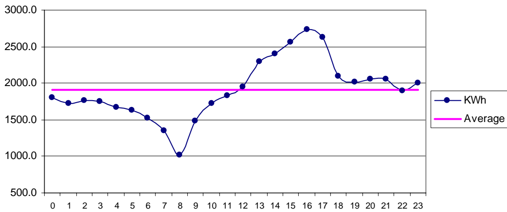
Fig 25 Sajawal Feb: Diurnal Variation of Wind Genrated Electric Energy Output
