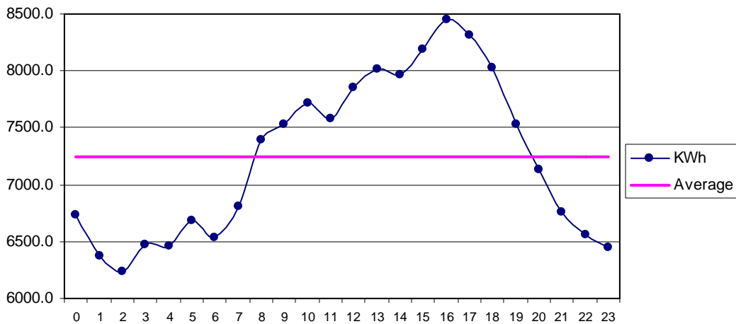
Fig 31 Nooriabad Aug: Diurnal Variation of Wind Genrated Electric Energy Output
