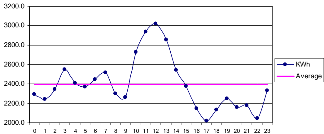
Fig 35 Nooriabad Dec: Diurnal Variation of Wind Genrated Electric Energy Output
