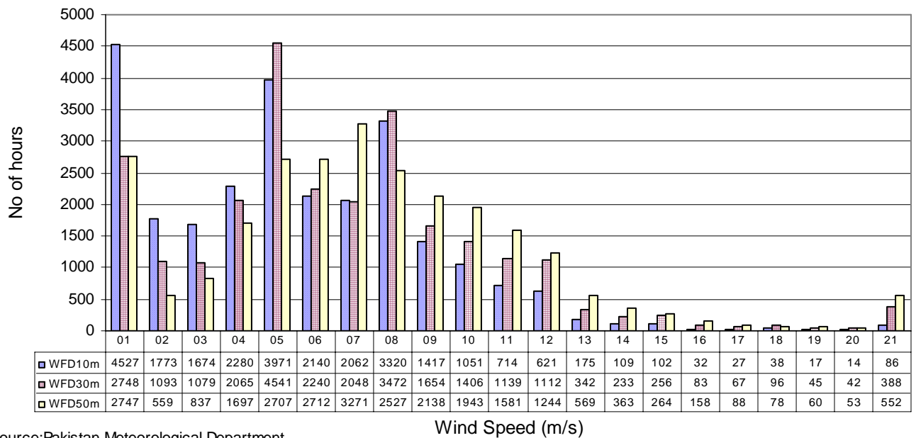
Annual Wind Frequency Distribution at Nooriabad in three years
