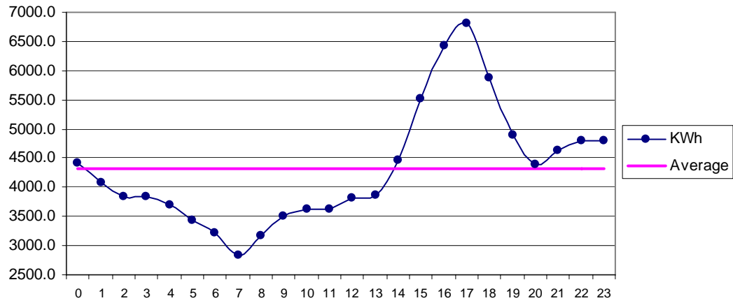
Fig 27 Nooriabad Apr: Diurnal Variation of Wind Genrated Electric Energy Output
