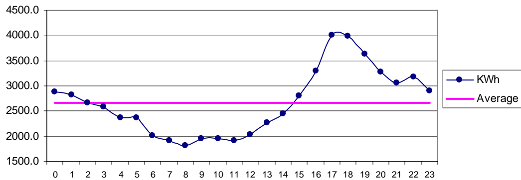
Fig 26 Nooriabad Mar: Diurnal Variation of Wind Genrated Electric Energy Output
