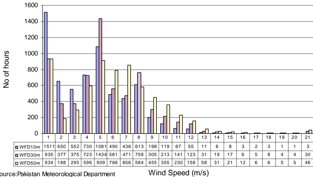
Wind Frequency Distribution at Nooriabad (Sep to Nov) in three years
