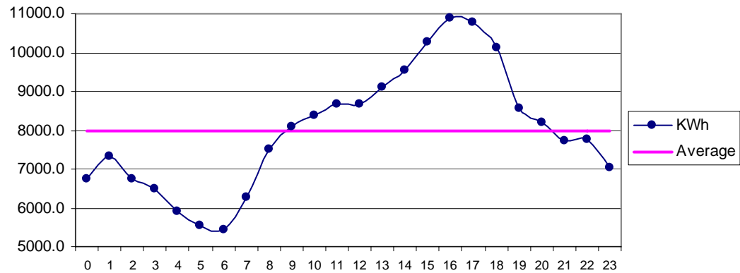
Fig 28 Nooriabad May: Diurnal Variation of Wind Genrated Electric Energy Output
