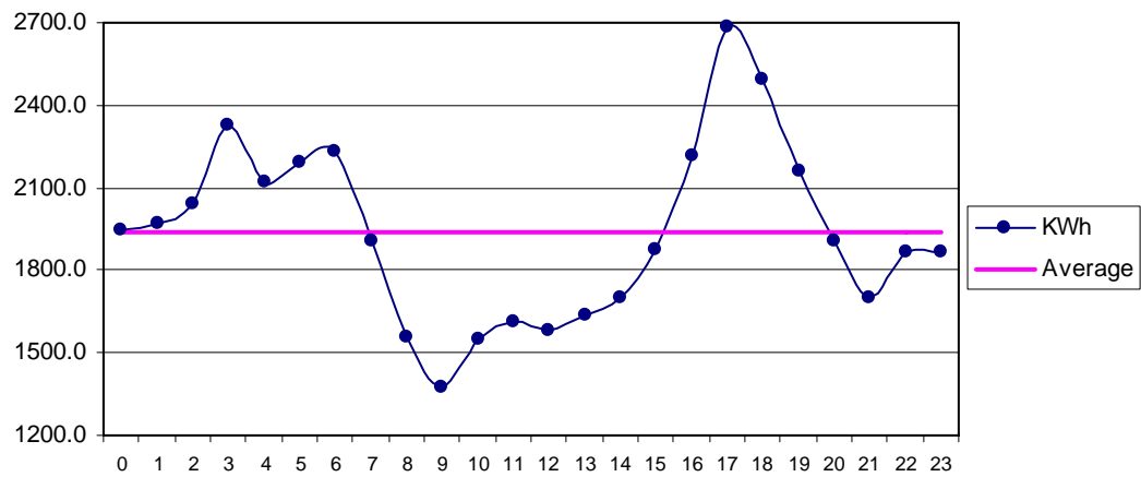
Fig 33 Nooriabad Oct: Diurnal Variation of Wind Genrated Electric Energy Output
