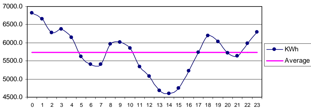
Fig 32 Nooriabad Sep: Diurnal Variation of Wind Genrated Electric Energy Output
