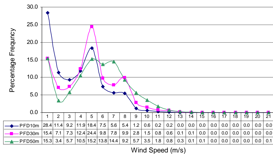
Fig-18 Percentage Wind Frequency Distribution at Nooriabad (Dec to Feb) in three years
