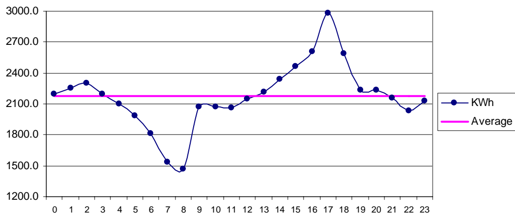
Fig 25 Nooriabad Feb: Diurnal Variation of Wind Genrated Electric Energy Output
