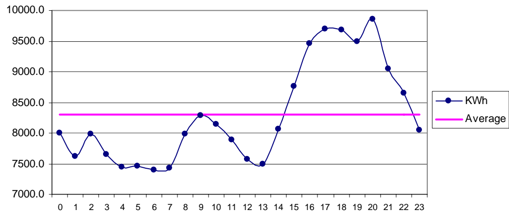
Fig 29 Nooriabad Jun: Diurnal Variation of Wind Genrated Electric Energy Output
