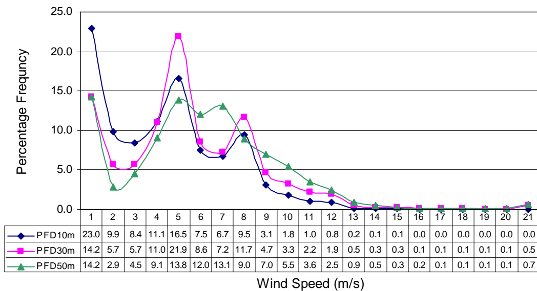
Fig-17 Percentage Wind Frequency Distribution at Nooriabad (Sep to Nov) in three years
