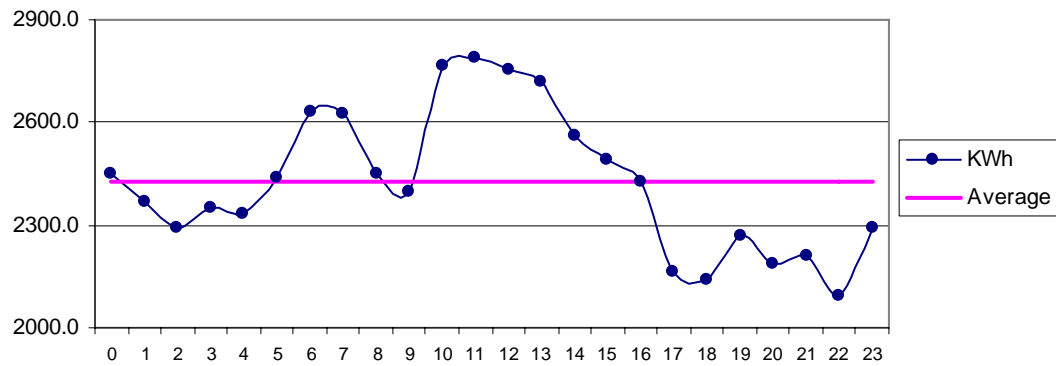
Fig 24 Nooriabad Jan: Diurnal Variation of Wind Genrated Electric Energy Output
