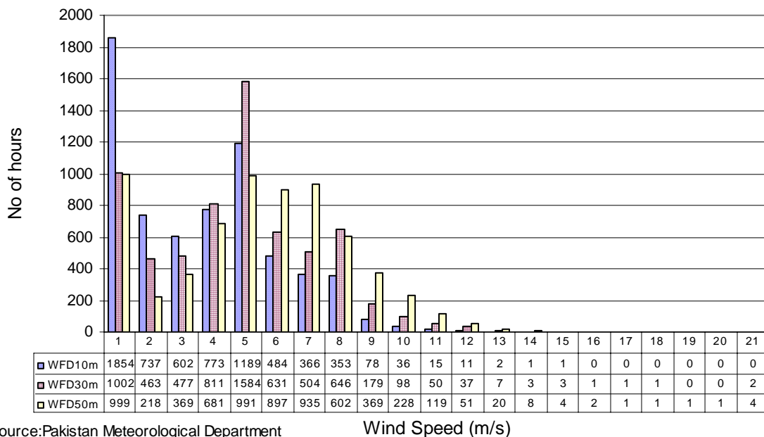
Wind Frequency Distribution at Nooriabad (Dec to Feb) in three years
