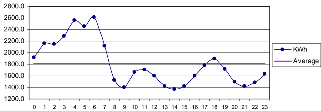
Fig 34 Nooriabad Nov: Diurnal Variation of Wind Genrated Electric Energy Output
