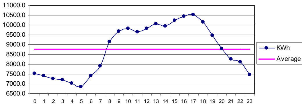
Fig 30 Nooriabad July: Diurnal Variation of Wind Genrated Electric Energy Output
