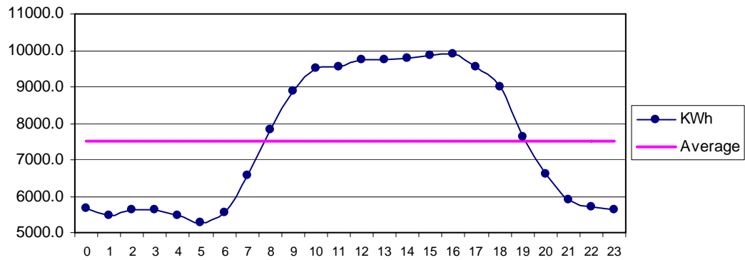
Fig 30 MirPur Sakro July: Diurnal Variation of Wind Genrated Electric Energy Output
