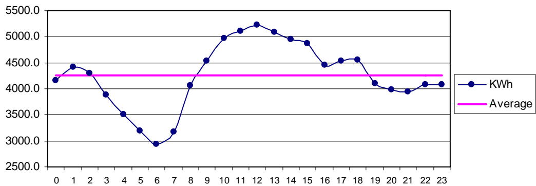
Fig 32 MirPur Sakro Sep: Diurnal Variation of Wind Genrated Electric Energy Output
