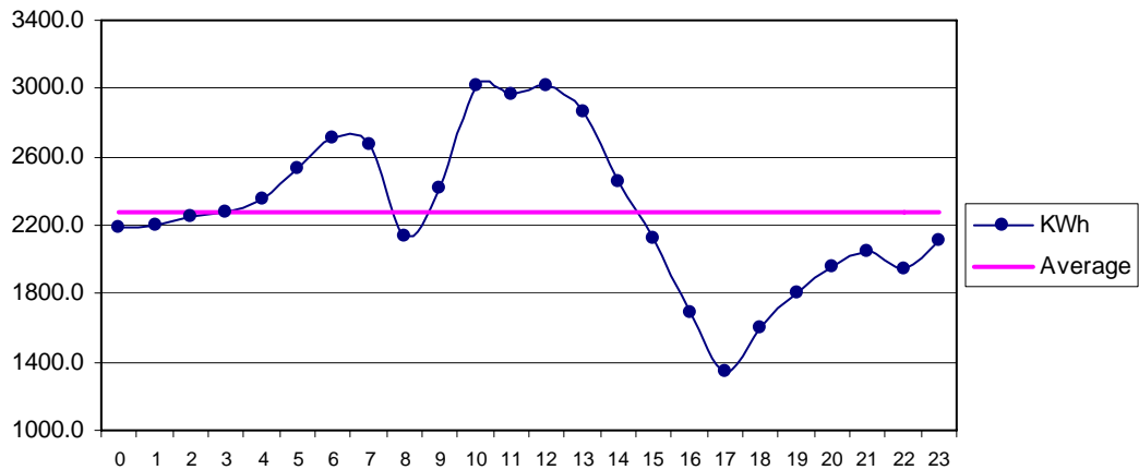
Fig 35 MirPur Sakro Dec: Diurnal Variation of Wind Genrated Electric Energy Output
