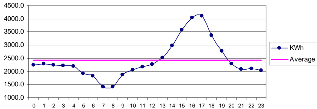
Fig 26 MirPur Sakro Mar: Diurnal Variation of Wind Genrated Electric Energy Output
