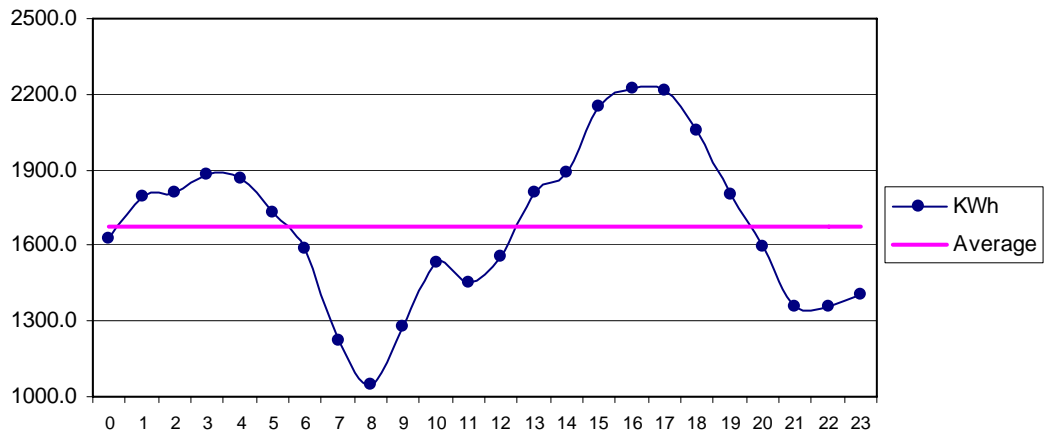
Fig 33 MirPur Sakro Oct: Diurnal Variation of Wind Genrated Electric Energy Output
