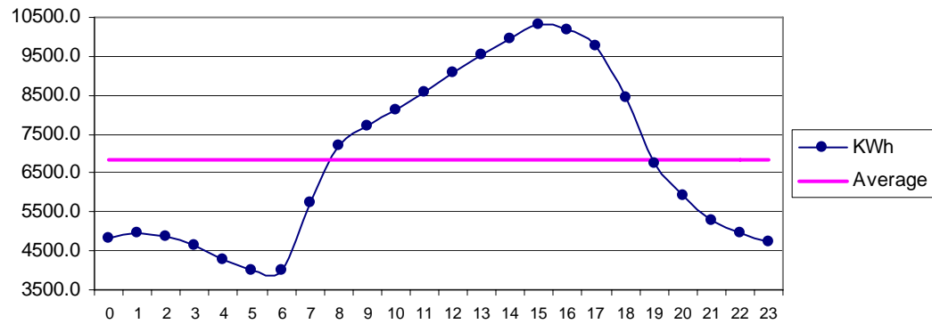
Fig 28 MirPur Sakro May: Diurnal Variation of Wind Genrated Electric Energy Output
