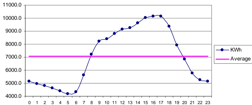
Fig 29 MirPur Sakro Jun: Diurnal Variation of Wind Genrated Electric Energy Output
