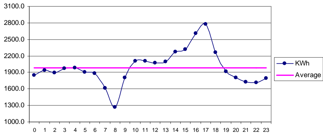
Fig 25 MirPur Sakro Feb: Diurnal Variation of Wind Genrated Electric Energy Output
