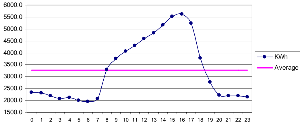
Fig 27 MirPur Sakro Apr: Diurnal Variation of Wind Genrated Electric Energy Output
