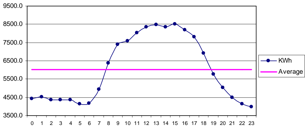
Fig 31 MirPur Sakro Aug: Diurnal Variation of Wind Genrated Electric Energy Output
