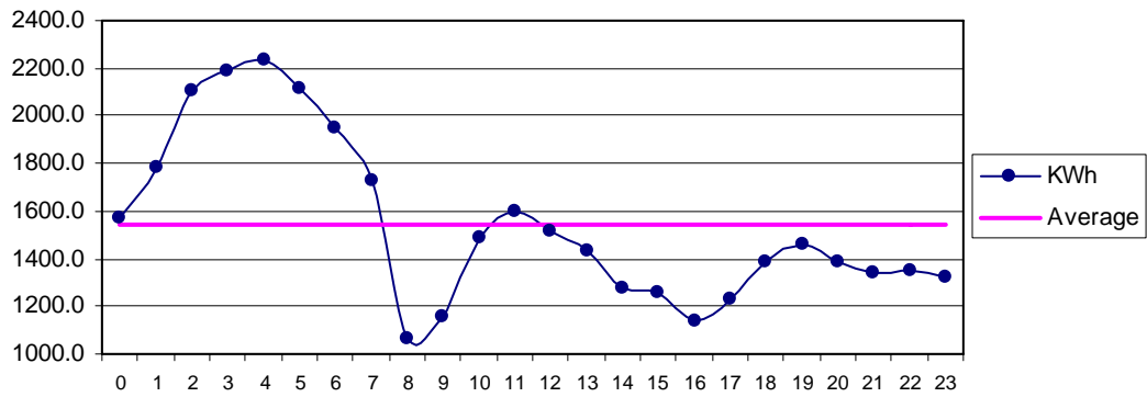
Fig 34 MirPur Sakro Nov: Diurnal Variation of Wind Genrated Electric Energy Output
