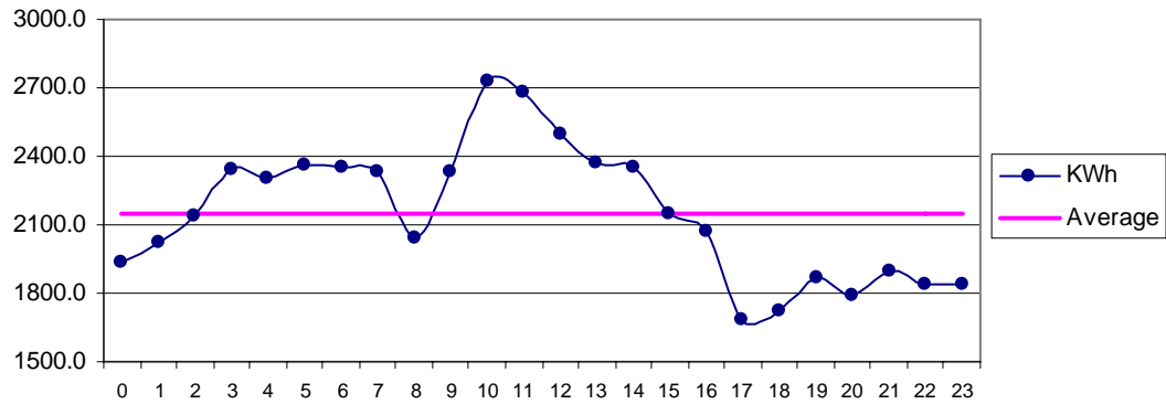
Fig 24 MirPur Sakro Jan: Diurnal Variation of Wind Genrated Electric Energy Output
