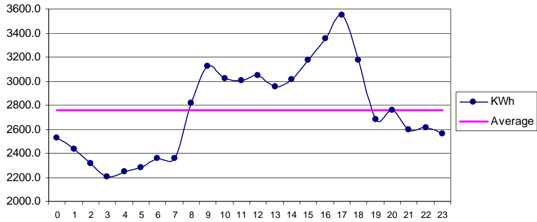
Fig 27 Matli Apr: Diurnal Variation of Wind Genrated Electric Energy Output
