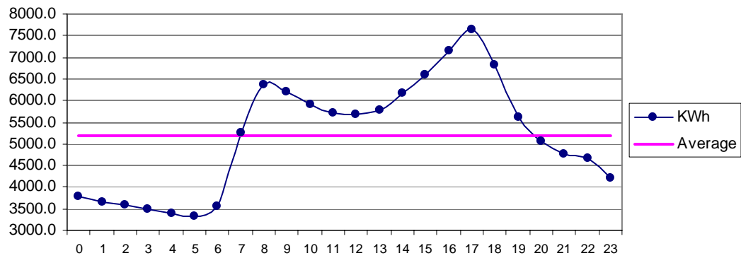
Fig 28 Matli May: Diurnal Variation of Wind Genrated Electric Energy Output
