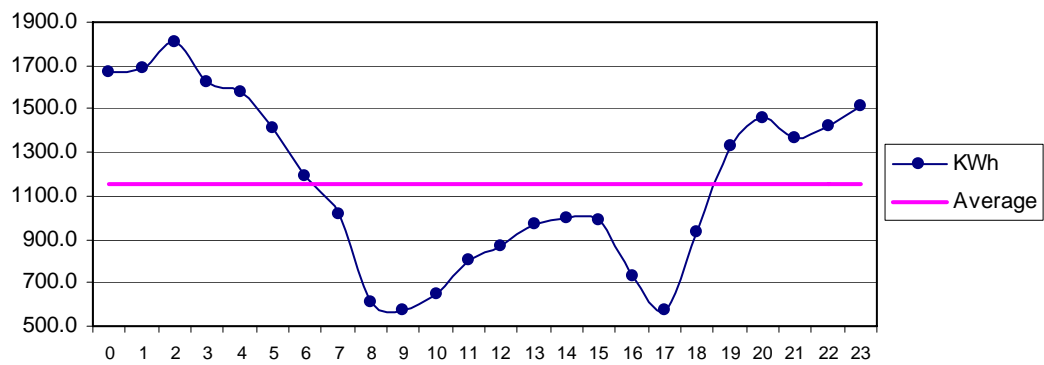
Fig 34 Matli Nov: Diurnal Variation of Wind Genrated Electric Energy Output
