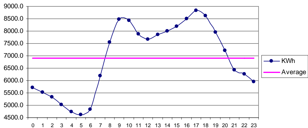
Fig 29 Matli Jun: Diurnal Variation of Wind Genrated Electric Energy Output
