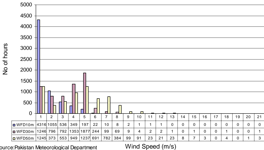
Wind Frequency Distribution at Matli (Dec to Feb) in three years
