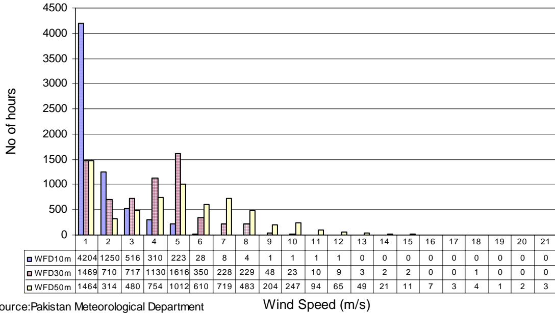
Wind Frequency Distribution at Matli (Sep to Nov) in three years
