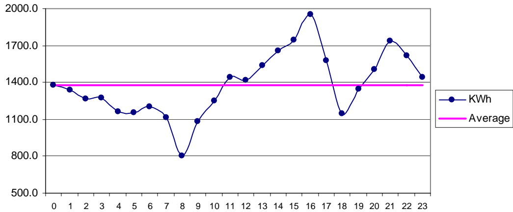
Fig 25 Matli Feb: Diurnal Variation of Wind Genrated Electric Energy Output
