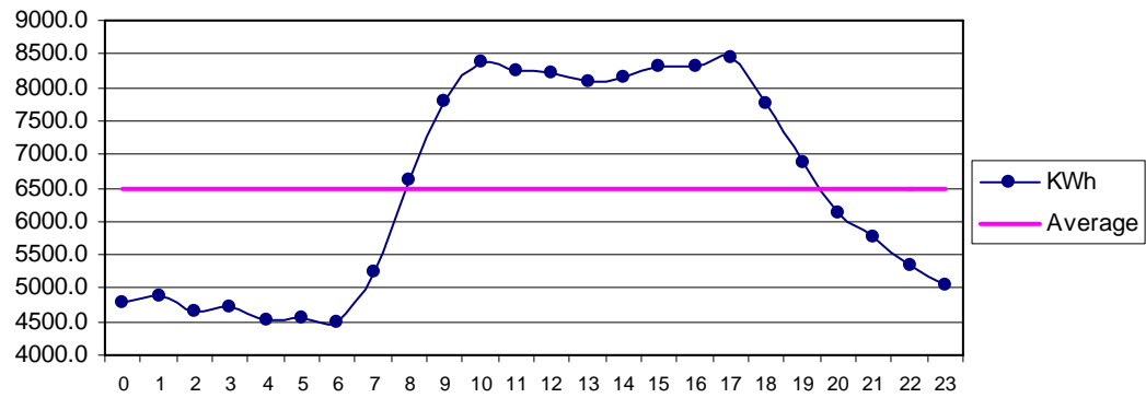
Fig 30 Matli July: Diurnal Variation of Wind Genrated Electric Energy Output
