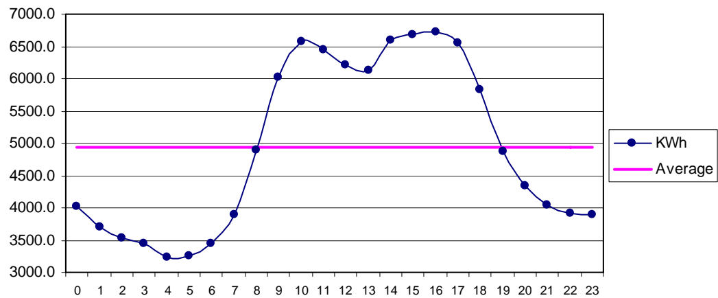
Fig 31 Matli Aug: Diurnal Variation of Wind Genrated Electric Energy Output
