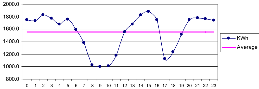
Fig 24 Matli Jan: Diurnal Variation of Wind Genrated Electric Energy Output
