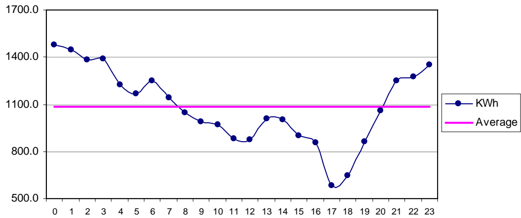
Fig 34 Matli Nov: Diurnal Variation of Wind Genrated Electric Energy Output
