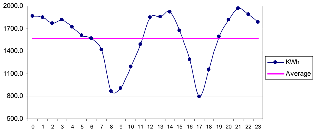
Fig 35 Matli Dec: Diurnal Variation of Wind Genrated Electric Energy Output
