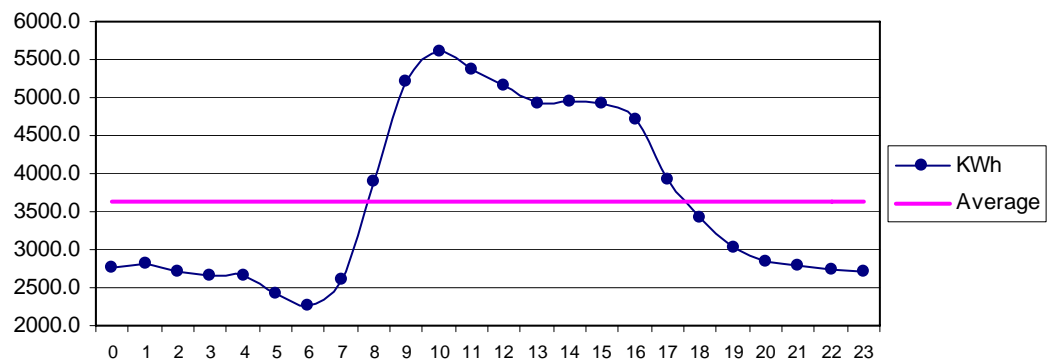
Fig 32 Matli Sep: Diurnal Variation of Wind Genrated Electric Energy Output
