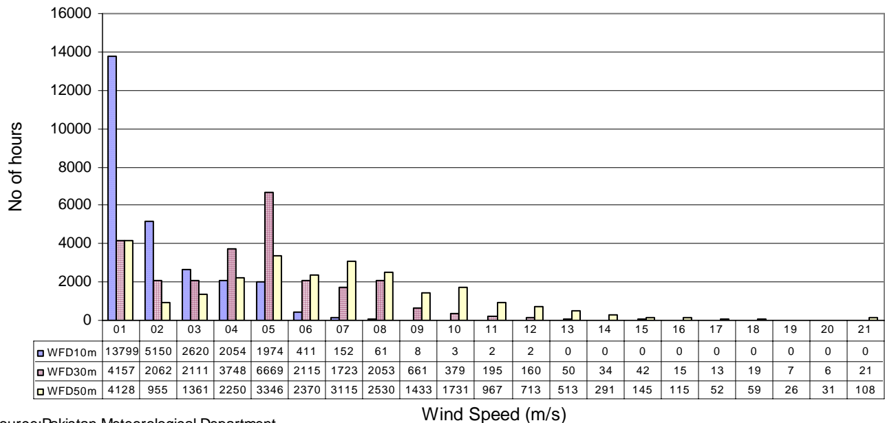
Annual Wind Frequency Distribution at Matli in three years
