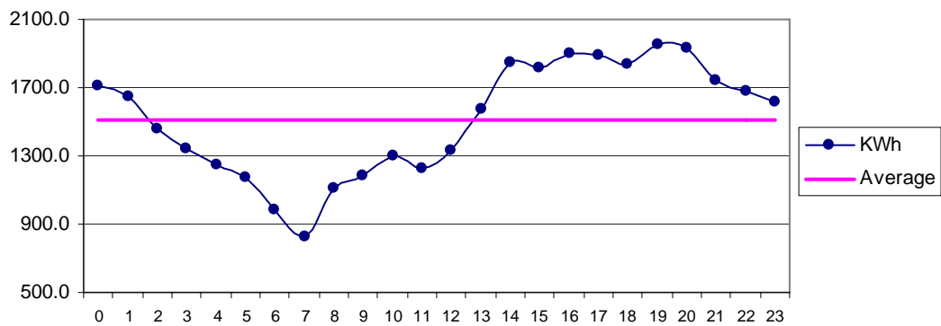
Fig 26 Matli Mar: Diurnal Variation of Wind Genrated Electric Energy Output
