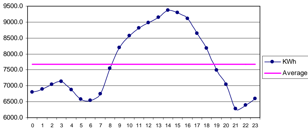
Fig 31 Kati Bandar Aug: Diurnal Variation of Wind Genrated Electric Energy Output
