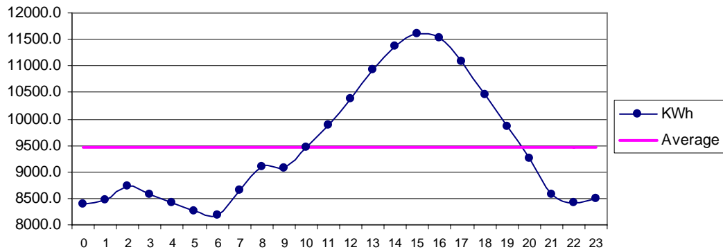
Fig 28 Kati Bandar May: Diurnal Variation of Wind Genrated Electric Energy Output
