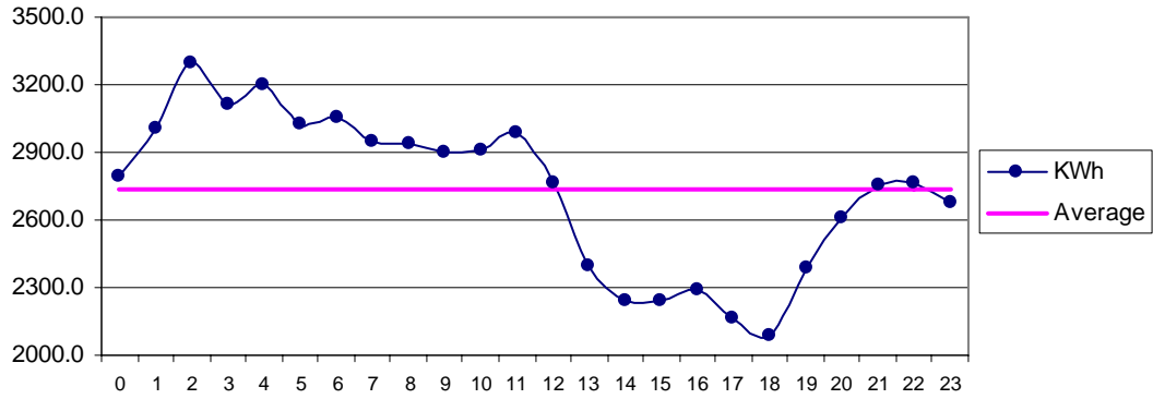
Fig 24 Kati Bandar Jan: Diurnal Variation of Wind Genrated Electric Energy Output
