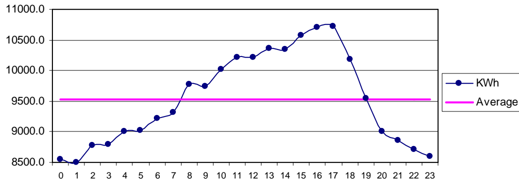
Fig 30 Kati Bandar July: Diurnal Variation of Wind Genrated Electric Energy Output
