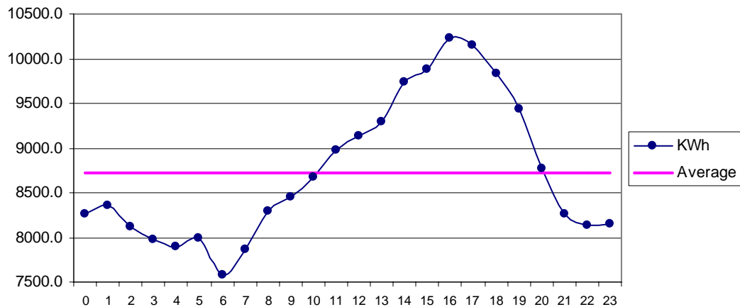
Fig 29 Kati Bandar Jun: Diurnal Variation of Wind Genrated Electric Energy Output
