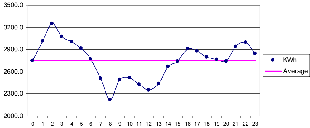
Fig 25 Kati Bandar Feb: Diurnal Variation of Wind Genrated Electric Energy Output
