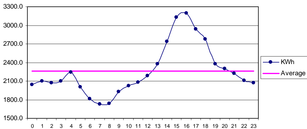
Fig 33 Kati Bandar Oct: Diurnal Variation of Wind Genrated Electric Energy Output
