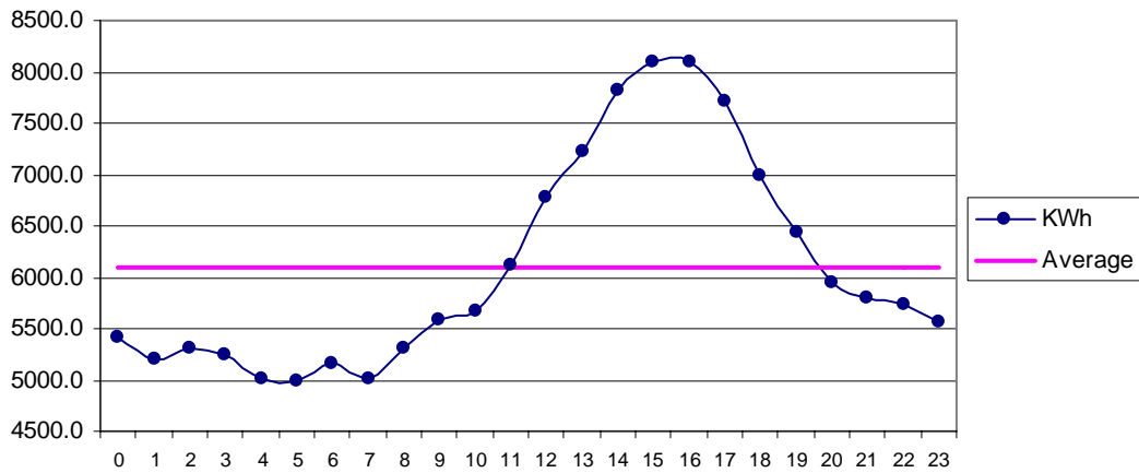
Fig 27 Kati Bandar Apr: Diurnal Variation of Wind Genrated Electric Energy Output
