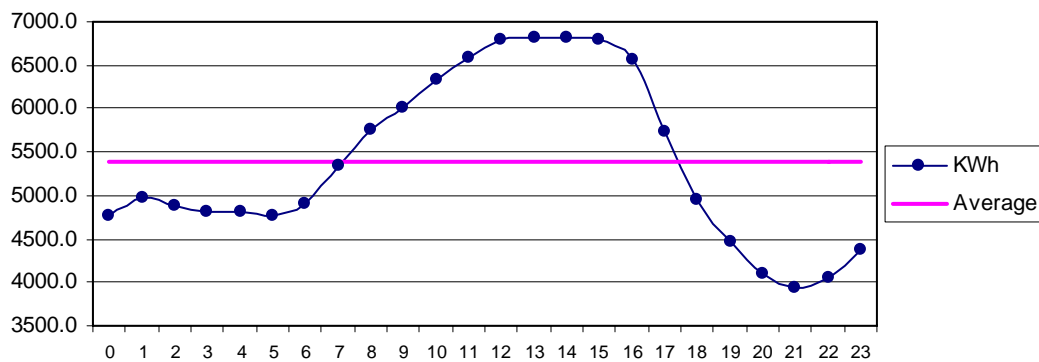
Fig 32 Kati Bandar Sep: Diurnal Variation of Wind Genrated Electric Energy Output
