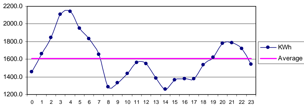
Fig 34 Kati Bandar Nov: Diurnal Variation of Wind Genrated Electric Energy Output
