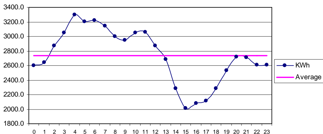
Fig 35 Kati Bandar Dec: Diurnal Variation of Wind Genrated Electric Energy Output
