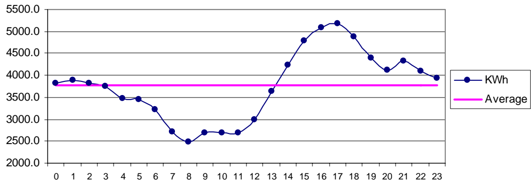
Fig 26 Kati Bandar Mar: Diurnal Variation of Wind Genrated Electric Energy Output
