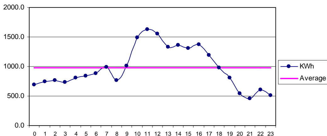
Fig 35 Karachi Dec: Diurnal Variation of Wind Genrated Electric Energy Output
