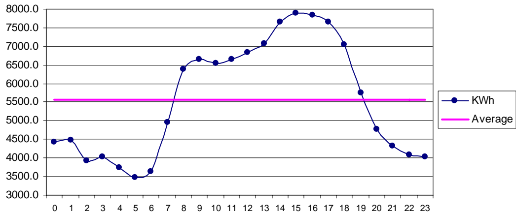
Fig 29 Jati Jun: Diurnal Variation of Wind Genrated Electric Energy Output
