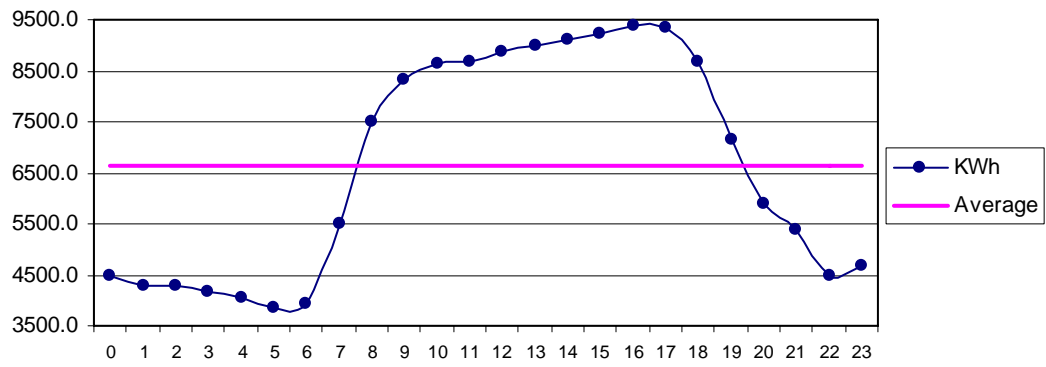
Fig 30 Jati July: Diurnal Variation of Wind Genrated Electric Energy Output
