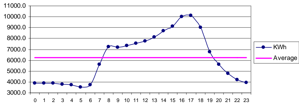
Fig 28 Jati May: Diurnal Variation of Wind Genrated Electric Energy Output
