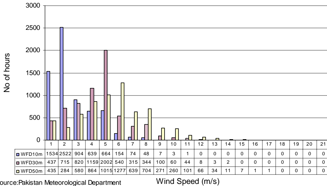
Wind Frequency Distribution at Jati (Sep to Nov) in three years
