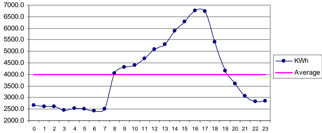
Fig 27 Jati Apr: Diurnal Variation of Wind Genrated Electric Energy Output
