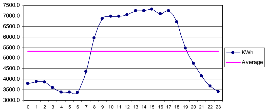
Fig 31 Jati Aug: Diurnal Variation of Wind Genrated Electric Energy Output
