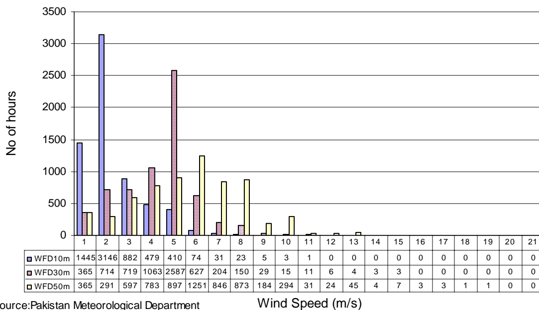
Wind Frequency Distribution at Jati (Dec to Feb) in three years
