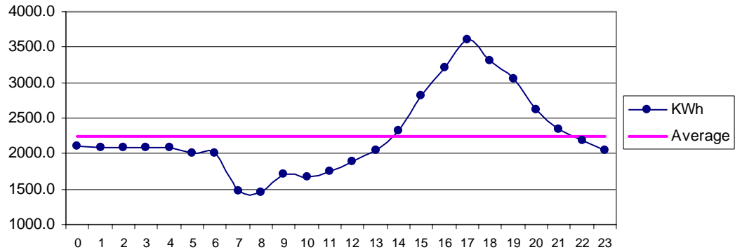
Fig 26 Jati Mar: Diurnal Variation of Wind Genrated Electric Energy Output
