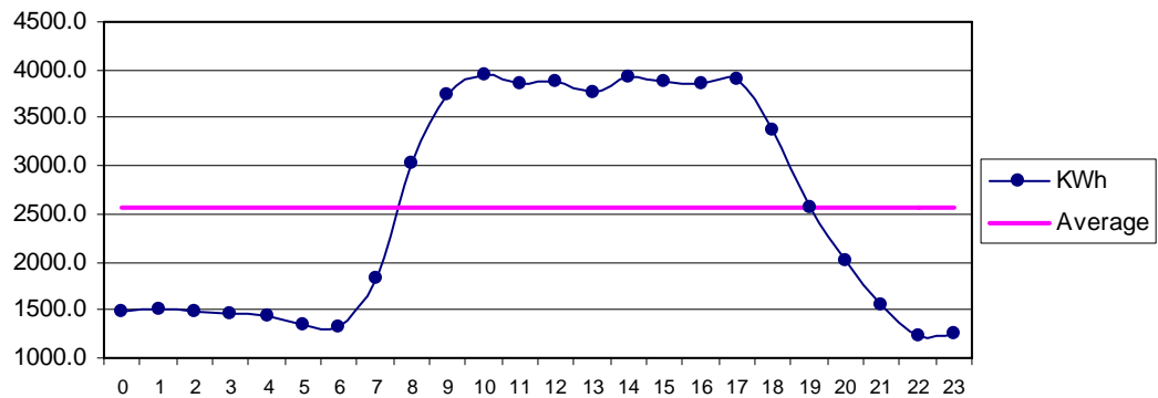
Fig 32 Jati Sep: Diurnal Variation of Wind Genrated Electric Energy Output
