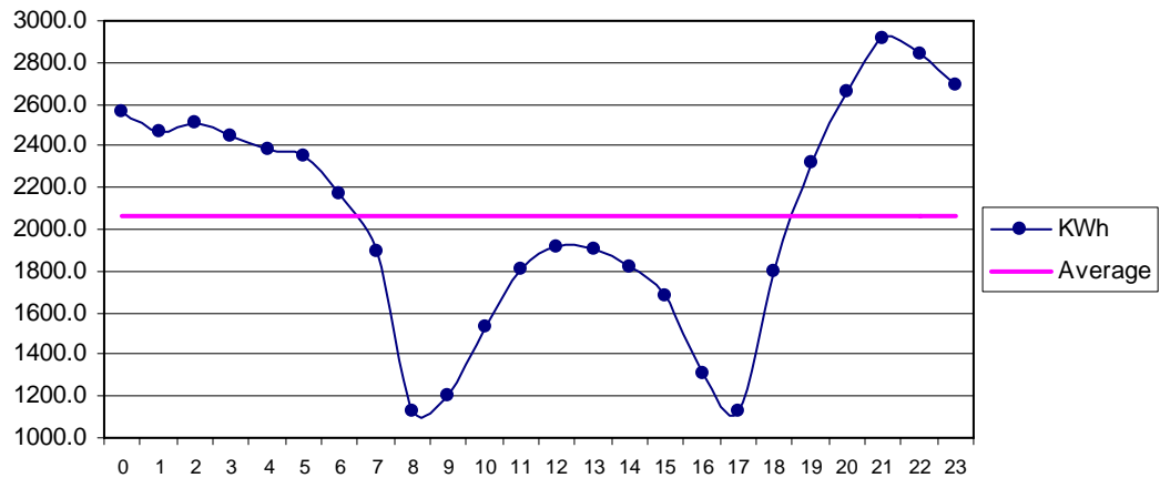
Fig 35 Jati Dec: Diurnal Variation of Wind Genrated Electric Energy Output
