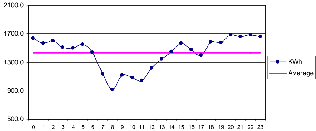
Fig 33 Jati Oct: Diurnal Variation of Wind Genrated Electric Energy Output
