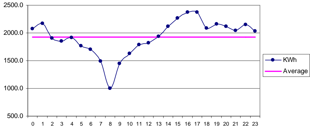
Fig 25 Jati Feb: Diurnal Variation of Wind Genrated Electric Energy Output
