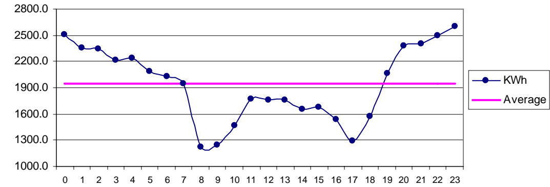
Fig 24 Jati Jan: Diurnal Variation of Wind Genrated Electric Energy Output
