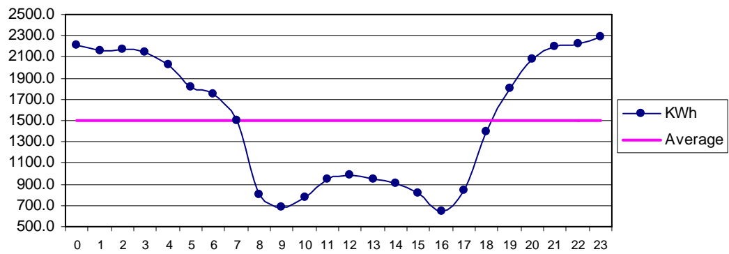
Fig 34 Jati Nov: Diurnal Variation of Wind Genrated Electric Energy Output
