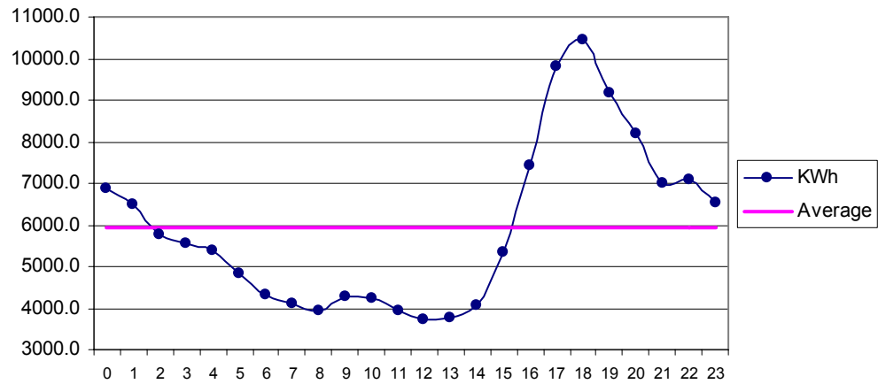
Fig 27 Jamshoro Apr: Diurnal Variation of Wind Genrated Electric Energy Output
