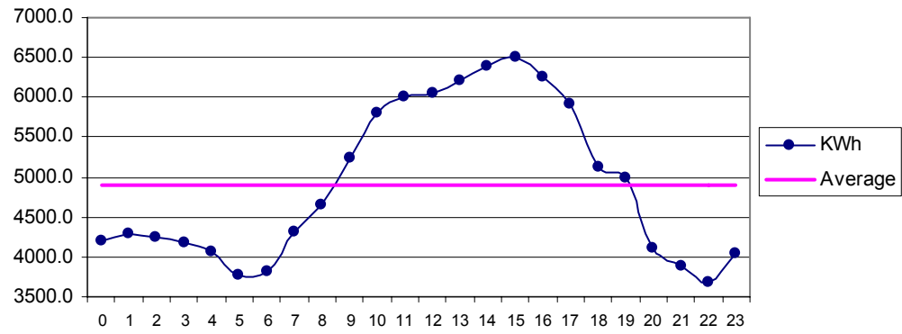
Fig 24 Jamshoro Jan: Diurnal Variation of Wind Genrated Electric Energy Output
