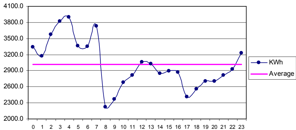
Fig 35 Jamshoro Dec: Diurnal Variation of Wind Genrated Electric Energy Output
