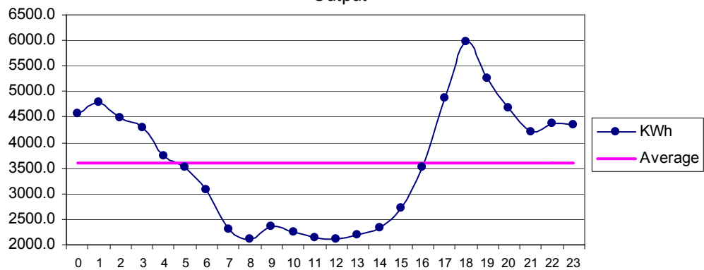
Fig 26 Jamshoro Mar: Diurnal Variation of Wind Genrated Electric Energy Output
