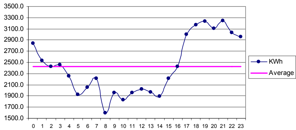
Fig 25 Jamshoro Feb: Diurnal Variation of Wind Genrated Electric Energy Output
