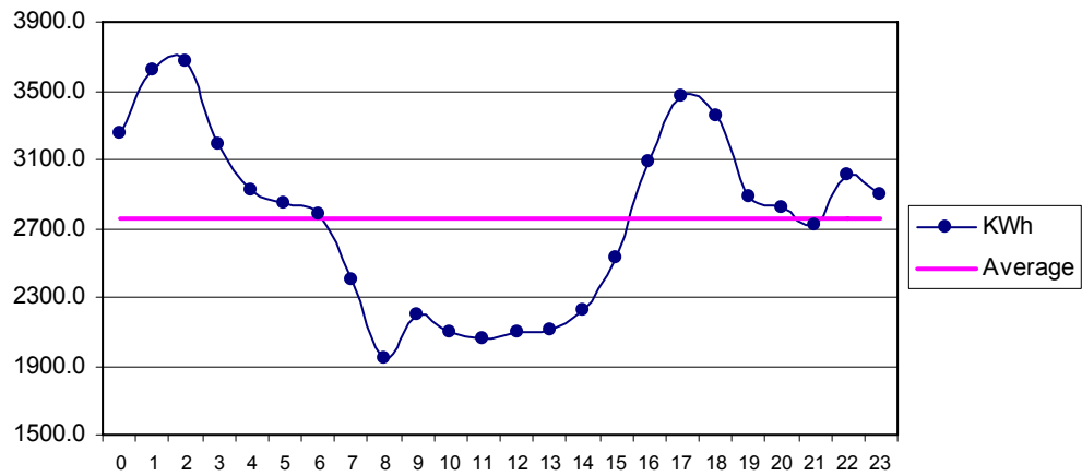
Fig 33 Jamshoro Oct: Diurnal Variation of Wind Genrated Electric Energy Output
