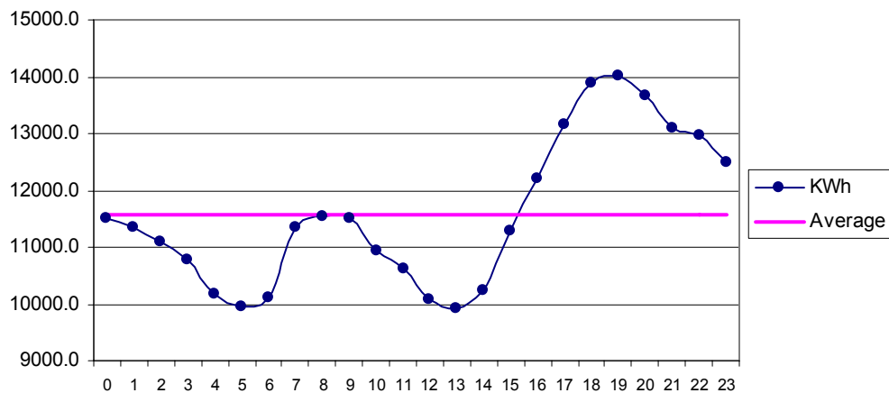
Fig 29 Jamshoro Jun: Diurnal Variation of Wind Genrated Electric Energy Output
