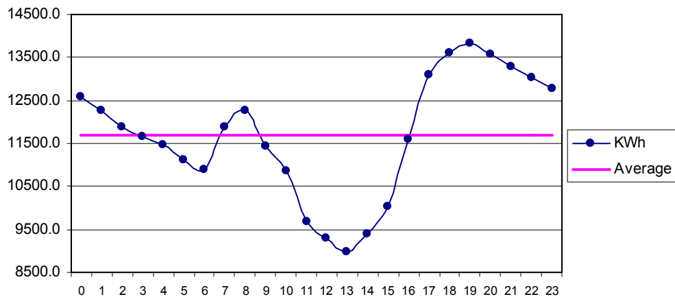
Fig 31 Jamshoro Aug: Diurnal Variation of Wind Genrated Electric Energy Output
