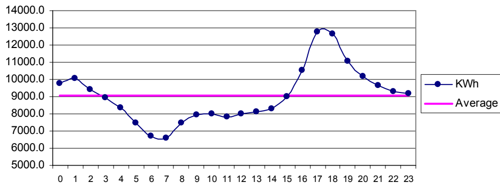
Fig 28 Jamshoro May: Diurnal Variation of Wind Genrated Electric Energy Output
