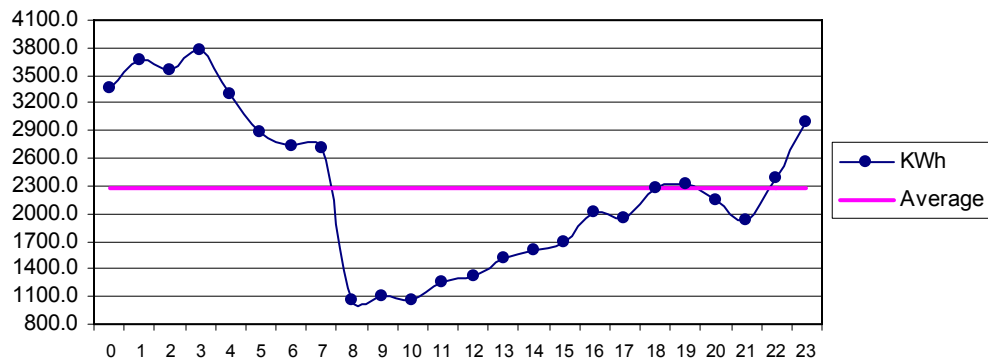
Fig 34 Jamshoro Nov: Diurnal Variation of Wind Genrated Electric Energy Output
