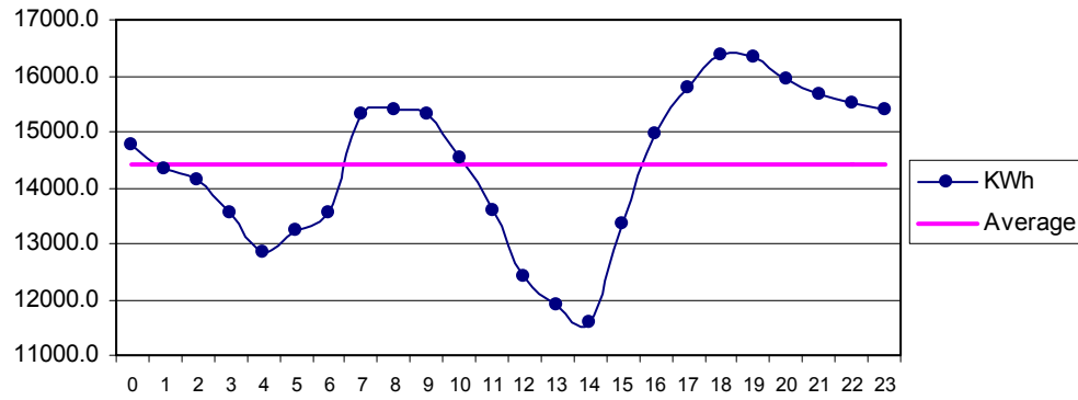
Fig 30 Jamshoro July: Diurnal Variation of Wind Genrated Electric Energy Output
