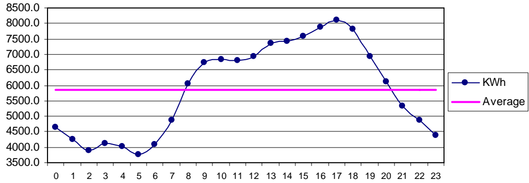
Fig 30 Golarchi July: Diurnal Variation of Wind Genrated Electric Energy Output
