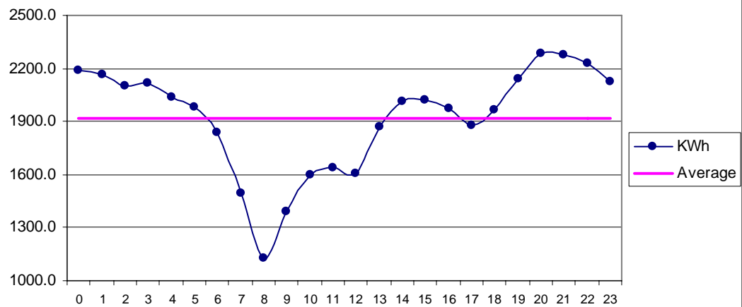
Fig 25 Golarchi Feb: Diurnal Variation of Wind Genrated Electric Energy Output
