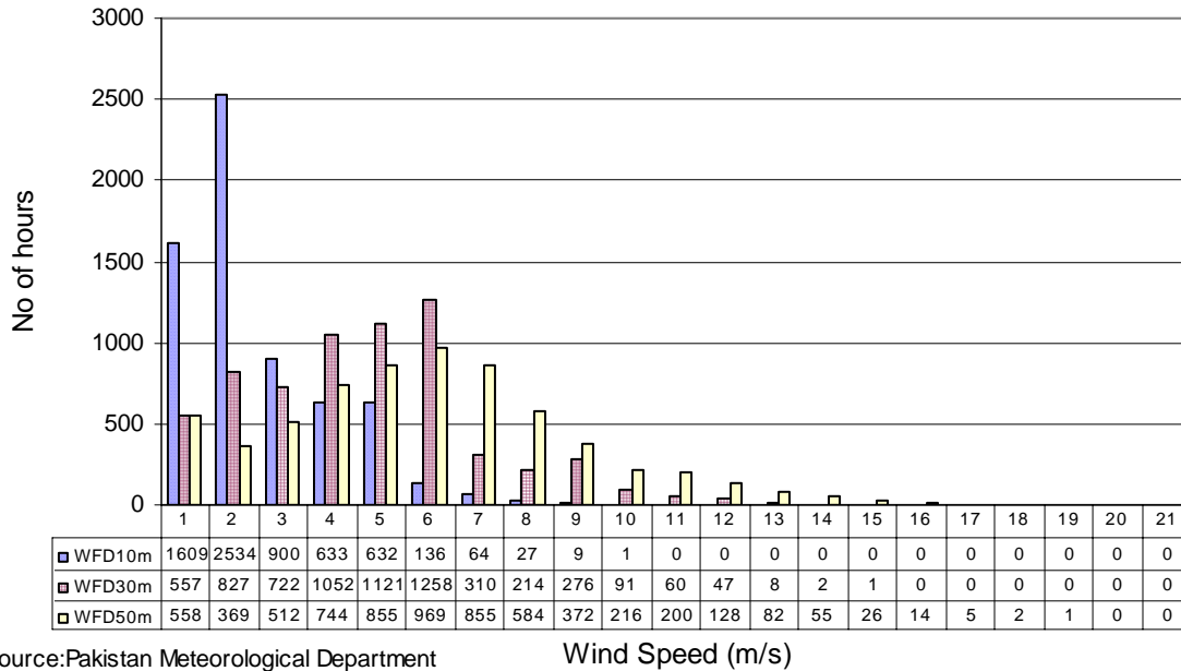
Wind Frequency Distribution at Golarchi (Sep to Nov) in three years
