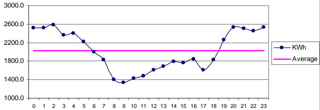
Fig 24 Golarchi Jan: Diurnal Variation of Wind Genrated Electric Energy Output
