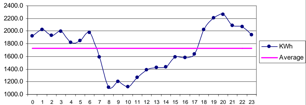
Fig 26 Golarchi Mar: Diurnal Variation of Wind Genrated Electric Energy Output
