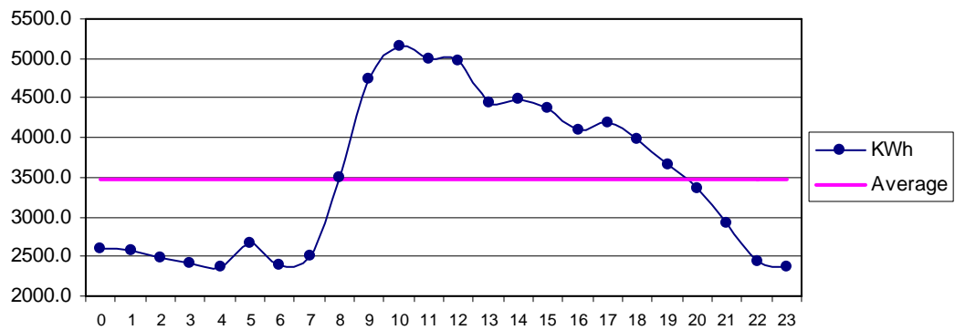
Fig 32 Golarchi Sep: Diurnal Variation of Wind Genrated Electric Energy Output
