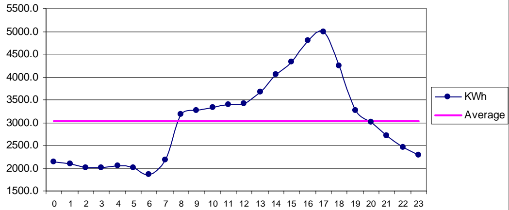
Fig 27 Golarchi Apr: Diurnal Variation of Wind Genrated Electric Energy Output
