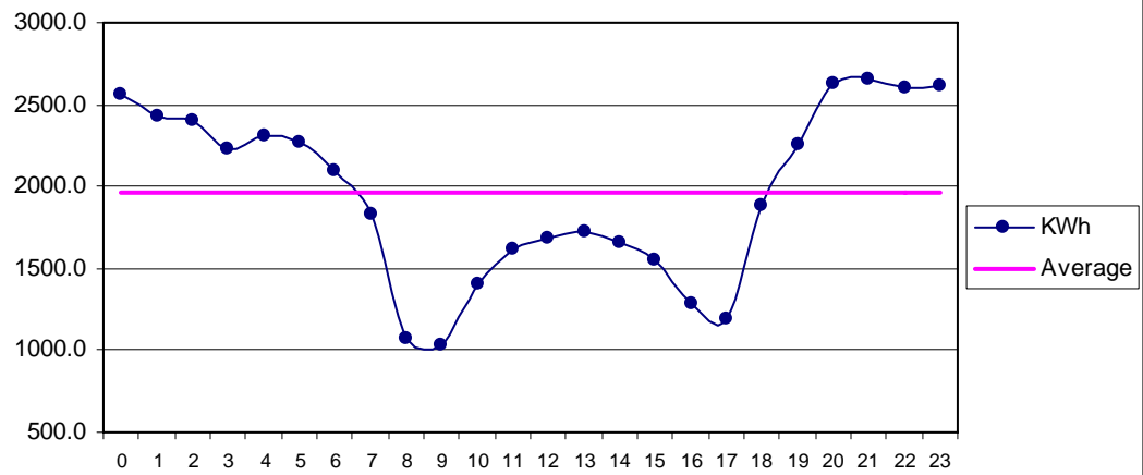
Fig 35 Golarchi Dec: Diurnal Variation of Wind Genrated Electric Energy Output
