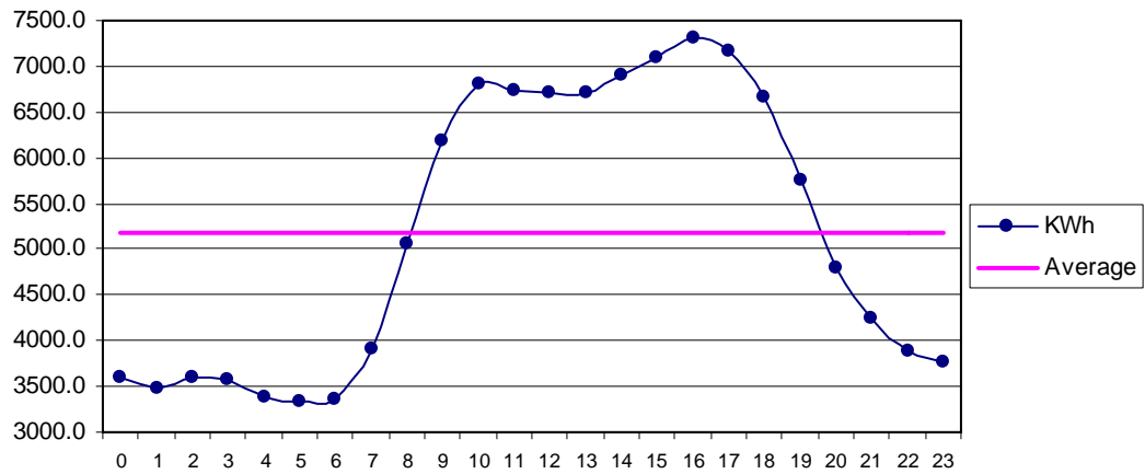
Fig 31 Golarchi Aug: Diurnal Variation of Wind Genrated Electric Energy Output
