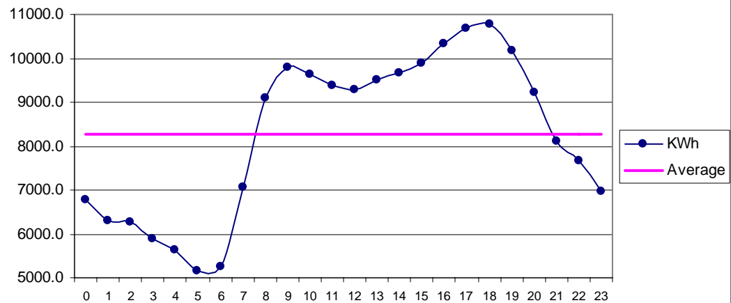
Fig 29 Golarchi Jun: Diurnal Variation of Wind Genrated Electric Energy Output
