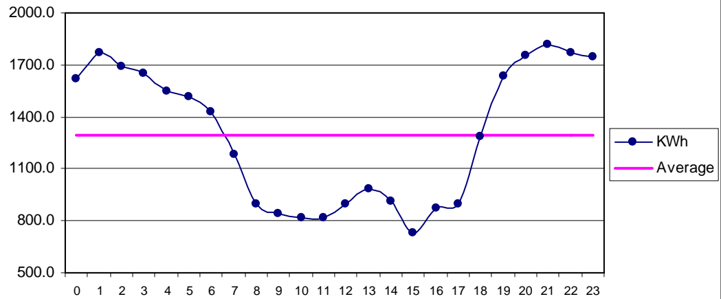
Fig 33 Golarchi Oct: Diurnal Variation of Wind Genrated Electric Energy Output
