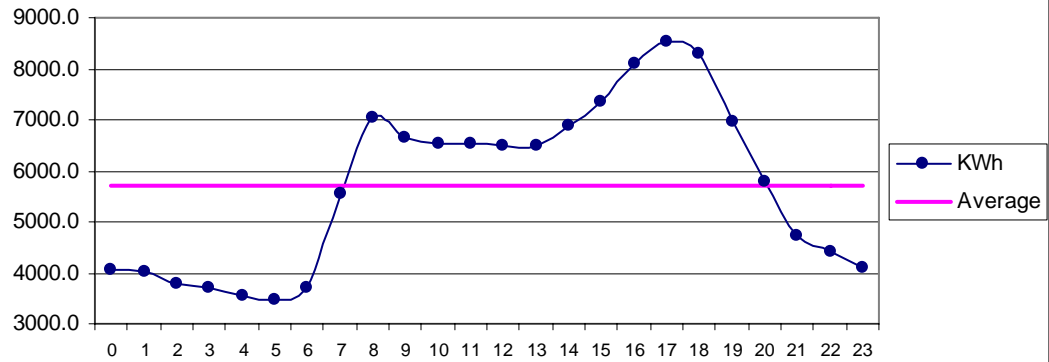
Fig 28 Golarchi May: Diurnal Variation of Wind Genrated Electric Energy Output
