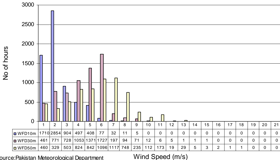
Wind Frequency Distribution at Golarchi (Dec to Feb) in three years
