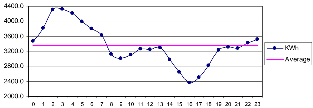
Fig 34 Golarchi Nov: Diurnal Variation of Wind Genrated Electric Energy Output
