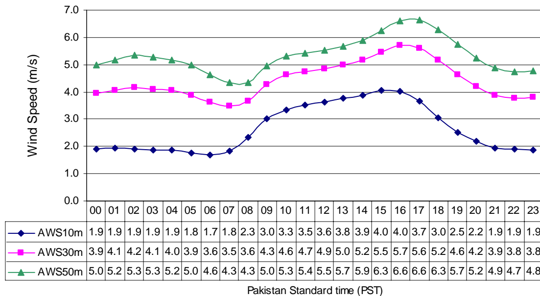
Diurnal Variation of Wind Speed at Gharo (Sep to Nov) in three years
