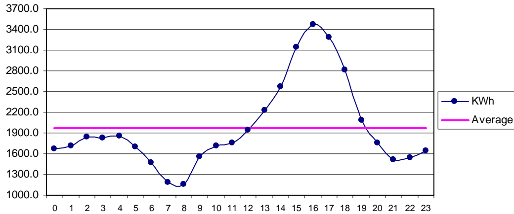
Fig 33 Gharo Oct: Diurnal Variation of Wind Genrated Electric Energy Output
