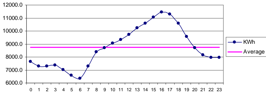
Fig 28 Gharo May: Diurnal Variation of Wind Genrated Electric Energy Output
