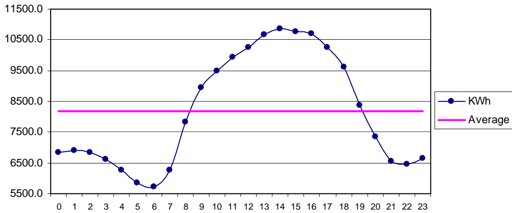
Fig 31 Gharo Aug: Diurnal Variation of Wind Genrated Electric Energy Output
