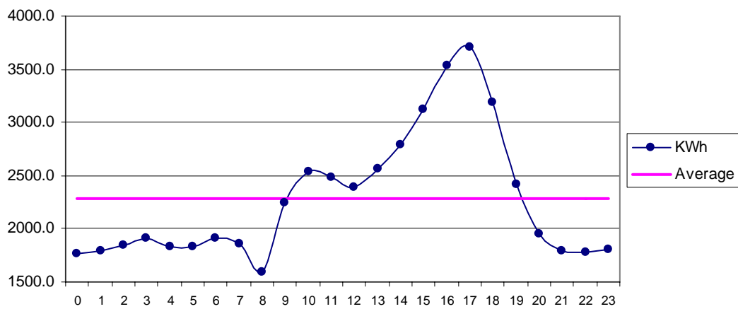
Fig 25 Gharo Feb: Diurnal Variation of Wind Genrated Electric Energy Output
