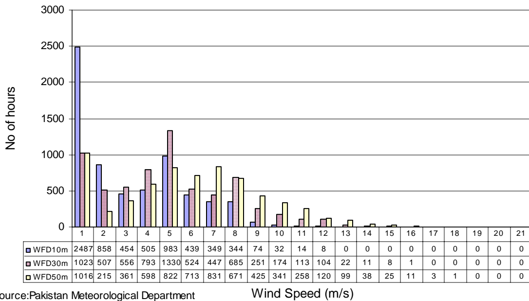
Wind Frequency Distribution at Gharo (Sep to Nov) in three years
