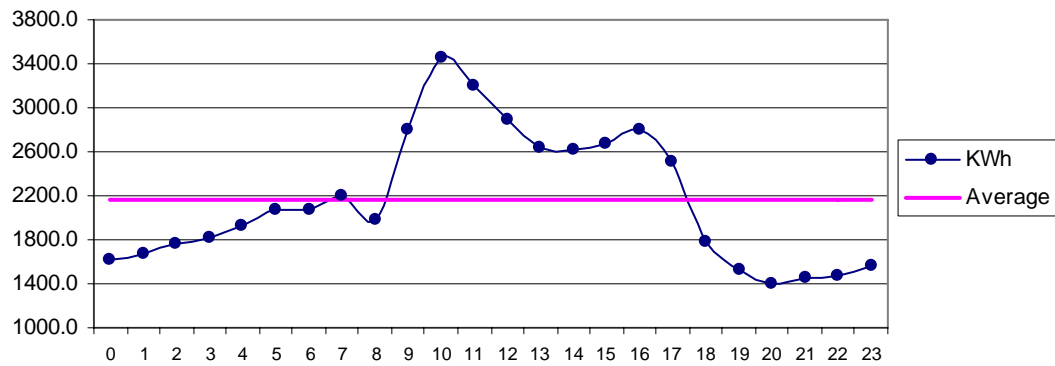
Fig 24 Gharo Jan: Diurnal Variation of Wind Genrated Electric Energy Output
