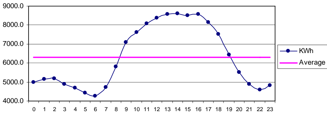
Fig 32 Gharo Sep: Diurnal Variation of Wind Genrated Electric Energy Output
