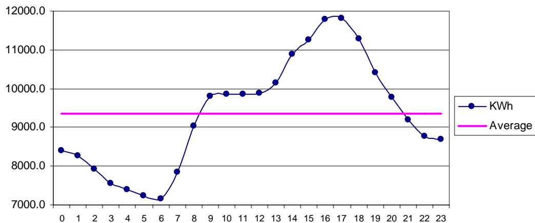
Fig 29 Gharo Jun: Diurnal Variation of Wind Genrated Electric Energy Output
