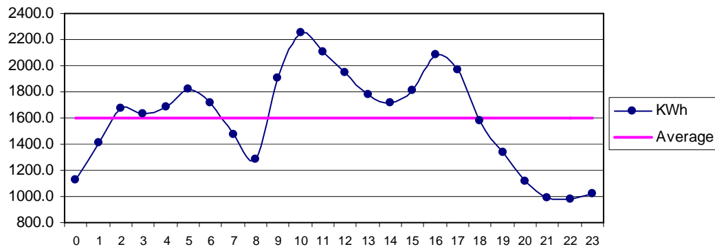
Fig 34 Gharo Nov: Diurnal Variation of Wind Genrated Electric Energy Output
