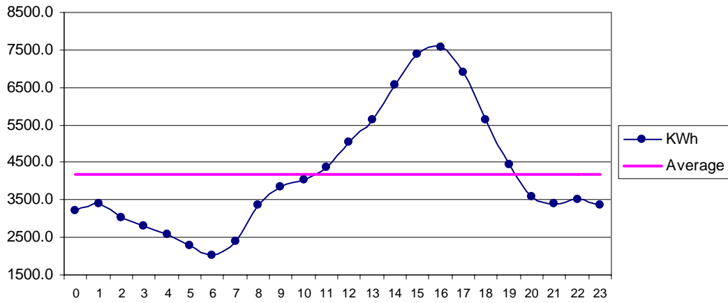
Fig 27 Gharo Apr: Diurnal Variation of Wind Genrated Electric Energy Output
