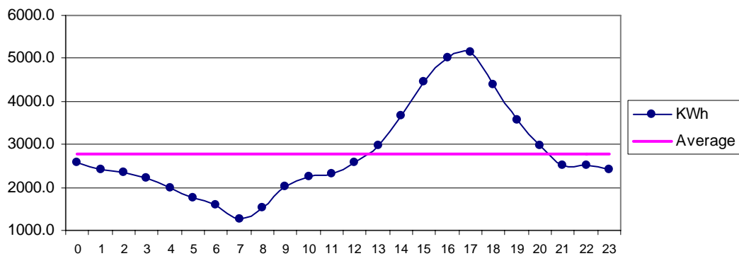
Fig 26 Gharo Mar: Diurnal Variation of Wind Genrated Electric Energy Output
