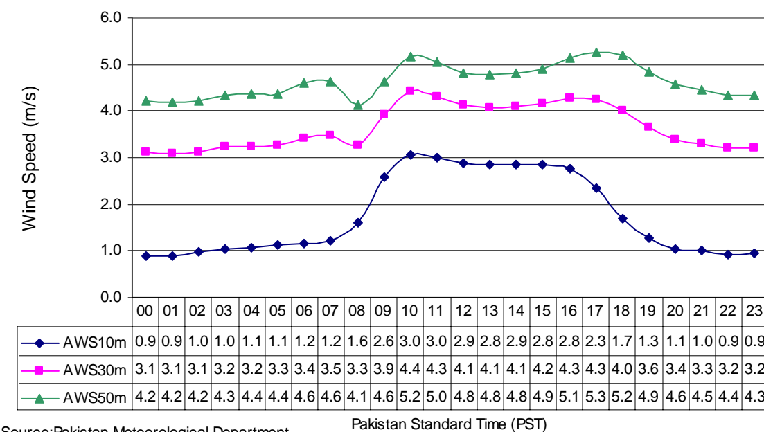
Diurnal Variation of Wind Speed at Gharo (Dec to Feb) in three Years
