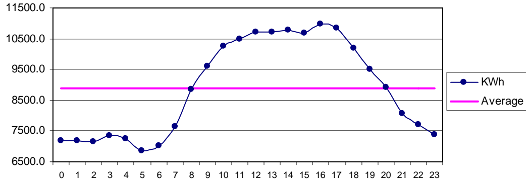
Fig 30 Gharo July: Diurnal Variation of Wind Genrated Electric Energy Output
