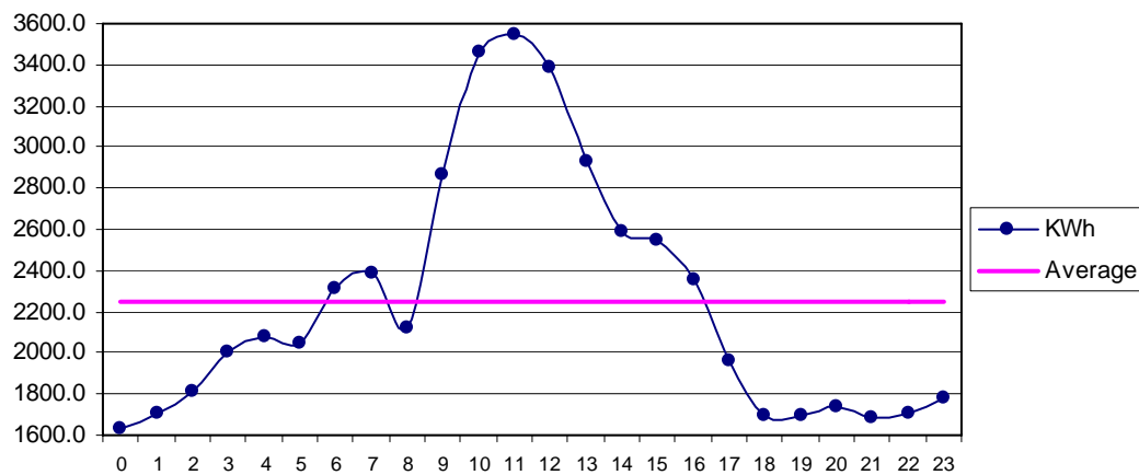
Fig 35 Gharo Dec: Diurnal Variation of Wind Genrated Electric Energy Output
