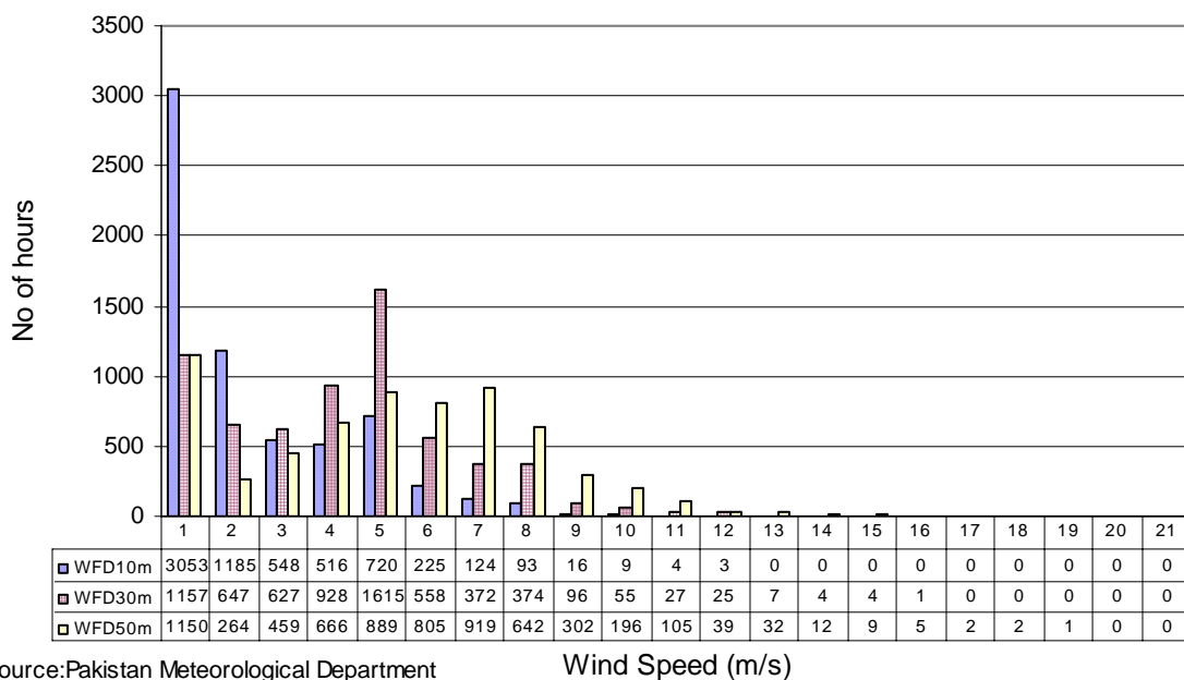
Wind Frequency Distribution at Gharo (Dec to Feb) in three years
