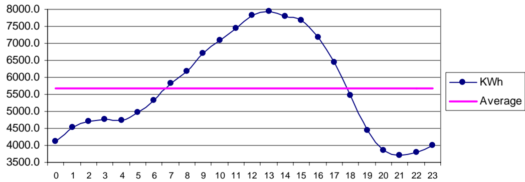
Fig 28 DHA Karachi May: Diurnal Variation of Wind Genrated Electric Energy Output
