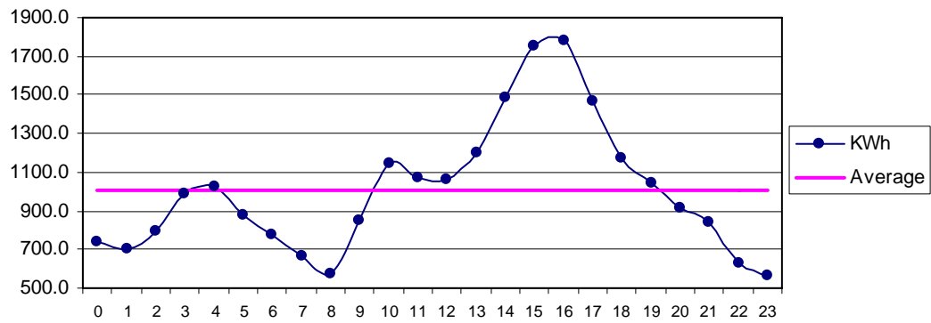
Fig 34 DHA Karachi Nov: Diurnal Variation of Wind Genrated Electric Energy Output
