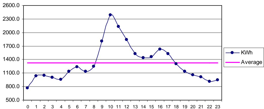
Fig 35 DHA Karachi Dec: Diurnal Variation of Wind Genrated Electric Energy Output
