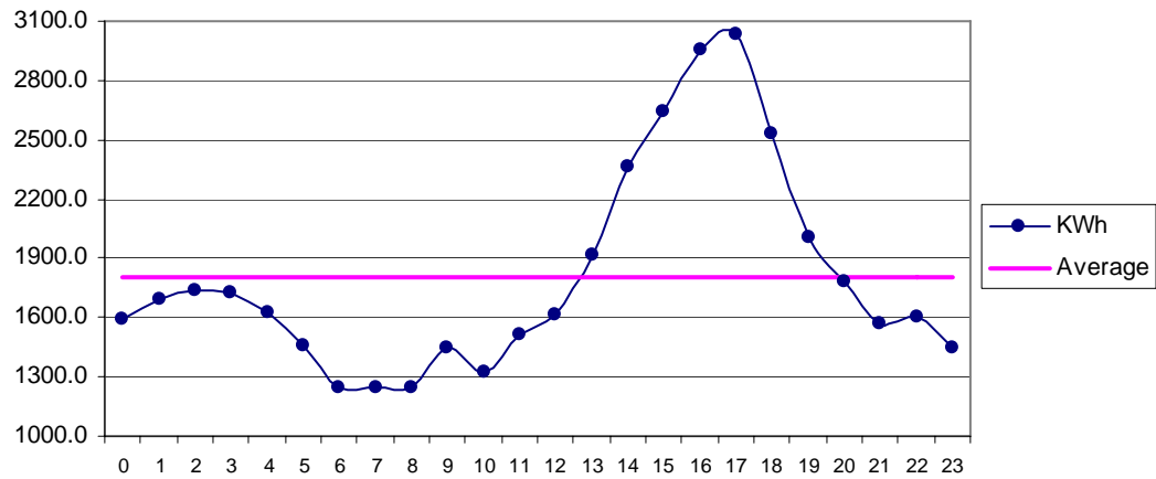
Fig 25 DHA Karachi Feb: Diurnal Variation of Wind Genrated Electric Energy Output
