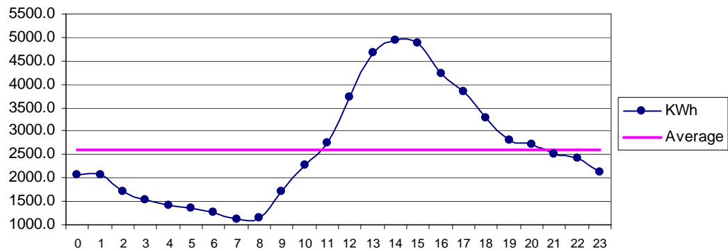
Fig 26 DHA Karachi Mar: Diurnal Variation of Wind Genrated Electric Energy Output
