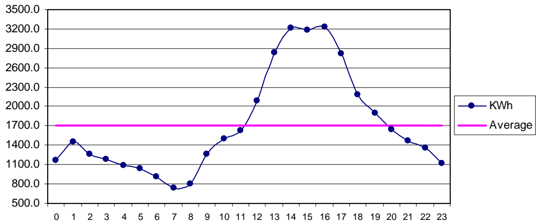
Fig 33 DHA Karachi Oct: Diurnal Variation of Wind Genrated Electric Energy Output
