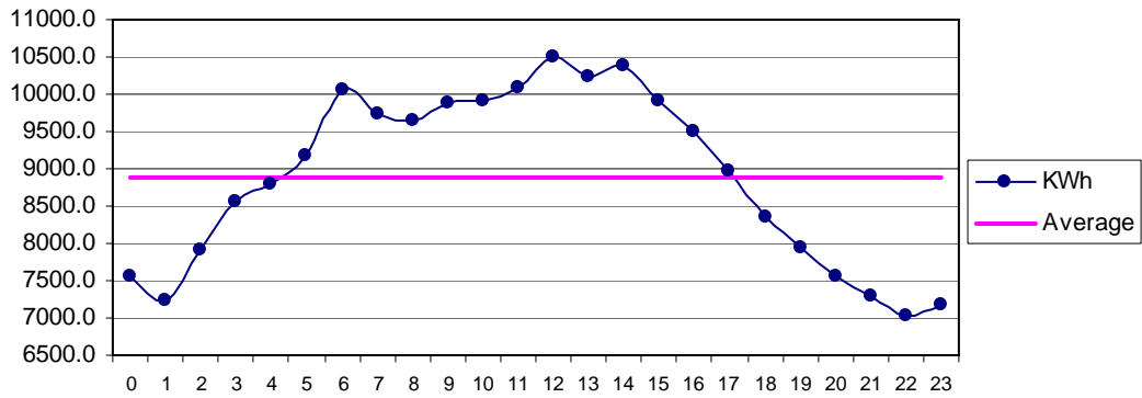
Fig 30 DHA Karachi July: Diurnal Variation of Wind Genrated Electric Energy Output
