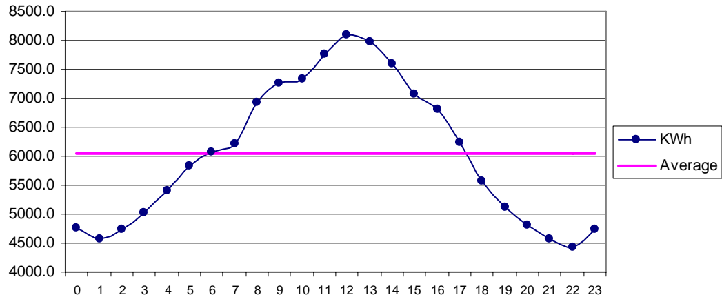
Fig 29 DHA Karachi Jun: Diurnal Variation of Wind Genrated Electric Energy Output
