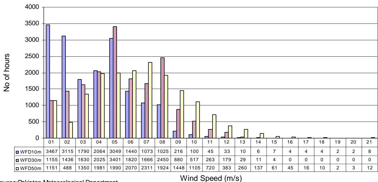
Annual Wind Frequency Distribution at DHA Karachi in two years
