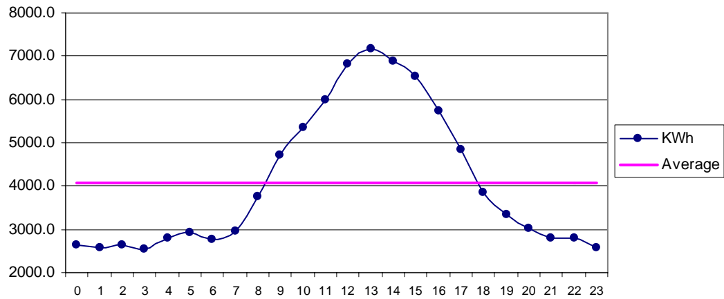
Fig 27 DHA Karachi Apr: Diurnal Variation of Wind Genrated Electric Energy Output
