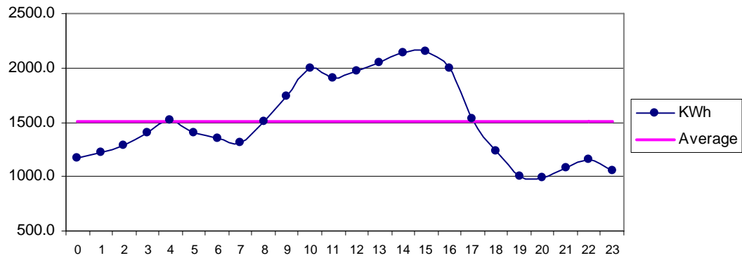
Fig 24 DHA Karachi Jan: Diurnal Variation of Wind Genrated Electric Energy Output
