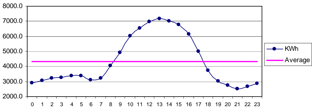
Fig 32 DHA Karachi Sep: Diurnal Variation of Wind Genrated Electric Energy Output
