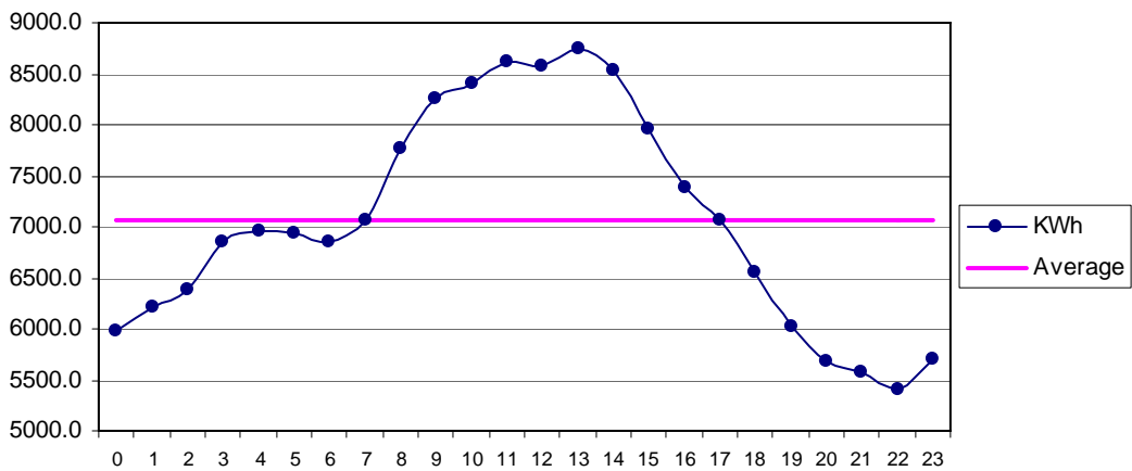
Fig 31 DHA Karachi Aug: Diurnal Variation of Wind Genrated Electric Energy Output
