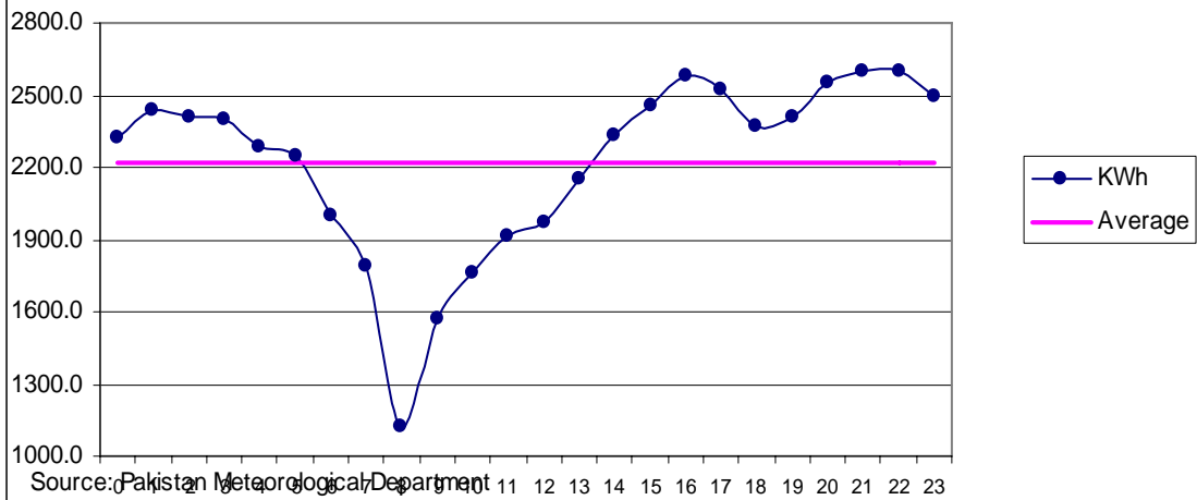
Fig 26 Chuhar Jamali Mar: Diurnal Variation of Wind Genrated Electric Energy Output
