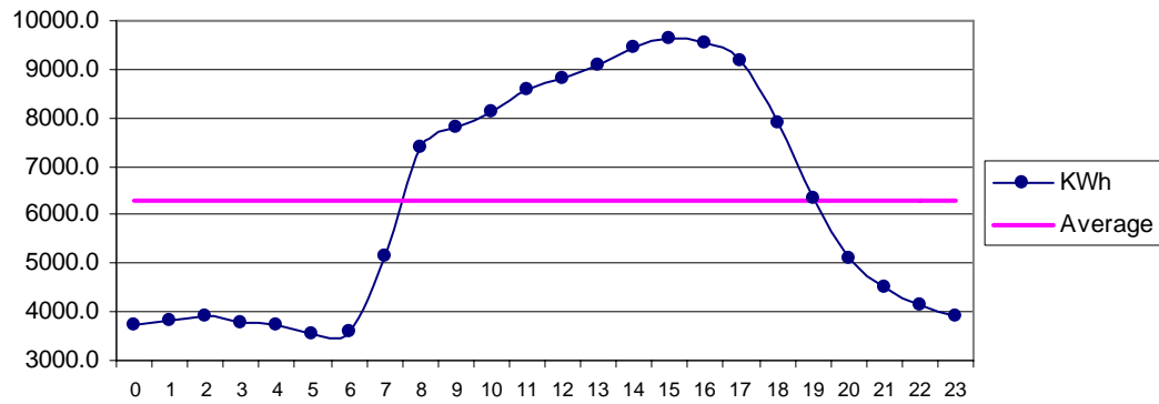
Fig 28 Chuhar Jamali May: Diurnal Variation of Wind Genrated Electric Energy Output
