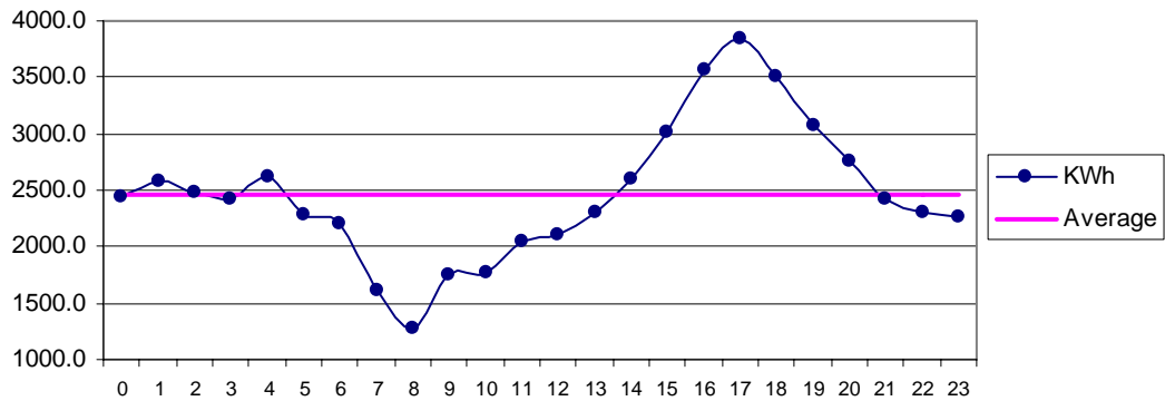
Fig 26 Chuhar Jamali Mar: Diurnal Variation of Wind Genrated Electric Energy Output
