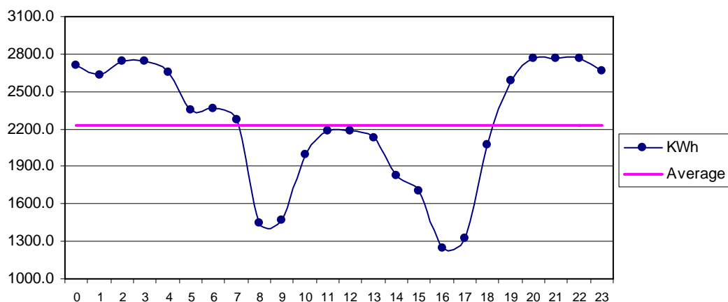
Fig 35 Chuhar Jamali Dec: Diurnal Variation of Wind Genrated Electric Energy Output
