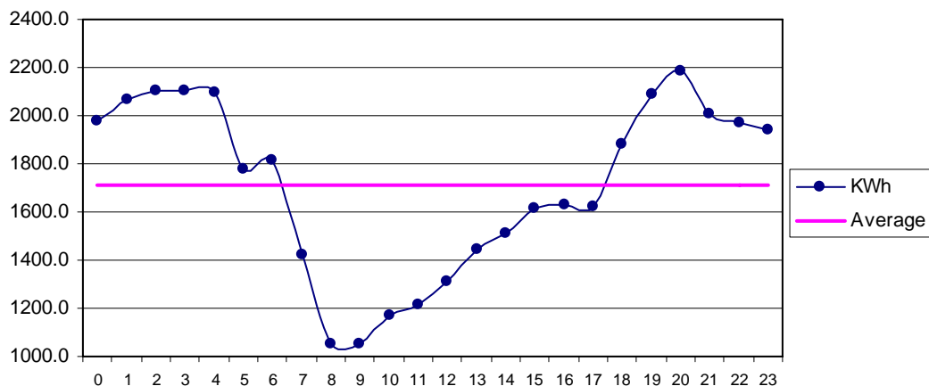
Fig 33 Chuhar Jamali Oct: Diurnal Variation of Wind Genrated Electric Energy Output
