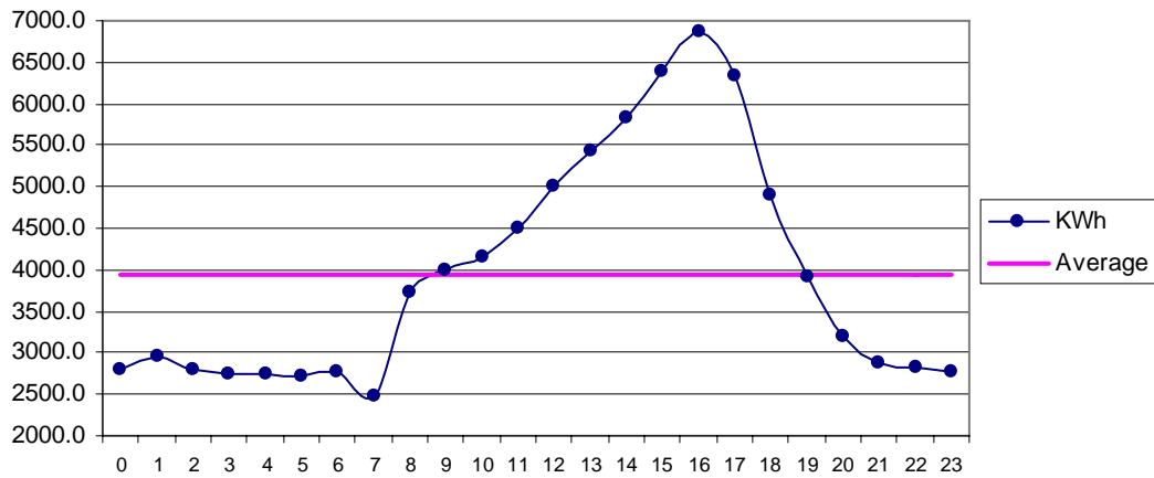
Fig 27 Chuhar Jamali Apr: Diurnal Variation of Wind Genrated Electric Energy Output
