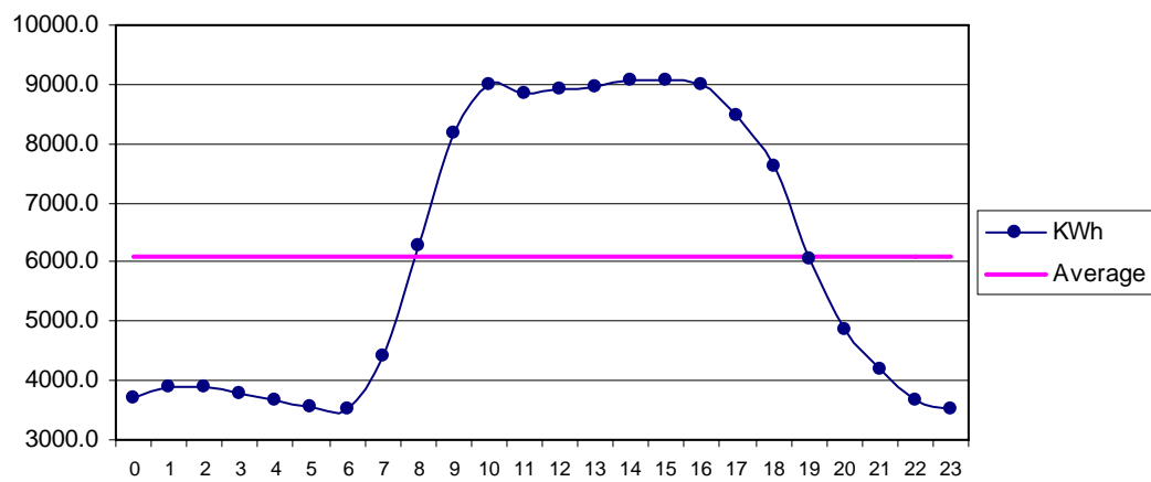
Fig 31 Chuhar Jamali Aug: Diurnal Variation of Wind Genrated Electric Energy Output
