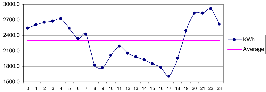
Fig 24 Chuhar Jamali Jan: Diurnal Variation of Wind Genrated Electric Energy Output
