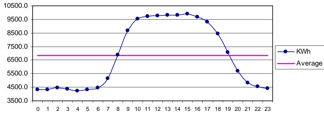
Fig 30 Chuhar Jamali July: Diurnal Variation of Wind Genrated Electric Energy Output
