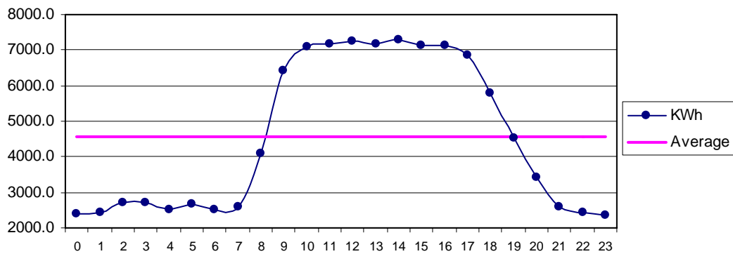
Fig 32 Chuhar Jamali Sep: Diurnal Variation of Wind Genrated Electric Energy Output
