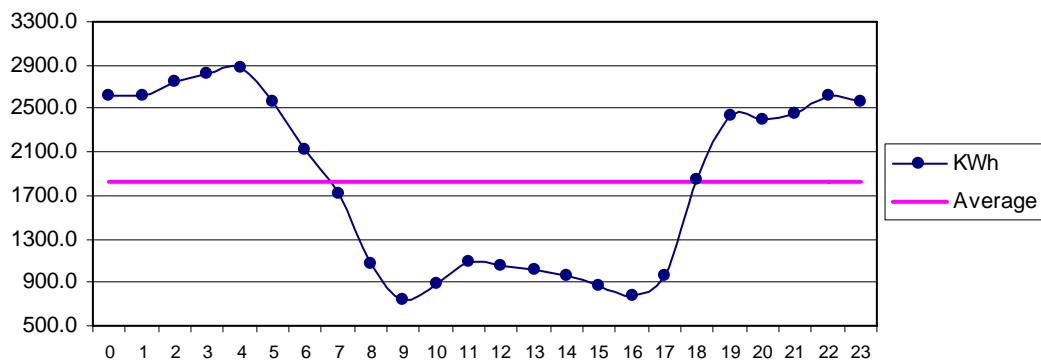
Fig 34 Chuhar Jamali Nov: Diurnal Variation of Wind Genrated Electric Energy Output
