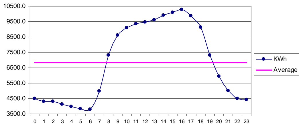
Fig 29 Chuhar Jamali Jun: Diurnal Variation of Wind Genrated Electric Energy Output
