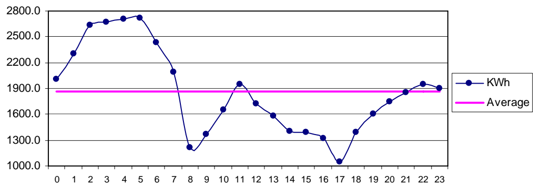
Fig 34 Baghan Nov: Diurnal Variation of Wind Genrated Electric Energy Output
