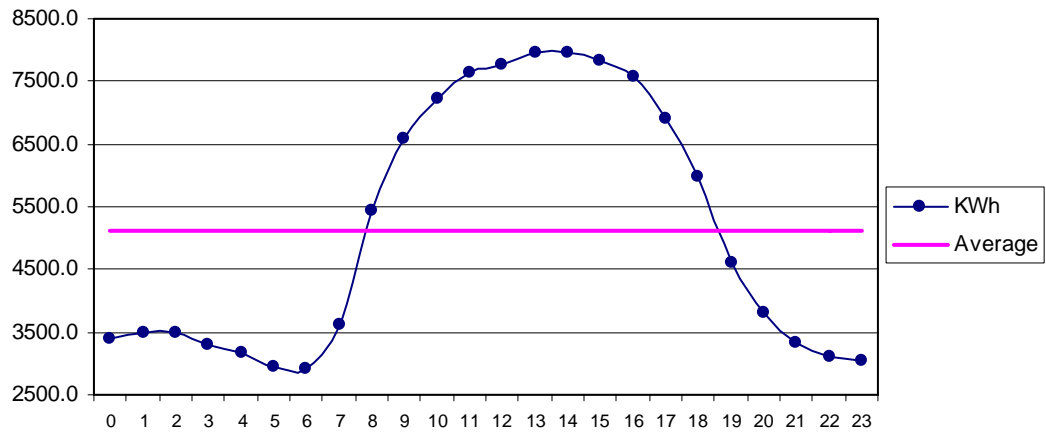
Fig 31 Baghan Aug: Diurnal Variation of Wind Genrated Electric Energy Output
