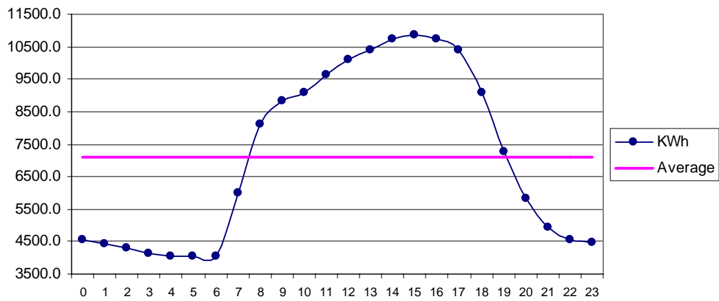
Fig 29 Baghan Jun: Diurnal Variation of Wind Genrated Electric Energy Output
