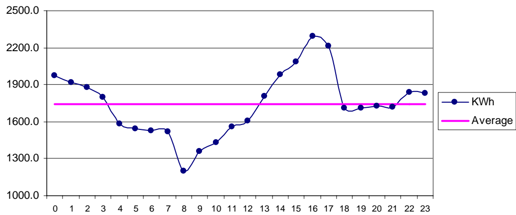
Fig 25 Baghan Feb: Diurnal Variation of Wind Genrated Electric Energy Output
