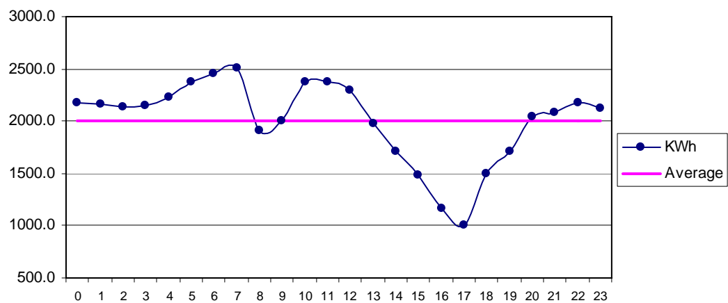
Fig 35 Baghan Dec: Diurnal Variation of Wind Genrated Electric Energy Output
