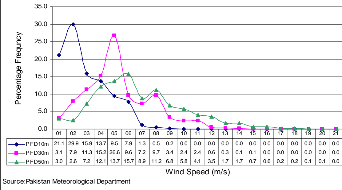
Fig-10 Annual Percentage Wind Frequency Distribution at Baghan in three years
