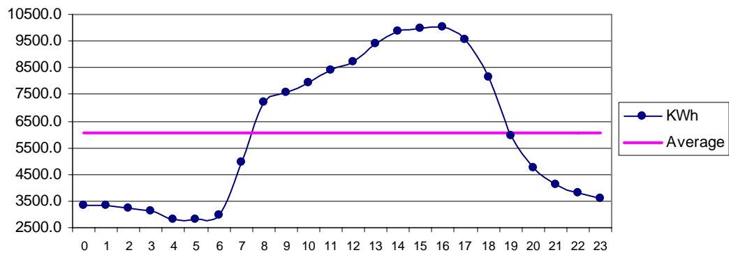
Fig 28 Baghan May: Diurnal Variation of Wind Genrated Electric Energy Output
