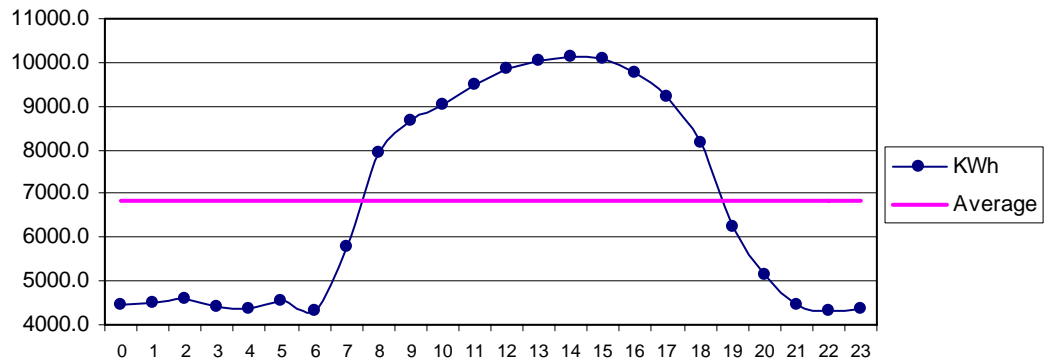
Fig 30 Baghan July: Diurnal Variation of Wind Genrated Electric Energy Output
