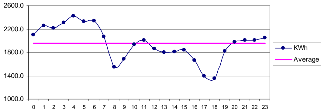
Fig 24 Baghan Jan: Diurnal Variation of Wind Genrated Electric Energy Output
