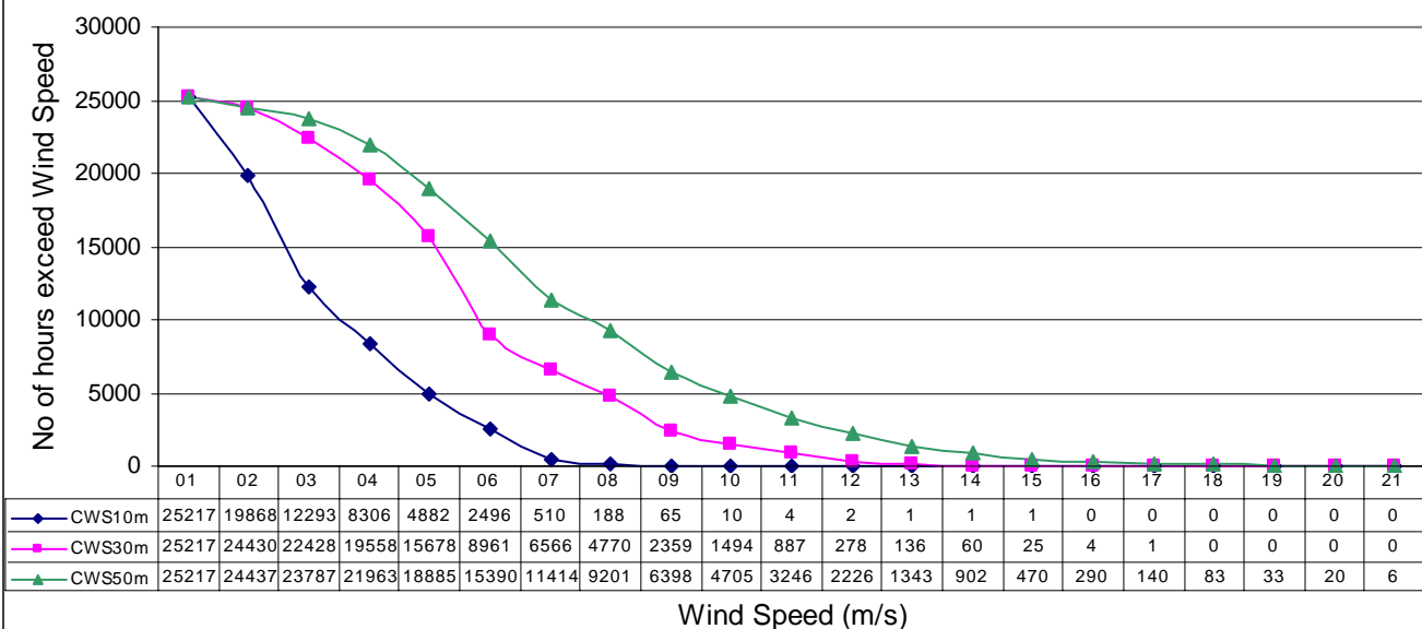
Comulative Wind Speed Distribution at Baghan in three years
