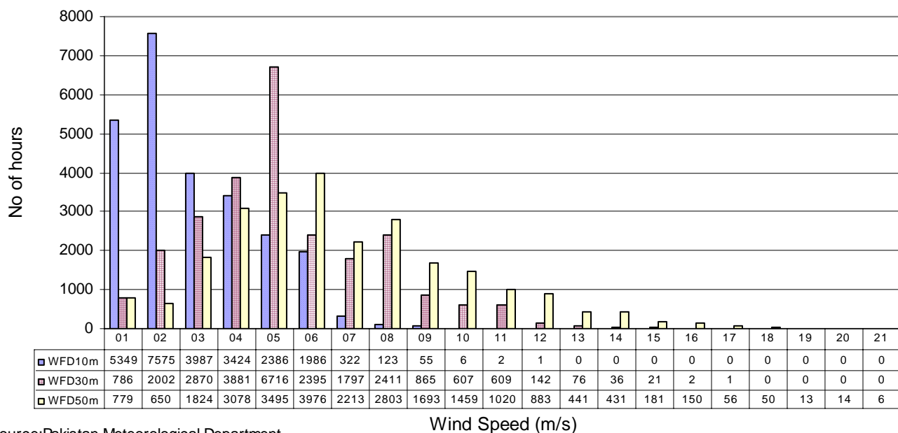
Annual Wind Frequency Distribution at Baghan in three years
