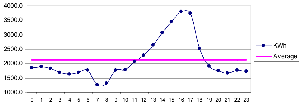
Fig 26 Baghan Mar: Diurnal Variation of Wind Genrated Electric Energy Output
