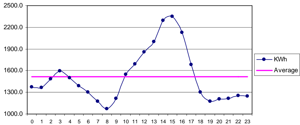
Fig 33 Baghan Oct: Diurnal Variation of Wind Genrated Electric Energy Output
