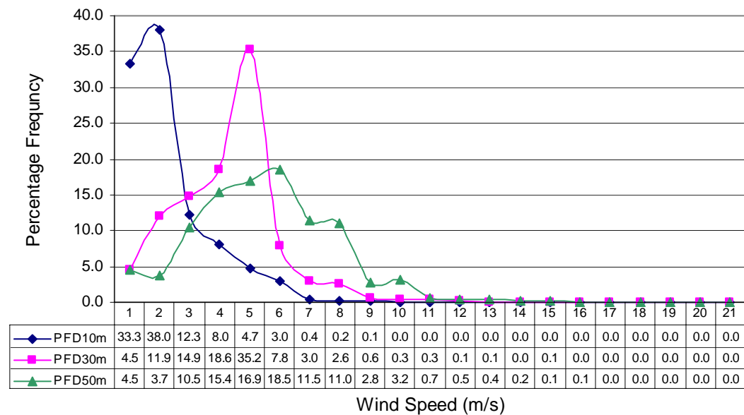
Percentage Wind Frequency Distribution at Baghan (Dec to Feb) in three years
