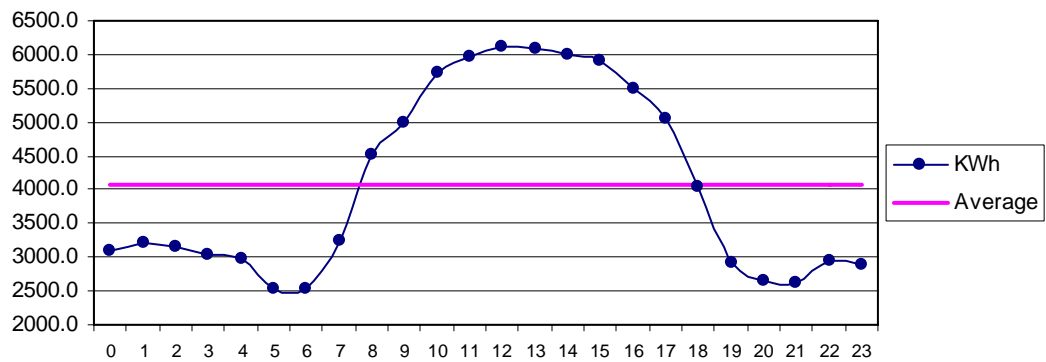
Fig 32 Baghan Sep: Diurnal Variation of Wind Genrated Electric Energy Output
