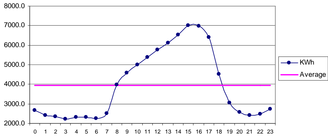
Fig 27 Baghan Apr: Diurnal Variation of Wind Genrated Electric Energy Output
