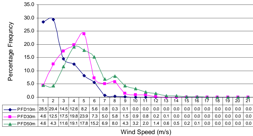
Percentage Wind Frequency Distribution at Baghan (Sep to Nov) in three years
