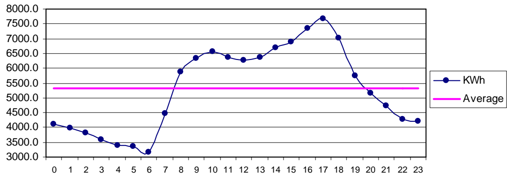
Fig 30 Badin July: Diurnal Variation of Wind Genrated Electric Energy Output
