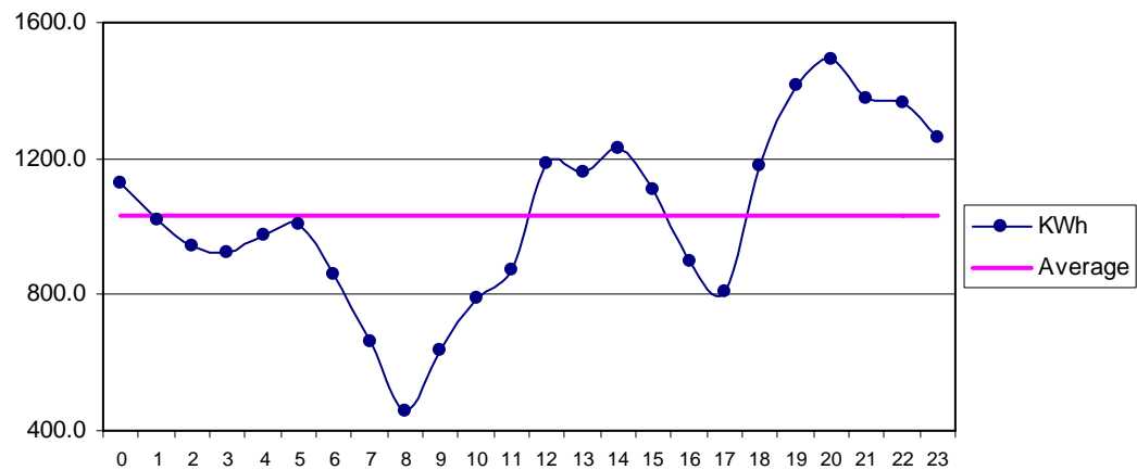
Fig 35 Badin Dec: Diurnal Variation of Wind Genrated Electric Energy Output
