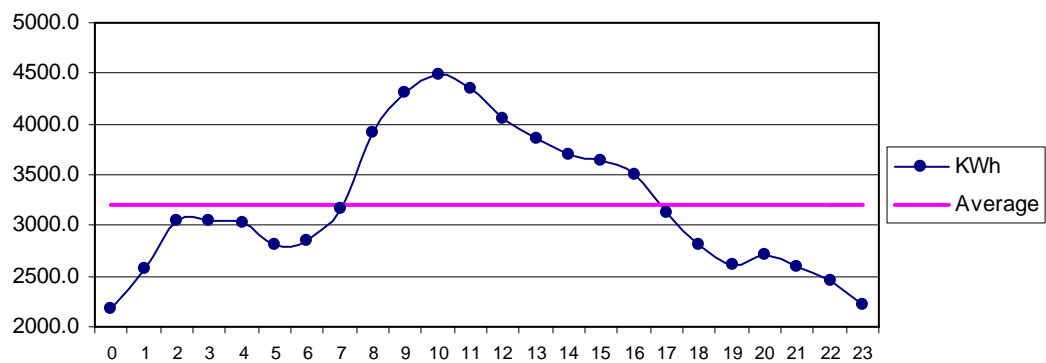
Fig 32 Badin Sep: Diurnal Variation of Wind Genrated Electric Energy Output
