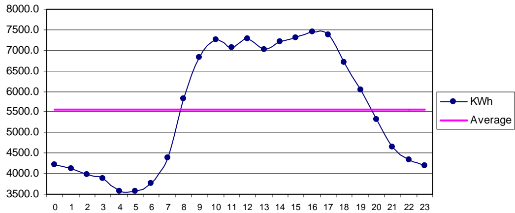
Fig 31 Badin Aug: Diurnal Variation of Wind Genrated Electric Energy Output
