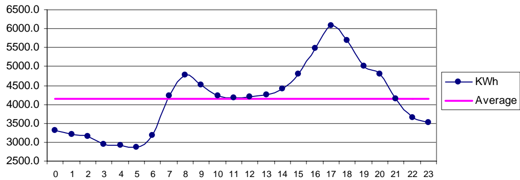
Fig 28 Badin May: Diurnal Variation of Wind Genrated Electric Energy Output
