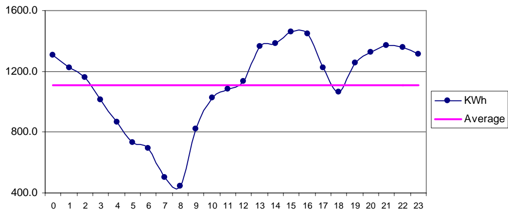
Fig 25 Badin Feb: Diurnal Variation of Wind Genrated Electric Energy Output
