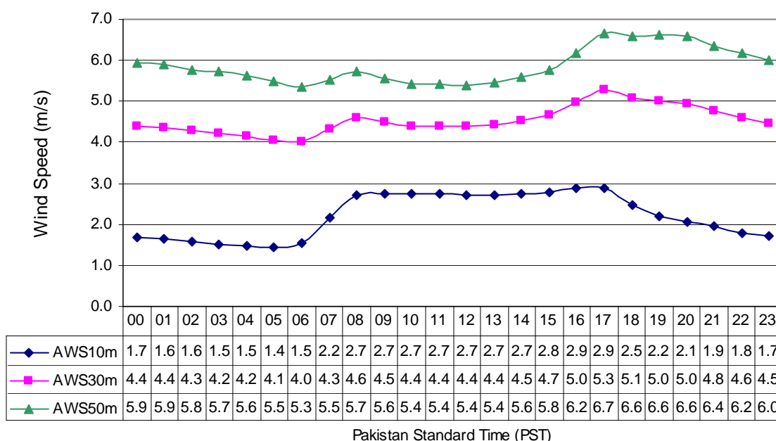
Diurnal Variation of Wind Speed at Badin (Mar to May) in three Years
