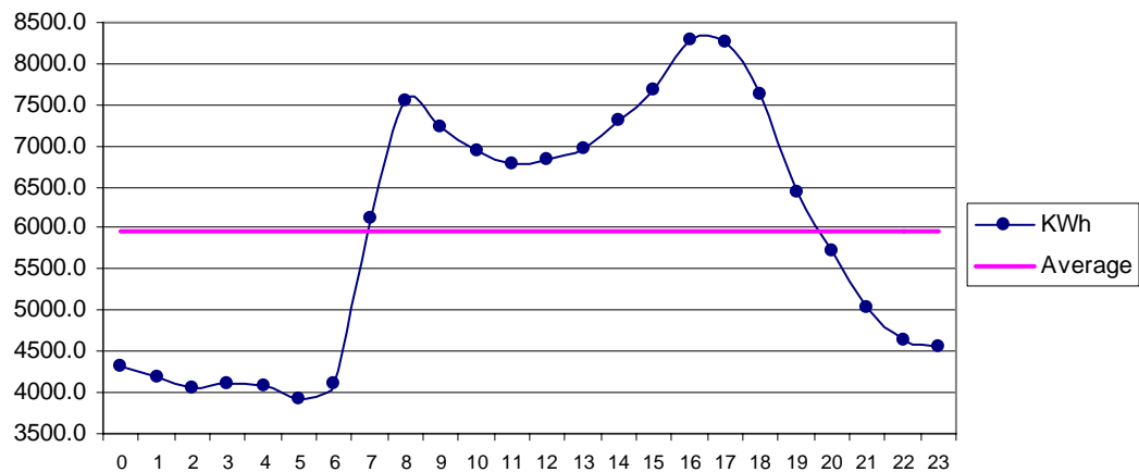
Fig 29 Badin Jun: Diurnal Variation of Wind Genrated Electric Energy Output
