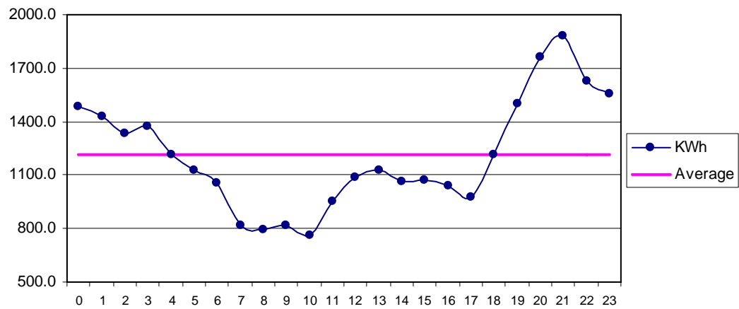
Fig 33 Badin Oct: Diurnal Variation of Wind Genrated Electric Energy Output
