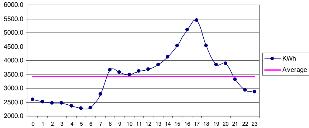
Fig 27 Badin Apr: Diurnal Variation of Wind Genrated Electric Energy Output
