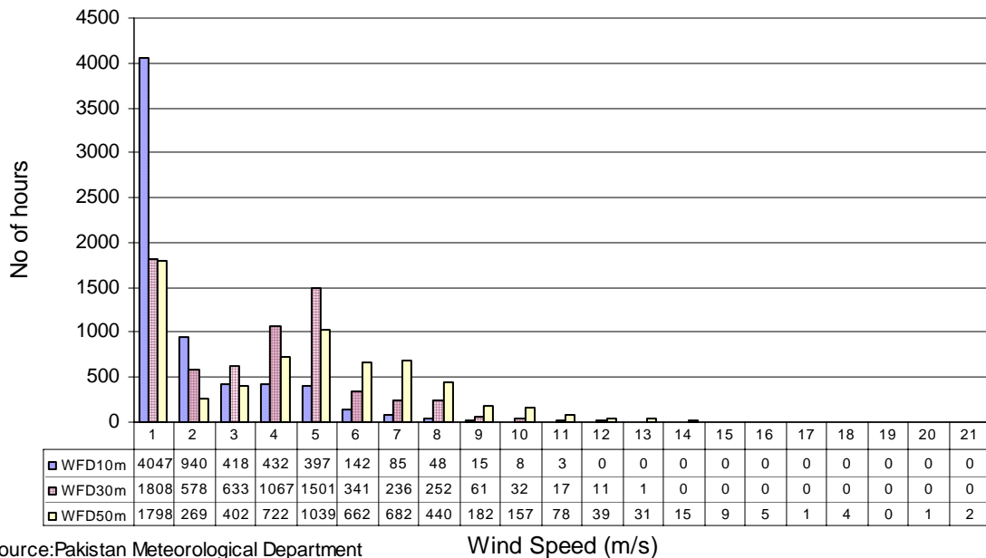
Wind Frequency Distribution at Badin (Sep to Nov) in three years
