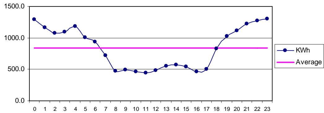
Fig 34 Badin Nov: Diurnal Variation of Wind Genrated Electric Energy Output
