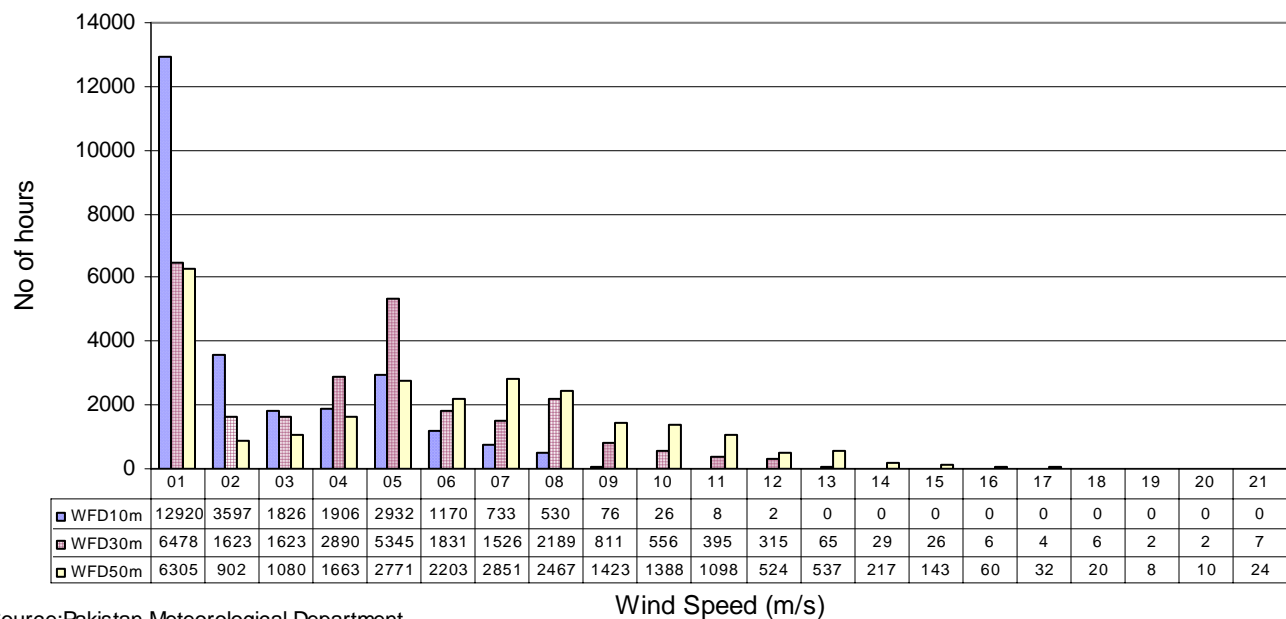
Annual Wind Frequency Distribution at Badin in three years
