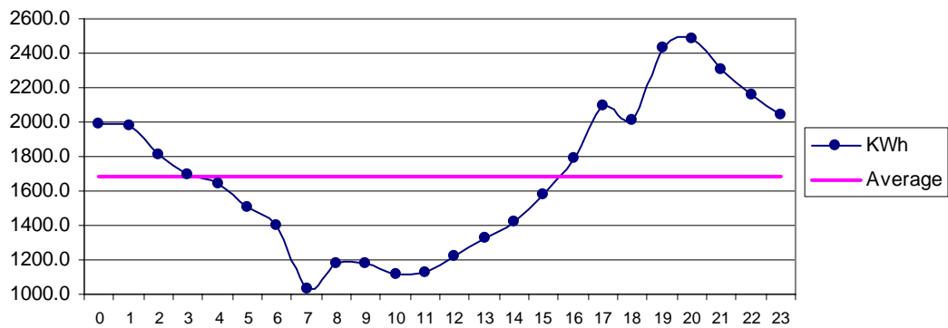
Fig 26 Badin Mar: Diurnal Variation of Wind Genrated Electric Energy Output
