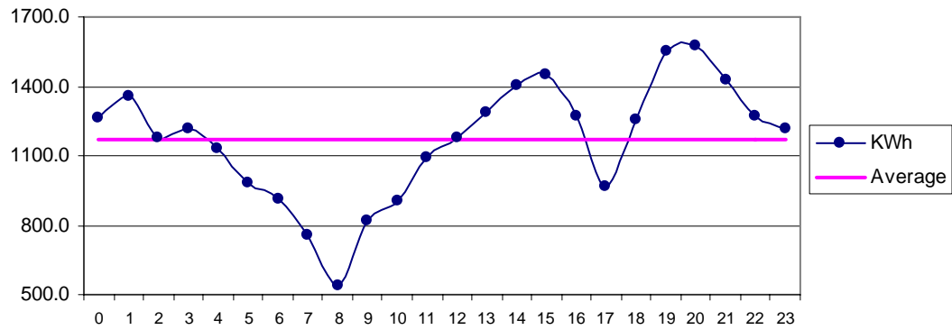
Fig 24 Badin Jan: Diurnal Variation of Wind Genrated Electric Energy Output
