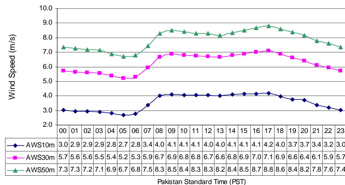
Diurnal Variation of Wind Speed at Badin (Jun to Aug) in three Years
