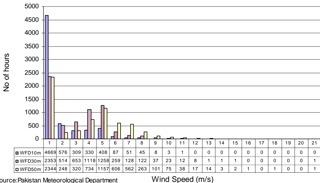
Wind Frequency Distribution at Winder (Dec to Feb) in three years
