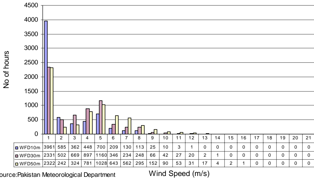
Wind Frequency Distribution at Winder (Sep to Nov) in three years
