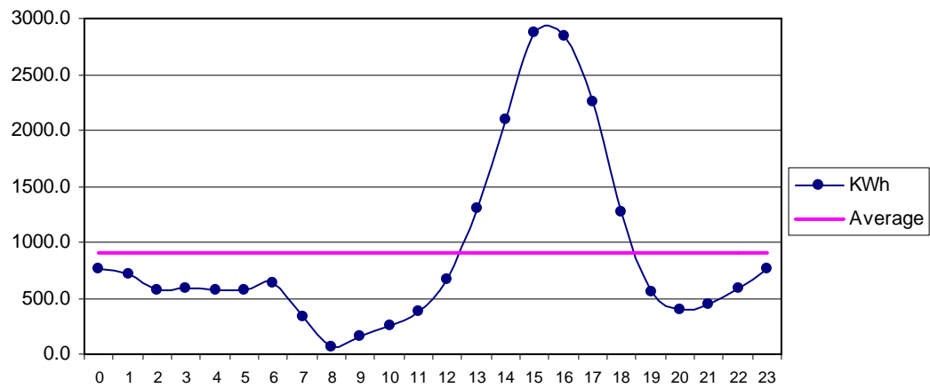
Fig 33 Winder Oct: Diurnal Variation of Wind Genrated Electric Energy Output
