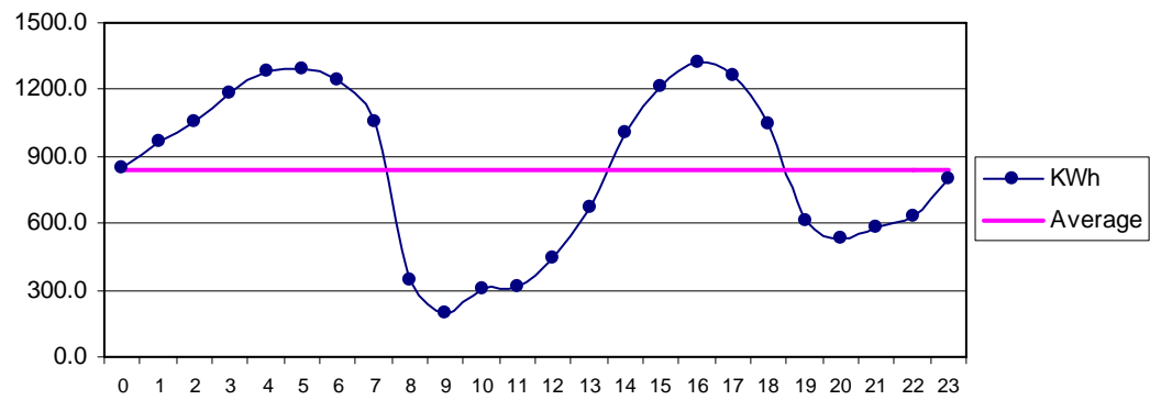
Fig 34 Winder Nov: Diurnal Variation of Wind Genrated Electric Energy Output
