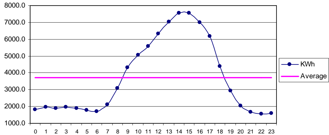
Fig 31 Winder Aug: Diurnal Variation of Wind Genrated Electric Energy Output
