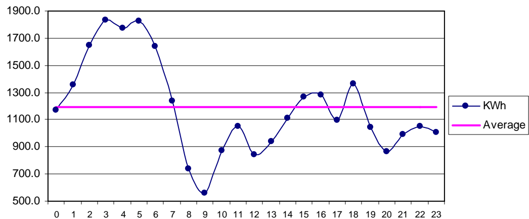
Fig 35 Winder Dec: Diurnal Variation of Wind Genrated Electric Energy Output
