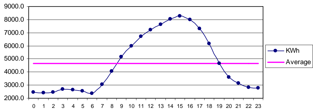
Fig 30 Winder July: Diurnal Variation of Wind Genrated Electric Energy Output
