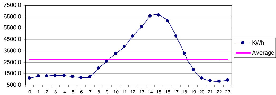
Fig 32 Winder Sep: Diurnal Variation of Wind Genrated Electric Energy Output
