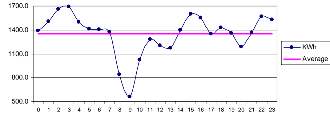
Fig 24 Winder Jan: Diurnal Variation of Wind Genrated Electric Energy Output
