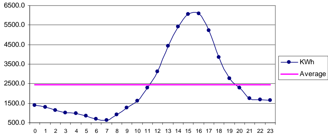
Fig 27 Winder Apr: Diurnal Variation of Wind Genrated Electric Energy Output
