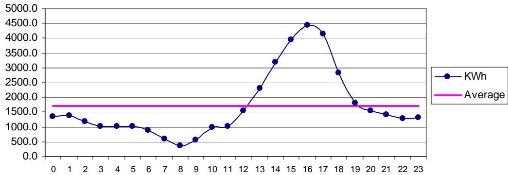
Fig 26 WinderMar: Diurnal Variation of Wind Genrated Electric Energy Output
