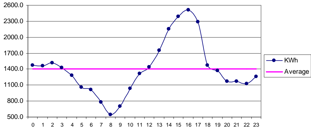
Fig 25 Winder Feb: Diurnal Variation of Wind Genrated Electric Energy Output
