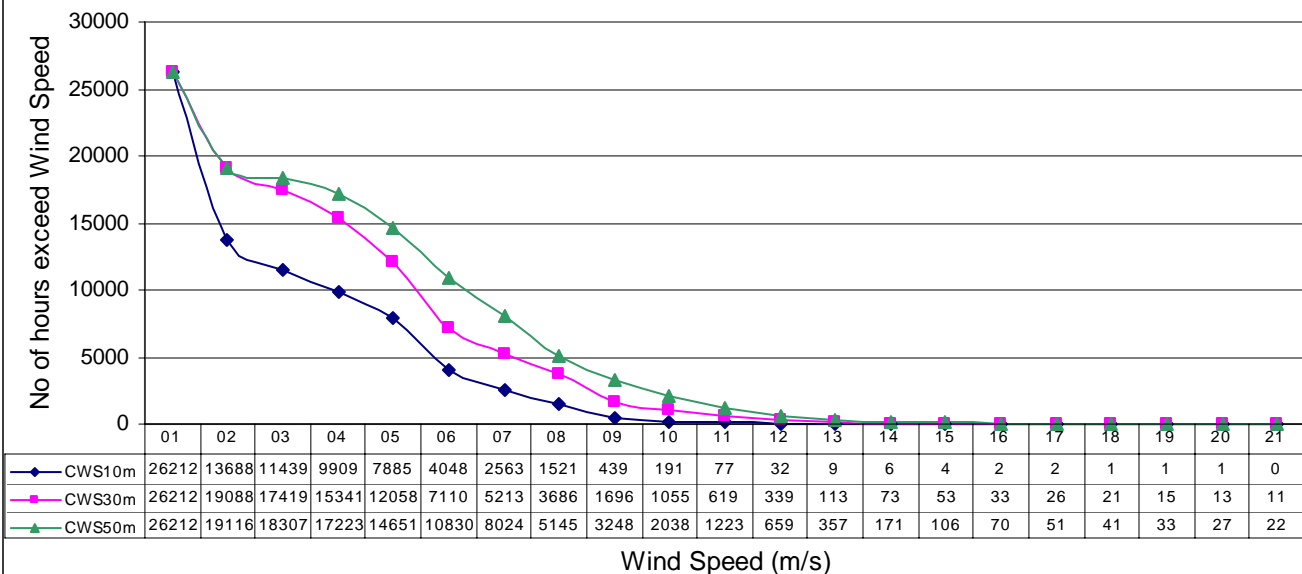
Comulative Wind Speed Distribution at Winder in three years
