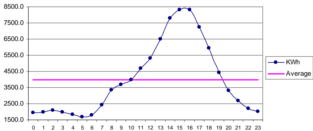
Fig 29 Winder Jun: Diurnal Variation of Wind Genrated Electric Energy Output
