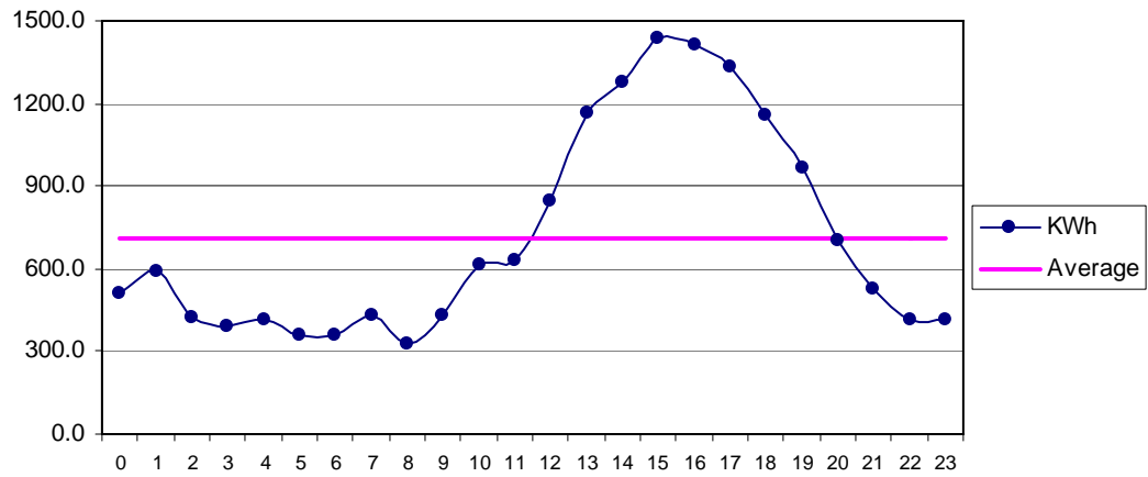
Fig 35 Ramra Dec: Diurnal Variation of Wind Genrated Electric Energy Output
