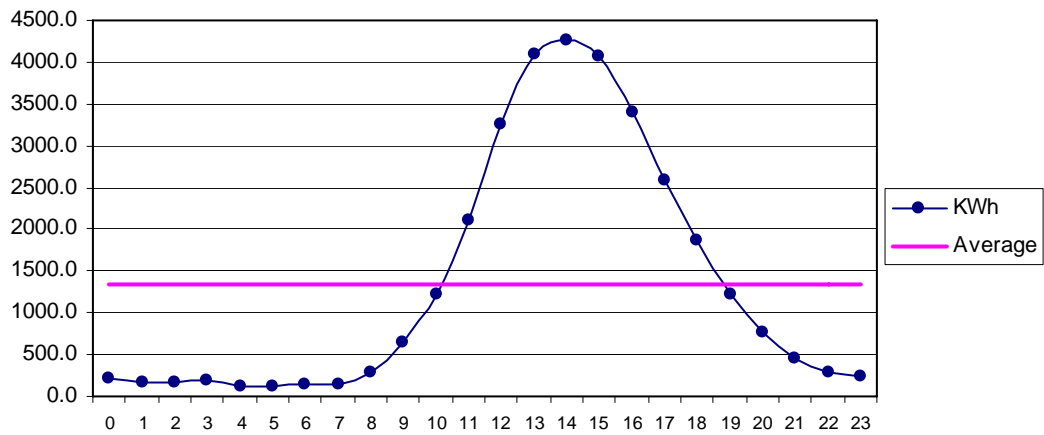
Fig 31 Ramra Aug: Diurnal Variation of Wind Genrated Electric Energy Output
