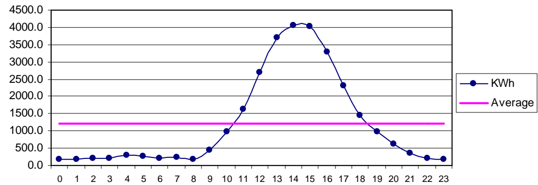
Fig 32 Ramra Sep: Diurnal Variation of Wind Genrated Electric Energy Output
