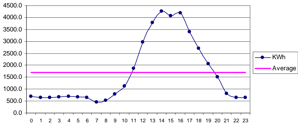
Fig 27 Ramra Apr: Diurnal Variation of Wind Genrated Electric Energy Output
