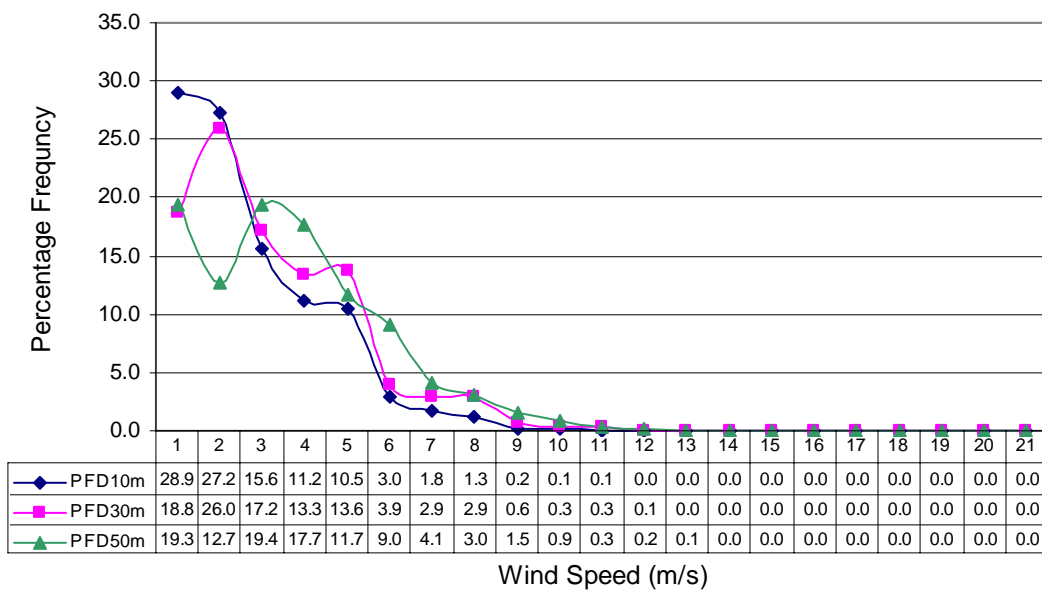
Percentage Wind Frequency Distribution at Ramra (Dec to Feb) in three years
