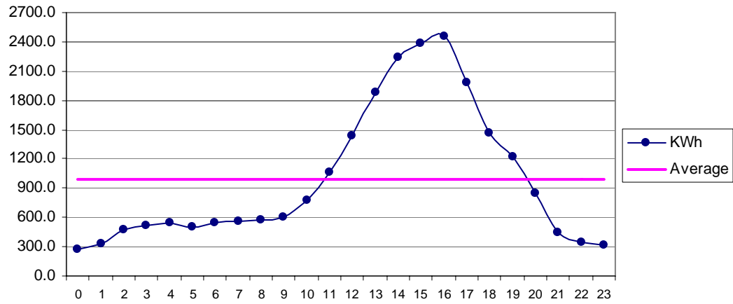
Fig 25 Ramra Feb: Diurnal Variation of Wind Genrated Electric Energy Output
