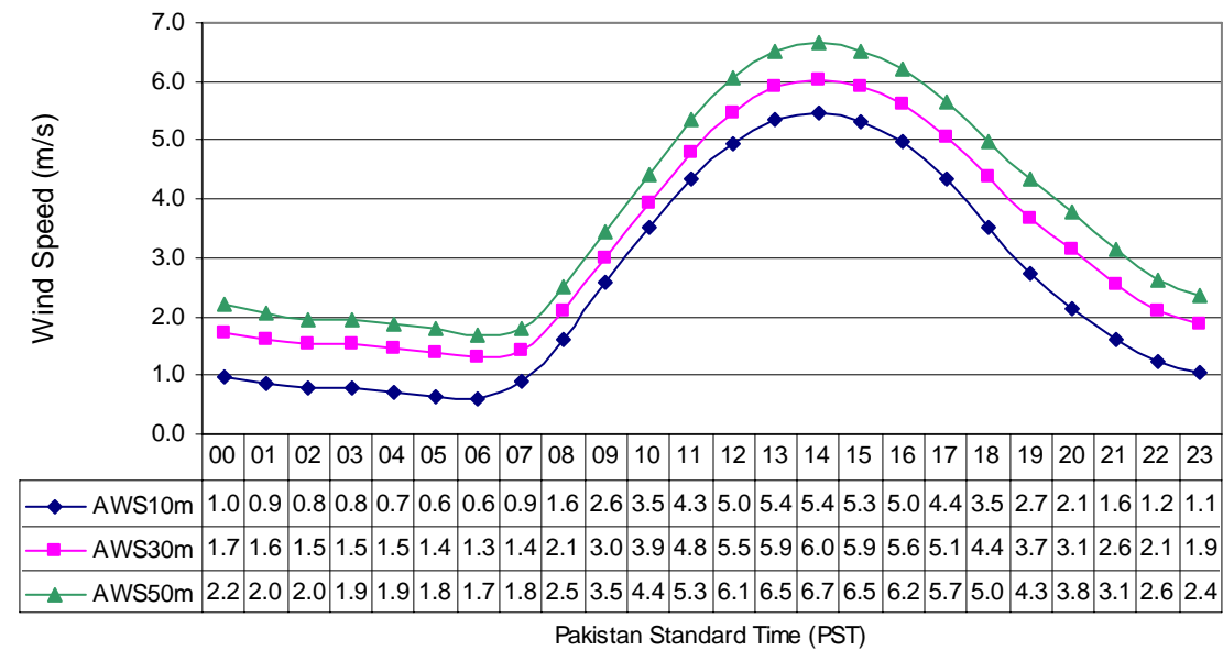
Fig-5 Diurnal Variation of Wind Speed at Ramra (Jun to Aug) in three Years
