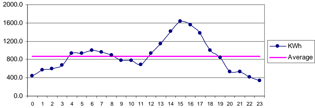
Fig 24 Ramra Jan: Diurnal Variation of Wind Genrated Electric Energy Output
