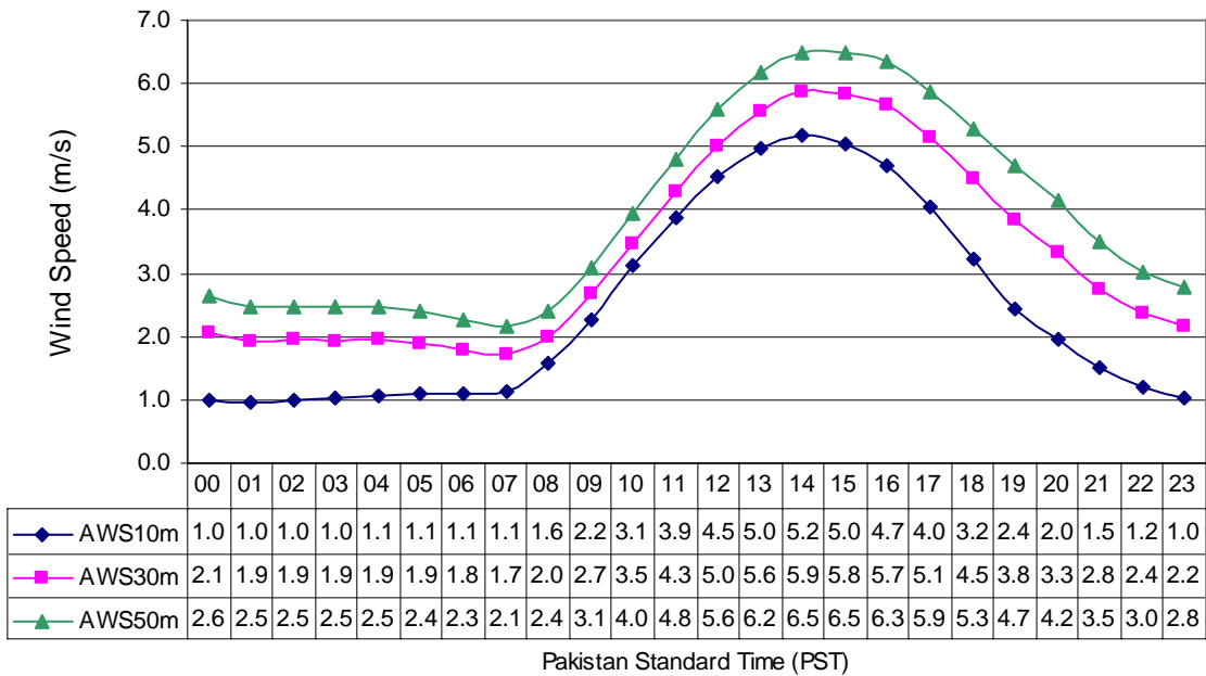
Fig-4 Diurnal Variation of Wind Speed at Ramra (Mar to May) in three Years
