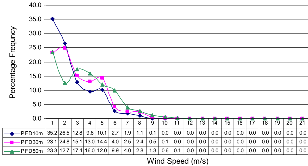
Percentage Wind Frequency Distribution at Ramra (Sep to Nov) in three years
