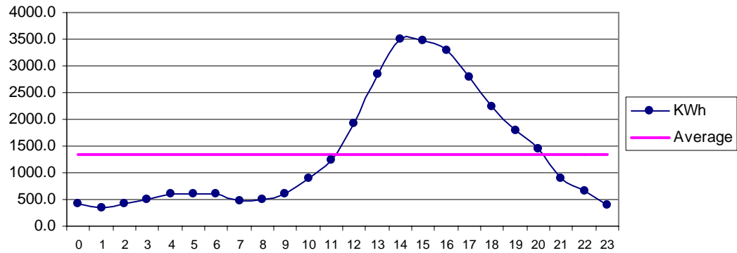
Fig 26 Ramra Mar: Diurnal Variation of Wind Genrated Electric Energy Output
