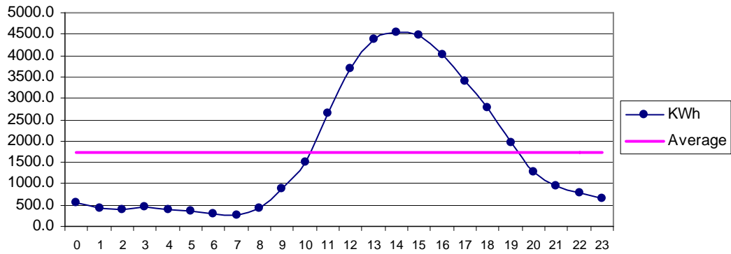
Fig 28 Ramra May: Diurnal Variation of Wind Genrated Electric Energy Output
