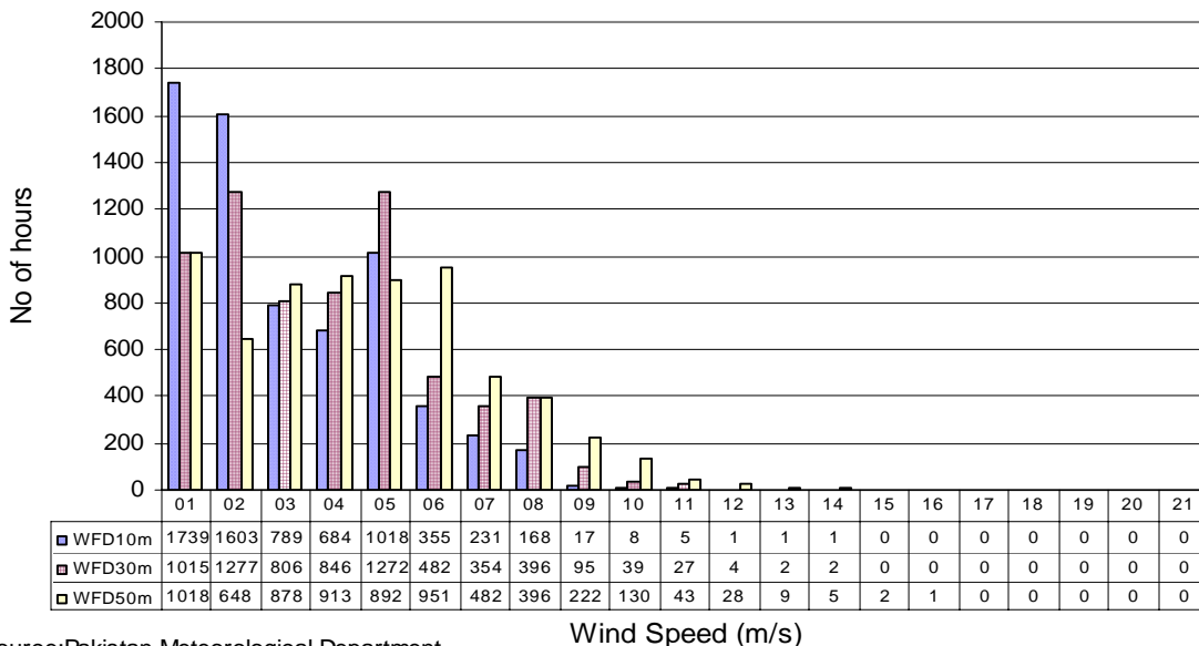
Wind Frequency Distribution at Ramra (Mar to May) in three years
