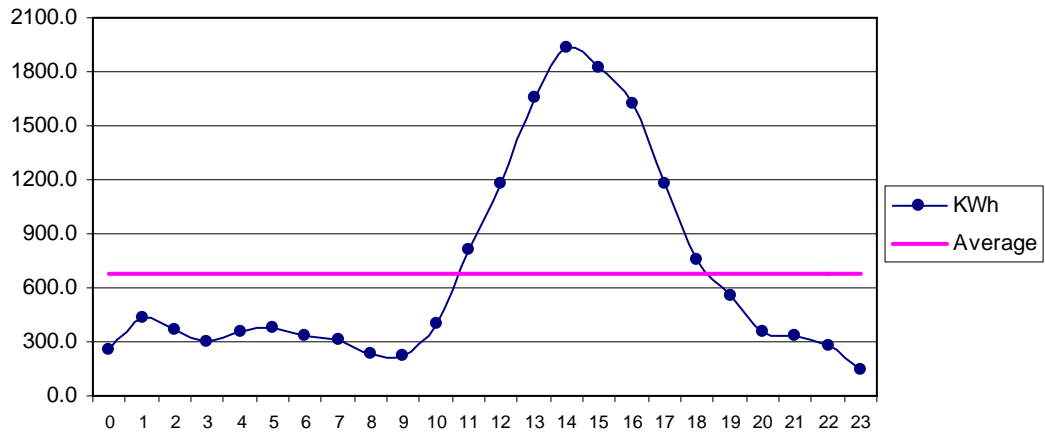
Fig 34 Ramra Nov: Diurnal Variation of Wind Genrated Electric Energy Output
