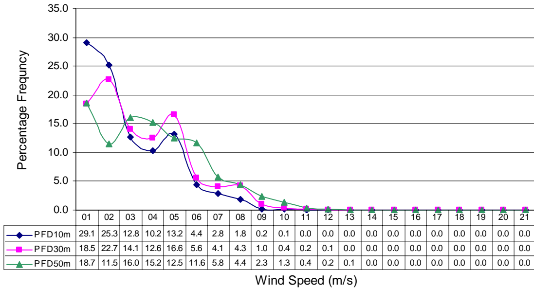
Annual Percentage Wind Frequency Distribution at Ramra in three years
