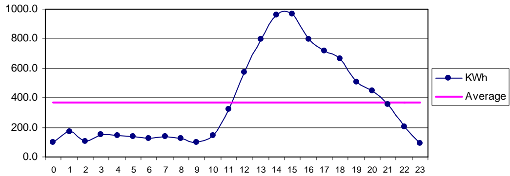
Fig 34 Ramra Nov: Diurnal Variation of Wind Genrated Electric Energy Output
