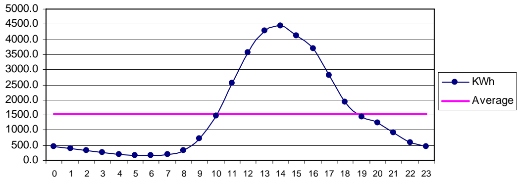
Fig 30 Ramra July: Diurnal Variation of Wind Genrated Electric Energy Output
