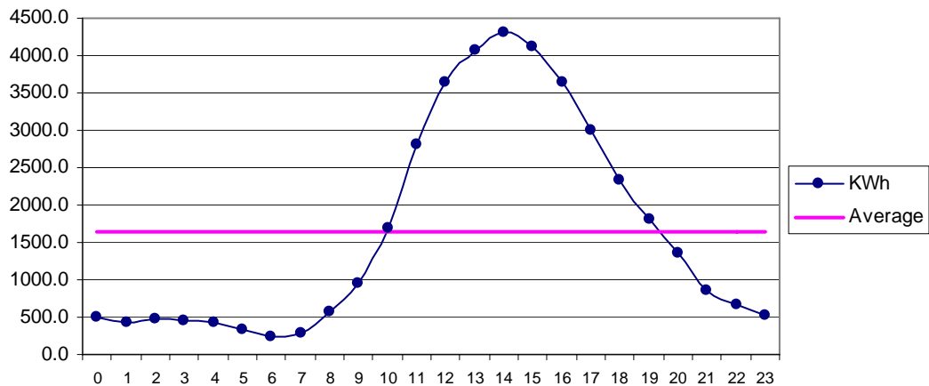
Fig 29 Ramra Jun: Diurnal Variation of Wind Genrated Electric Energy Output
