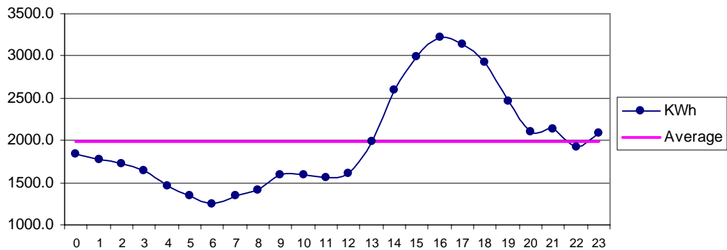
Fig 26 Pishukan Mar: Diurnal Variation of Wind Genrated Electric Energy Output
