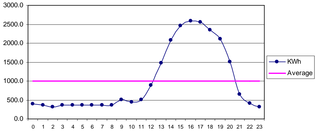
Fig 33 Pishukan Oct: Diurnal Variation of Wind Genrated Electric Energy Output
