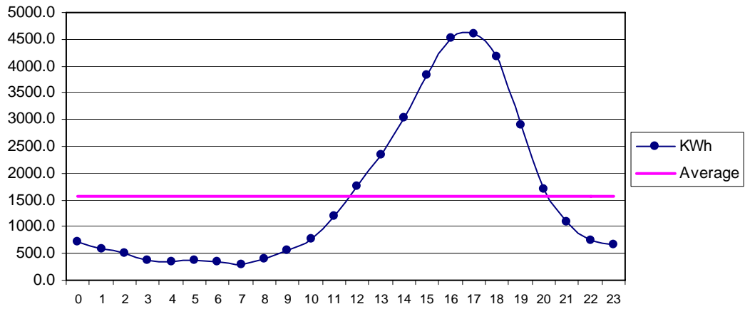
Fig 31 Pishukan Aug: Diurnal Variation of Wind Genrated Electric Energy Output
