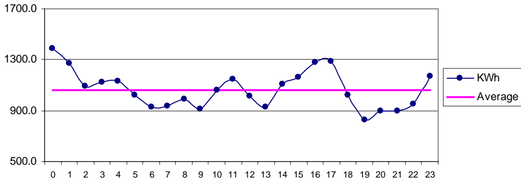
Fig 24 Pishukan Jan: Diurnal Variation of Wind Genrated Electric Energy Output
