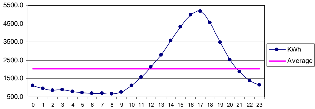
Fig 30 Pishukan July: Diurnal Variation of Wind Genrated Electric Energy Output
