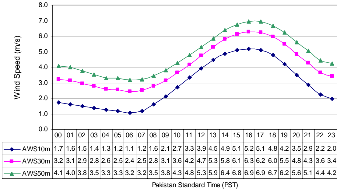
Diurnal Variation of Wind Speed at Pishukan (Mar to May) in three Years
