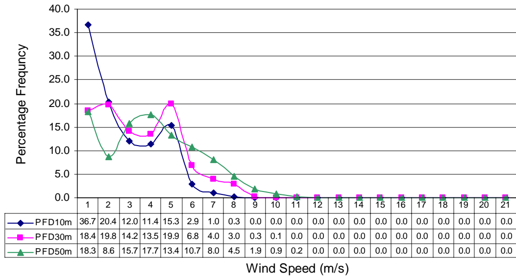
Percentage Wind Frequency Distribution at Pishukan (Sep to Nov) in three years
