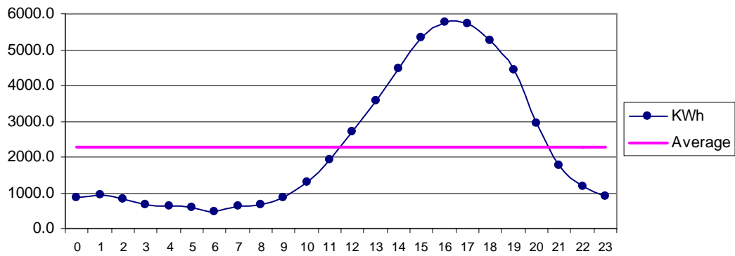
Fig 28 Pishukan May: Diurnal Variation of Wind Genrated Electric Energy Output
