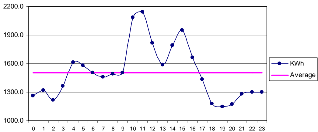
Fig 35 Pishukan Dec: Diurnal Variation of Wind Genrated Electric Energy Output
