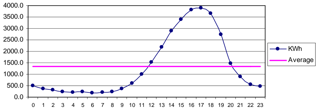
Fig 32 Pishukan Sep: Diurnal Variation of Wind Genrated Electric Energy Output
