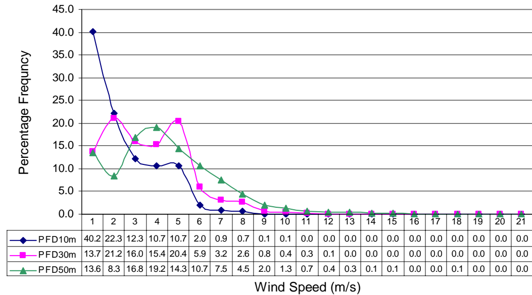
Percentage Wind Frequency Distribution at Pishukan (Dec to Feb) in three years
