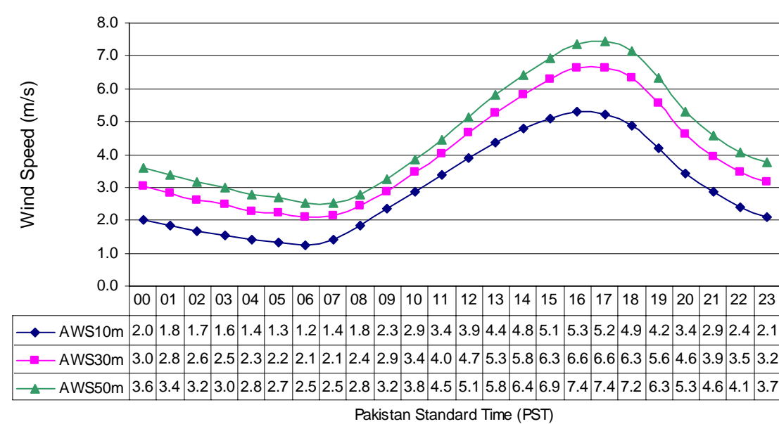
Diurnal Variation of Wind Speed at Pishukan (Jun to Aug) in three Years
