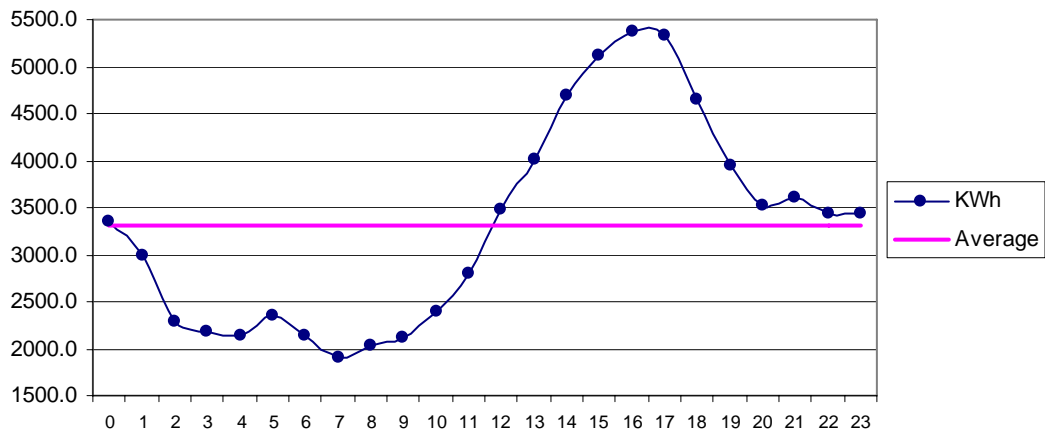
Fig 27 Pishukan Apr: Diurnal Variation of Wind Genrated Electric Energy Output
