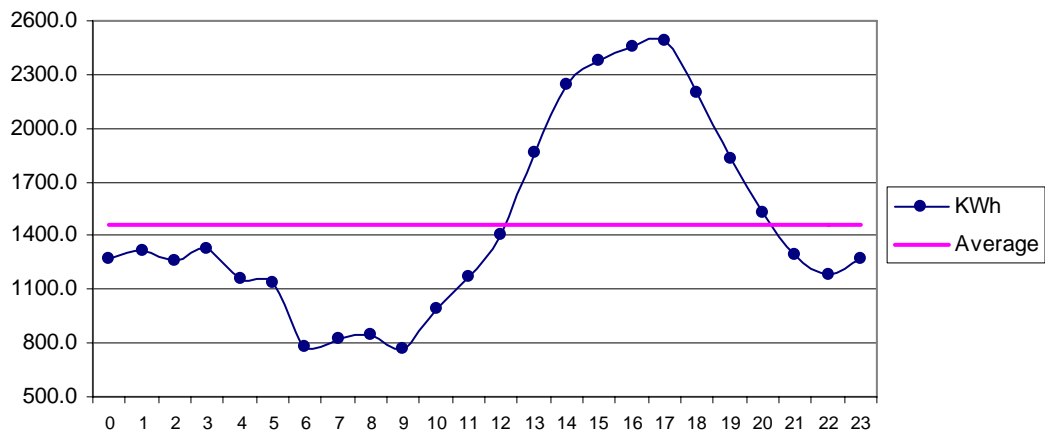
Fig 25 Pishukan Feb: Diurnal Variation of Wind Genrated Electric Energy Output
