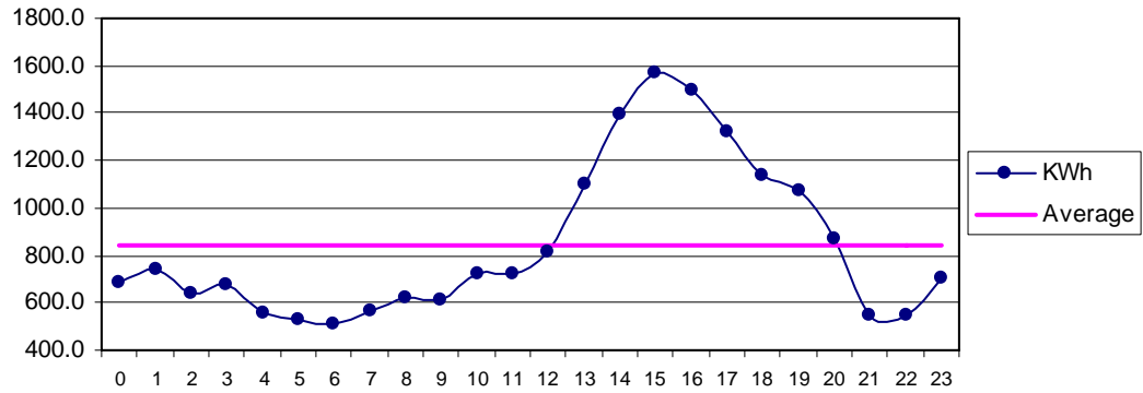
Fig 34 Pishukan Nov. Diurnal Variation of Wind Genrated Electric Energy Output
