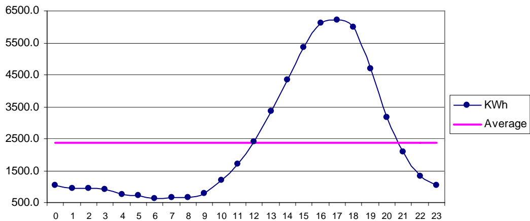
Fig 29 Pishukan Jun: Diurnal Variation of Wind Genrated Electric Energy Output
