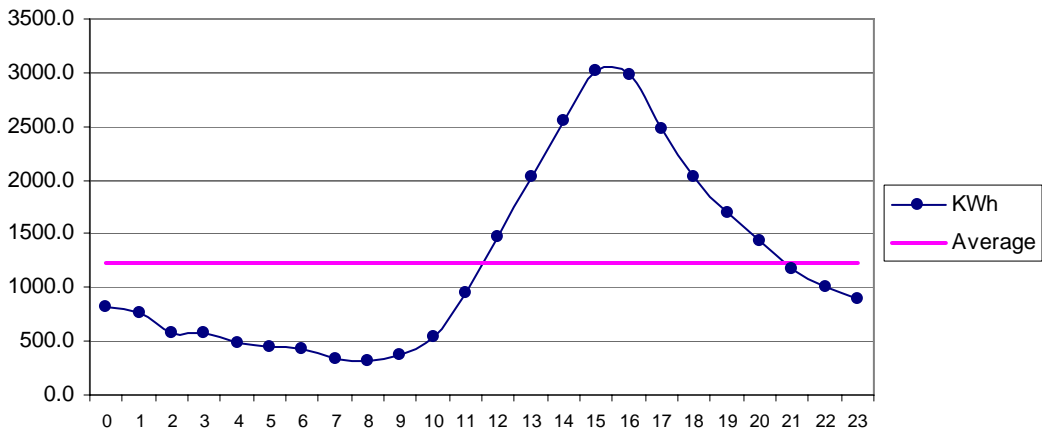
Fig 25 Phore Feb: Diurnal Variation of Wind Genrated Electric Energy Output
