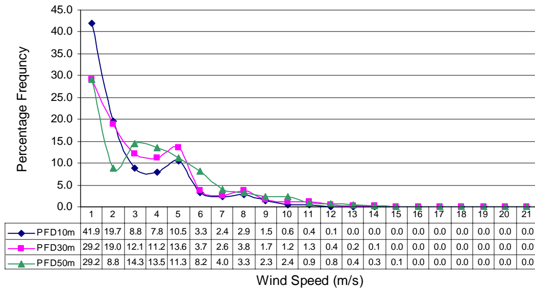
Fig-18 Percentage Wind Frequency Distribution at Phore (Dec to Feb) in three years
