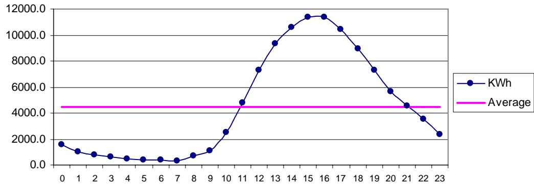
Fig 28 Phore May: Diurnal Variation of Wind Genrated Electric Energy Output
