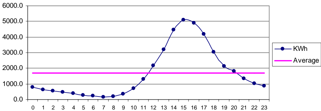
Fig 26 Phore Mar: Diurnal Variation of Wind Genrated Electric Energy Output
