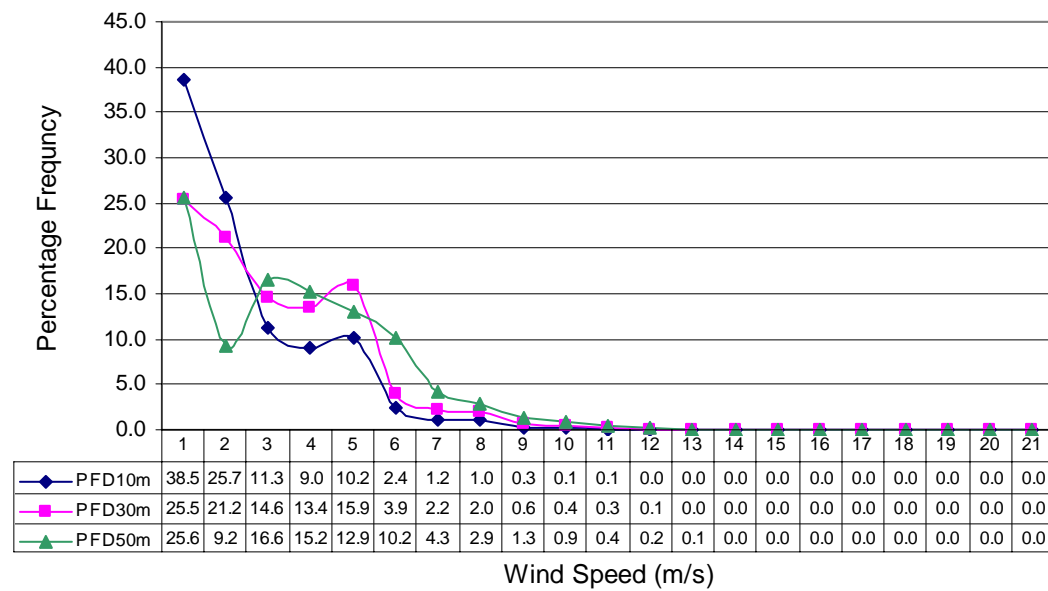
Fig-18 Percentage Wind Frequency Distribution at Phore (Dec to Feb) in three years
