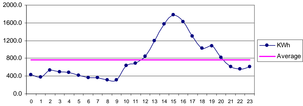
Fig 24 Phore Jan: Diurnal Variation of Wind Genrated Electric Energy Output
