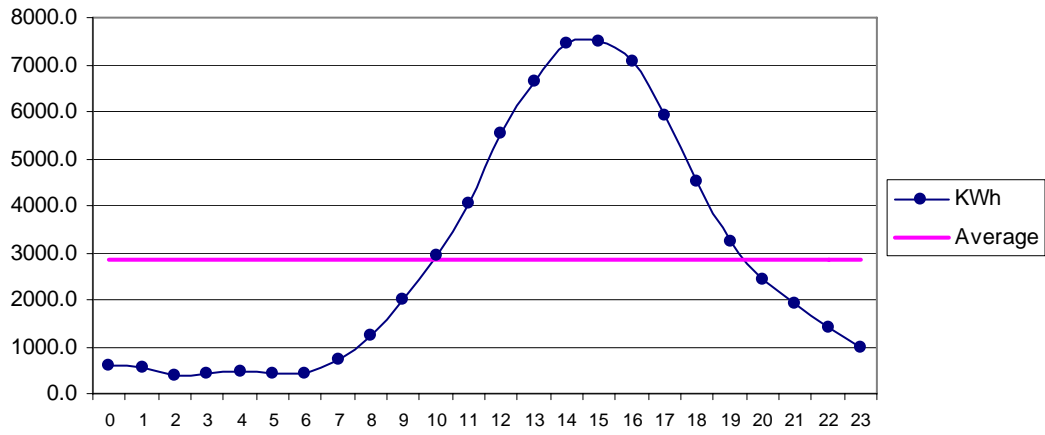
Fig 27 Phore Apr: Diurnal Variation of Wind Genrated Electric Energy Output
