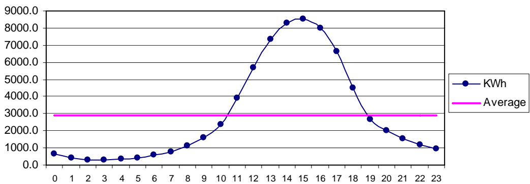
Fig 32 Phore Sep: Diurnal Variation of Wind Genrated Electric Energy Output
