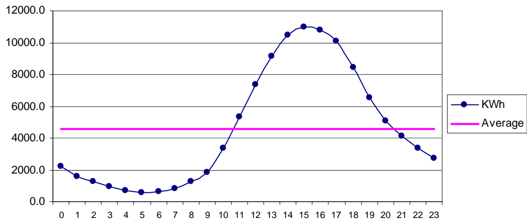
Fig 29 Phore Jun: Diurnal Variation of Wind Genrated Electric Energy Output
