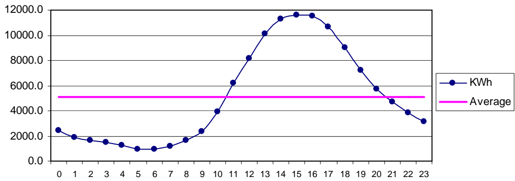
Fig 30 Phore July: Diurnal Variation of Wind Genrated Electric Energy Output
