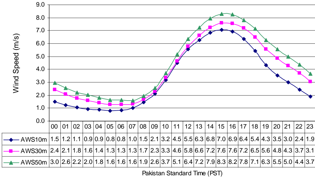
Fig-4 Diurnal Variation of Wind Speed at Phore (Mar to May) in three Years
