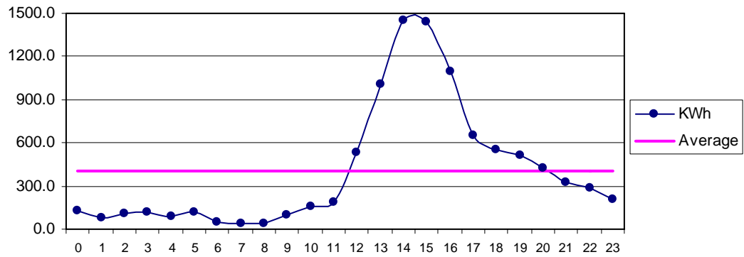
Fig 34 Phore Nov: Diurnal Variation of Wind Genrated Electric Energy Output
