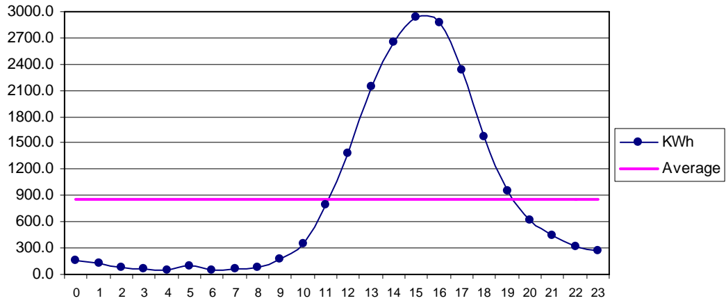
Fig 33 Phore Oct: Diurnal Variation of Wind Genrated Electric Energy Output
