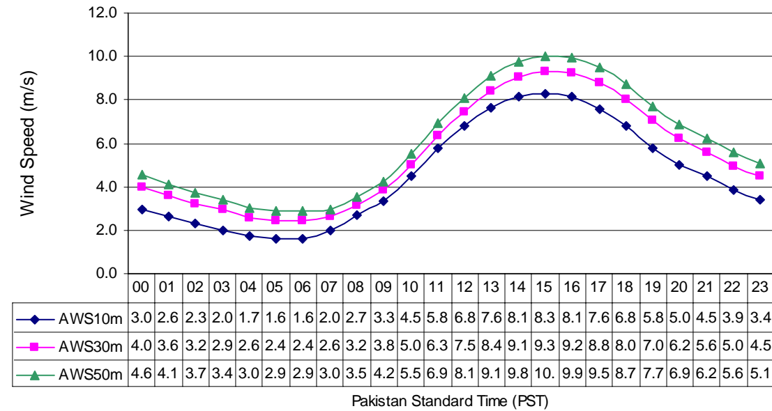
Fig-5 Diurnal Variation of Wind Speed at Phore (Jun to Aug) in three Years
