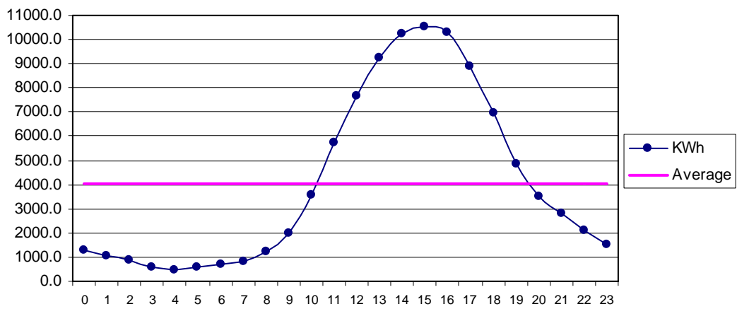
Fig 31 Phore Aug: Diurnal Variation of Wind Genrated Electric Energy Output
