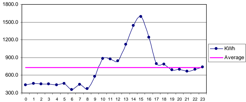
Fig 35 Phore Dec: Diurnal Variation of Wind Genrated Electric Energy Output
