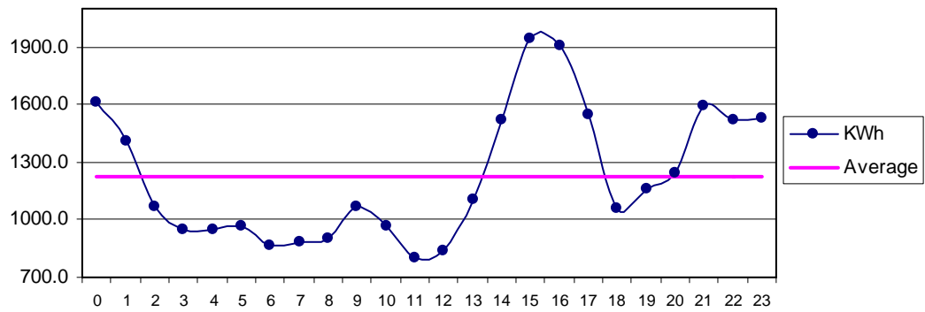
Fig 34 Pasni Nov: Diurnal Variation of Wind Genrated Electric Energy Output
