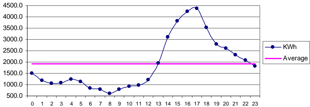
Fig 26 Pasni Mar: Diurnal Variation of Wind Genrated Electric Energy Output
