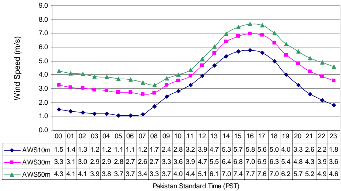
Fig-4 Diurnal Variation of Wind Speed at Pasni (Mar to May) in three Years
