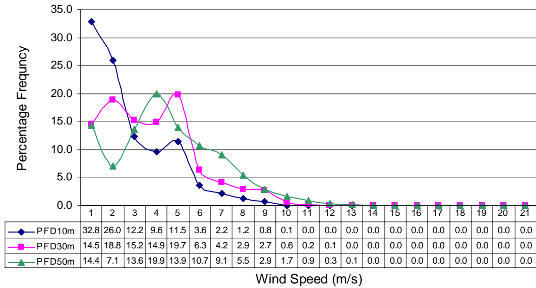
Fig-18 Percentage Wind Frequency Distribution at Pasni (Dec to Feb) in three years
