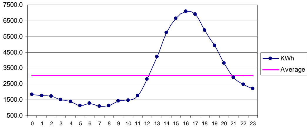
Fig 27 Pasni Apr: Diurnal Variation of Wind Genrated Electric Energy Output
