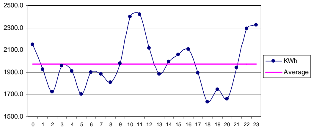
Fig 35 Pasni Dec: Diurnal Variation of Wind Genrated Electric Energy Output
