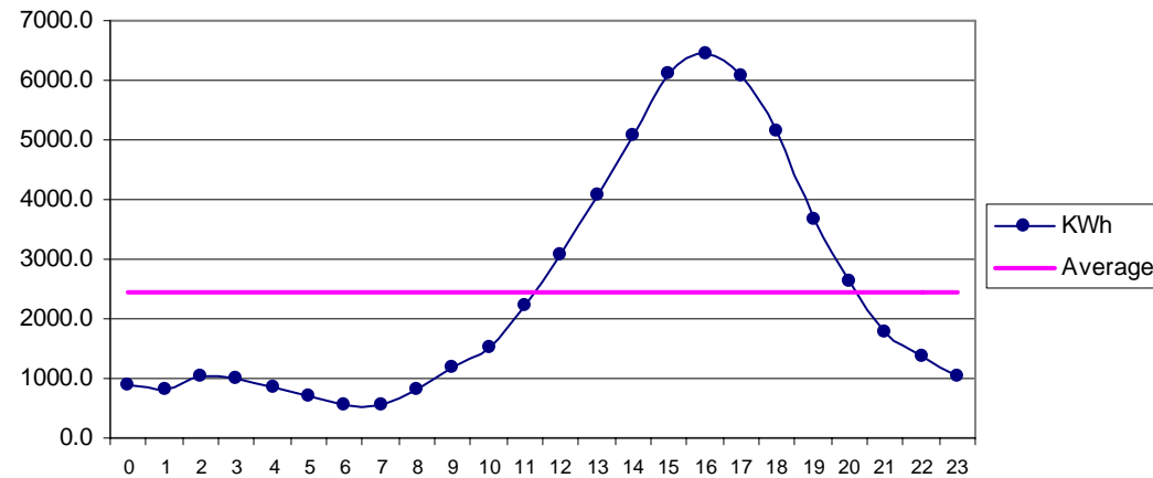
Fig 29 Pasni Jun: Diurnal Variation of Wind Genrated Electric Energy Output
