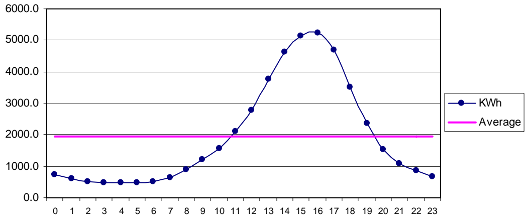
Fig 31 Pasni Aug: Diurnal Variation of Wind Genrated Electric Energy Output
