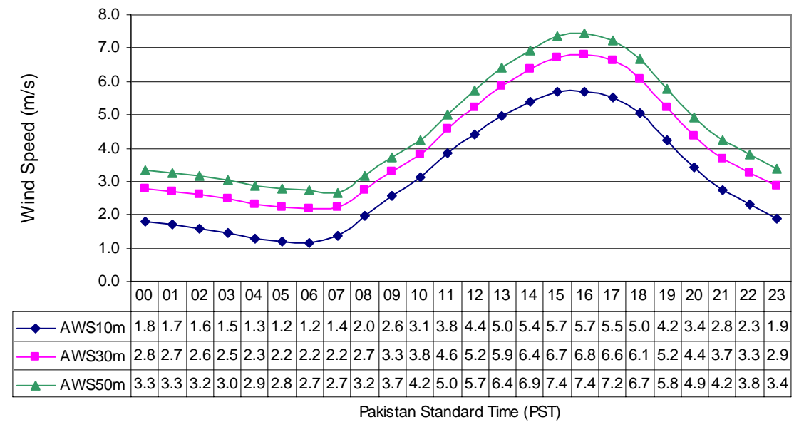
Fig-5 Diurnal Variation of Wind Speed at Pasni (Jun to Aug) in three Years
