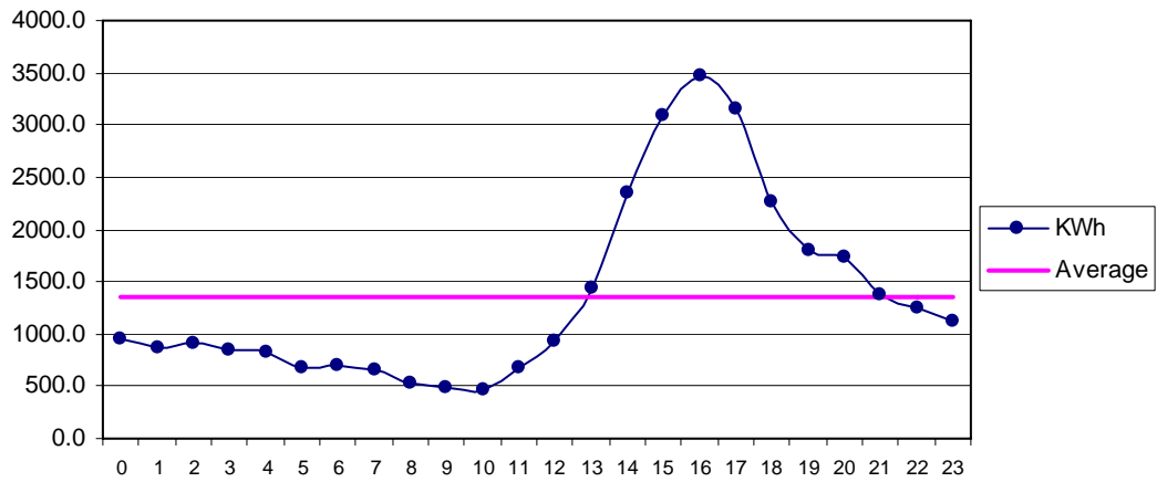
Fig 33 Pasni Oct: Diurnal Variation of Wind Genrated Electric Energy Output
