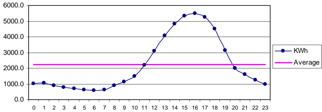
Fig 30 Pasni July: Diurnal Variation of Wind Genrated Electric Energy Output
