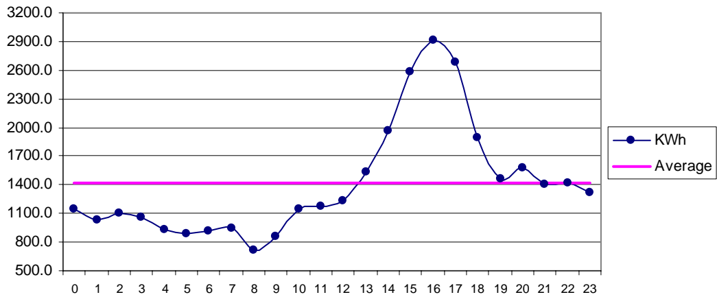
Fig 25 Pasni Feb: Diurnal Variation of Wind Genrated Electric Energy Output
