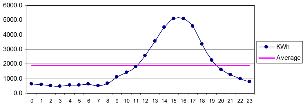
Fig 32 Pasni Sep: Diurnal Variation of Wind Genrated Electric Energy Output
