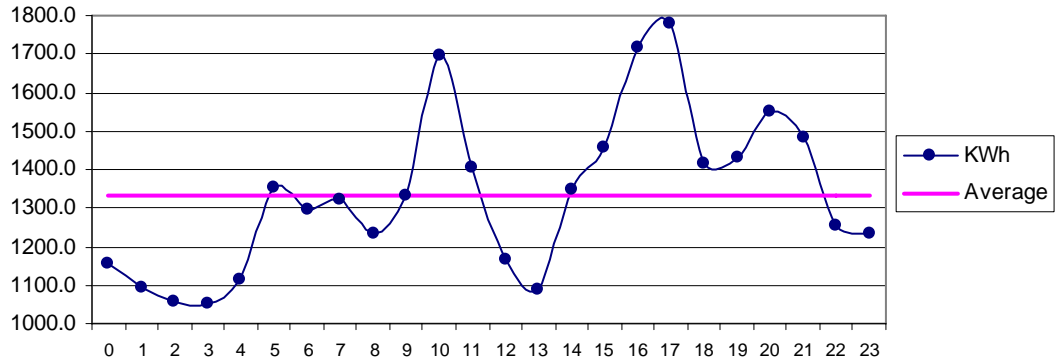
Fig 24 Pasni Jan: Diurnal Variation of Wind Genrated Electric Energy Output
