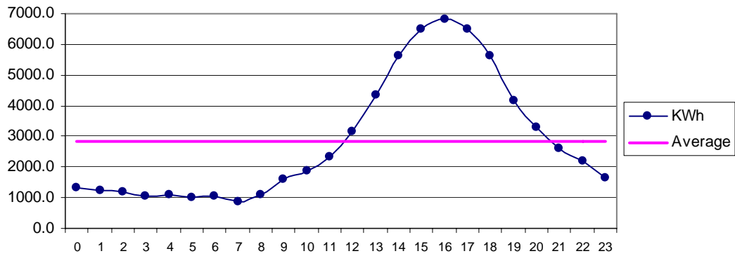
Fig 28 Pasni May: Diurnal Variation of Wind Genrated Electric Energy Output
