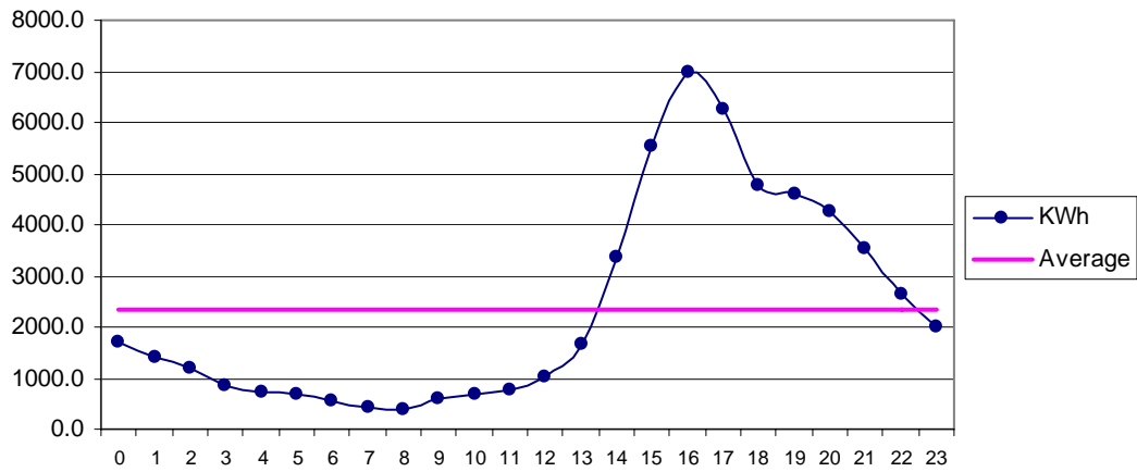
Fig 27 Othal Apr: Diurnal Variation of Wind Genrated Electric Energy Output
