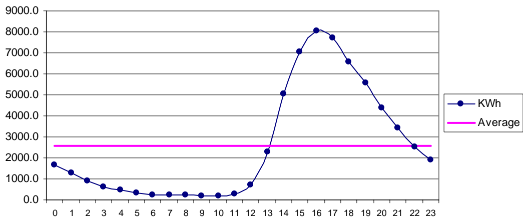
Fig 29 Othal Jun: Diurnal Variation of Wind Genrated Electric Energy Output
