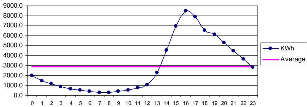
Fig 28 Othal May: Diurnal Variation of Wind Genrated Electric Energy Output
