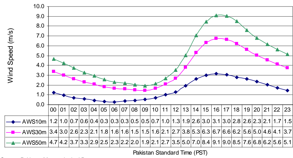
Diurnal Variation of Wind Speed at Othal (Jun to Aug) in three Years
