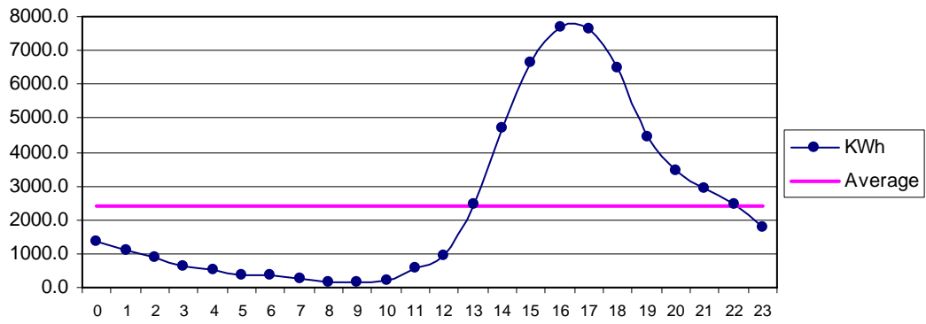
Fig 30 Othal July: Diurnal Variation of Wind Genrated Electric Energy Output
