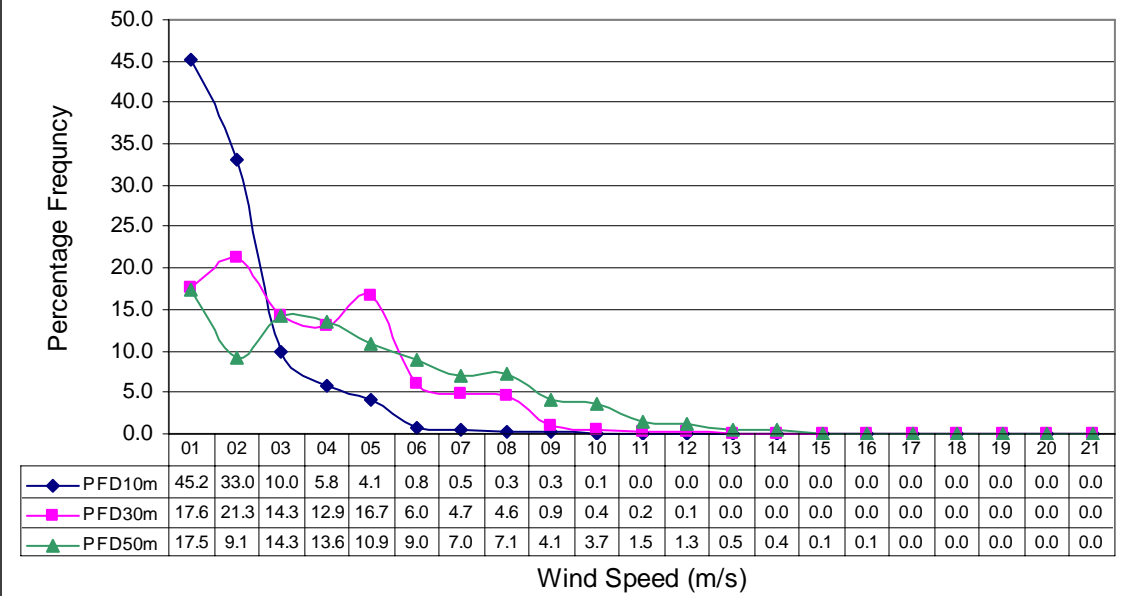
Annual Percentage Wind Frequency Distribution at Othal in three years
