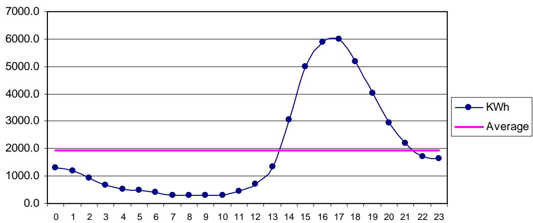
Fig 31 Othal Aug: Diurnal Variation of Wind Genrated Electric Energy Output
