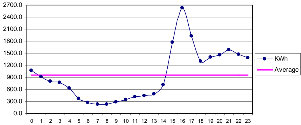
Fig 33 Othal Oct: Diurnal Variation of Wind Genrated Electric Energy Output
