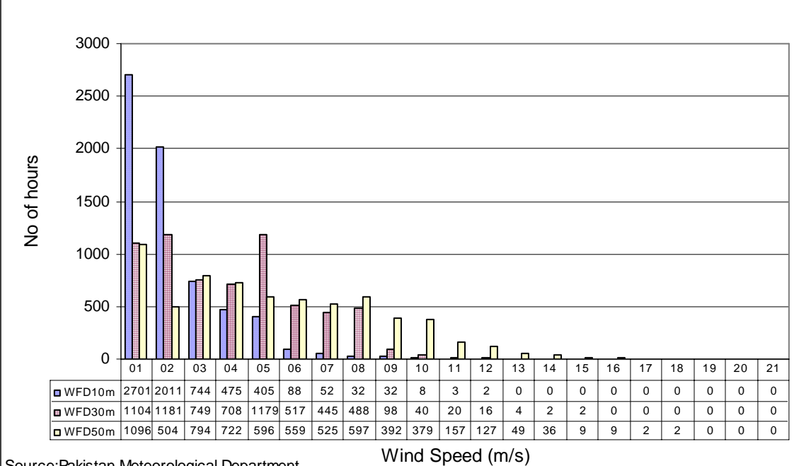
Wind Frequency Distribution at Othal (Mar to May) in three years
