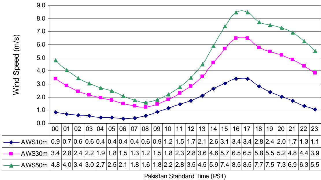
Diurnal Variation of Wind Speed at Othal (Mar to May) in three Years
