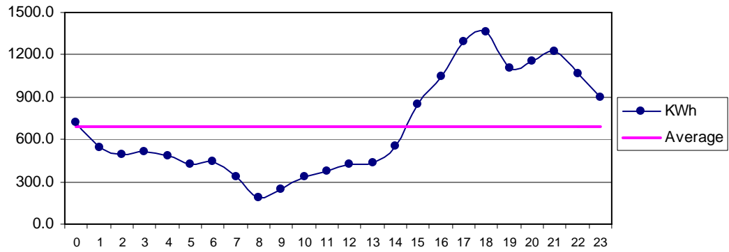
Fig 34 Othal Nov: Diurnal Variation of Wind Genrated Electric Energy Output
