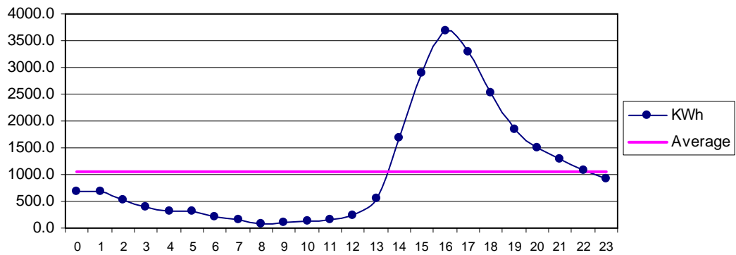
Fig 32 Othal Sep: Diurnal Variation of Wind Genrated Electric Energy Output
