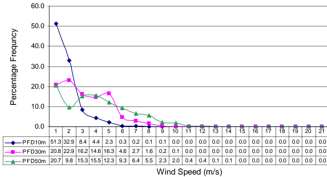
Fig-18 Percentage Wind Frequency Distribution at Othal (Dec to Feb) in three years
