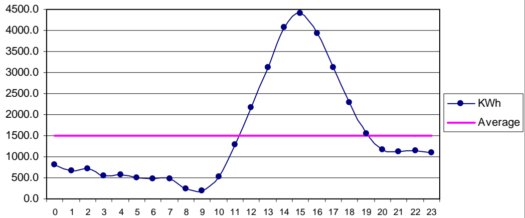
Fig 33 Ormara Oct: Diurnal Variation of Wind Genrated Electric Energy Output
