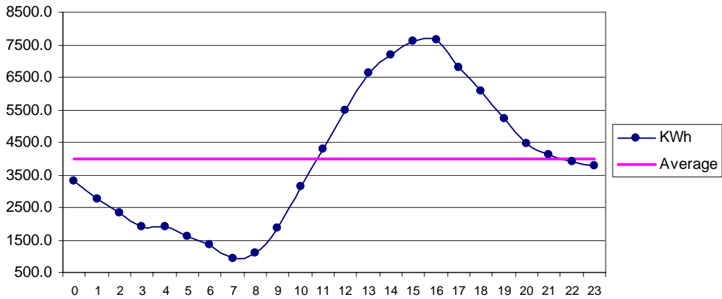
Fig 27 Ormara Apr: Diurnal Variation of Wind Genrated Electric Energy Output
