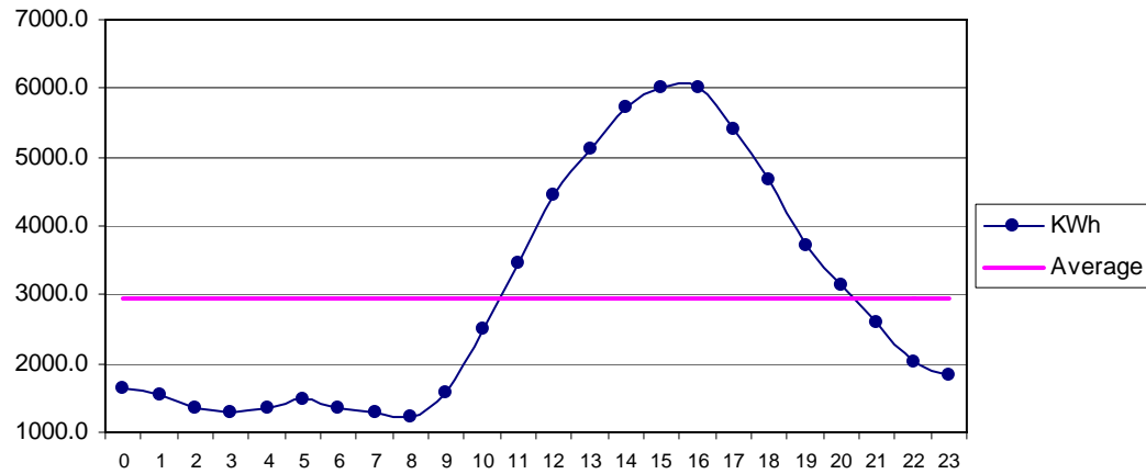
Fig 31 Ormara Aug: Diurnal Variation of Wind Genrated Electric Energy Output
