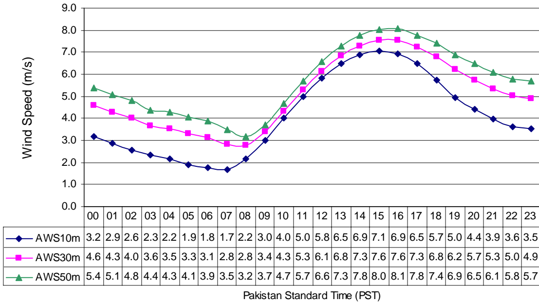
Diurnal Variation of Wind Speed at Ormara (Mar to May) in three Years
