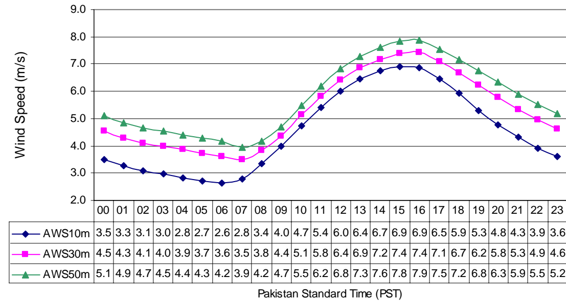
Diurnal Variation of Wind Speed at Ormara (Jun to Aug) in three Years
