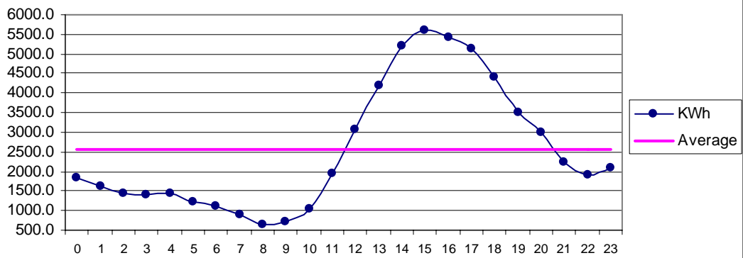
Fig 26 Ormara Mar: Diurnal Variation of Wind Genrated Electric Energy Output
