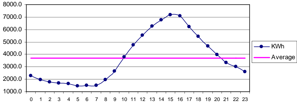
Fig 30 Ormara July: Diurnal Variation of Wind Genrated Electric Energy Output
