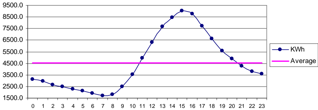
Fig 28 Ormara May: Diurnal Variation of Wind Genrated Electric Energy Output
