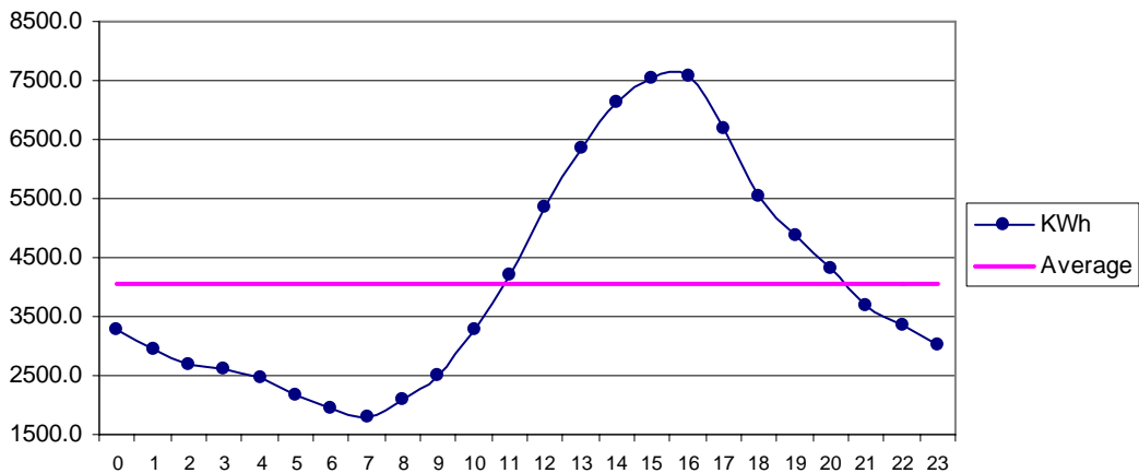
Fig 29 Ormara Jun: Diurnal Variation of Wind Genrated Electric Energy Output
