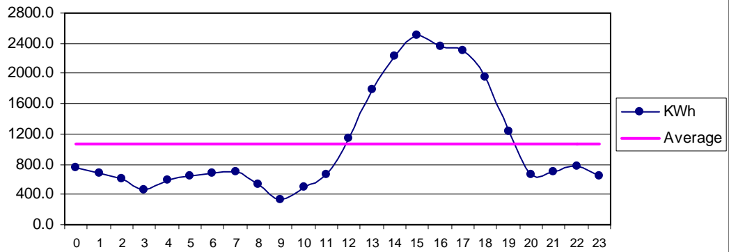
Fig 34 Ormara Nov: Diurnal Variation of Wind Genrated Electric Energy Output
