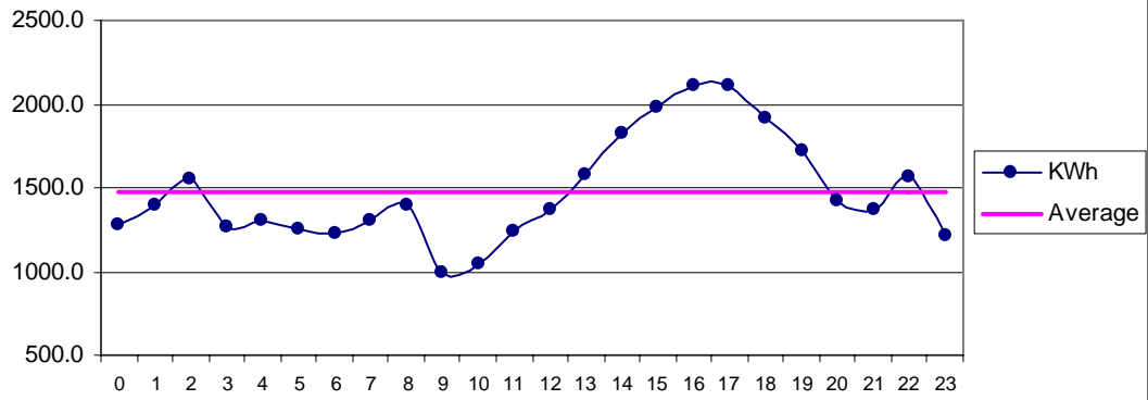
Fig 24 Ormara Jan: Diurnal Variation of Wind Genrated Electric Energy Output
