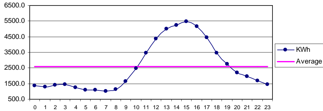
Fig 32 Ormara Sep: Diurnal Variation of Wind Genrated Electric Energy Output
