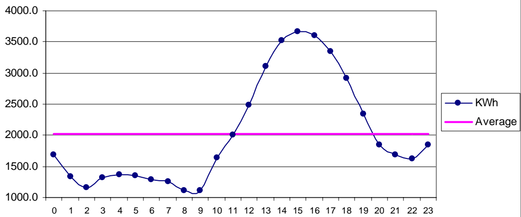
Fig 25 Ormara Feb: Diurnal Variation of Wind Genrated Electric Energy Output
