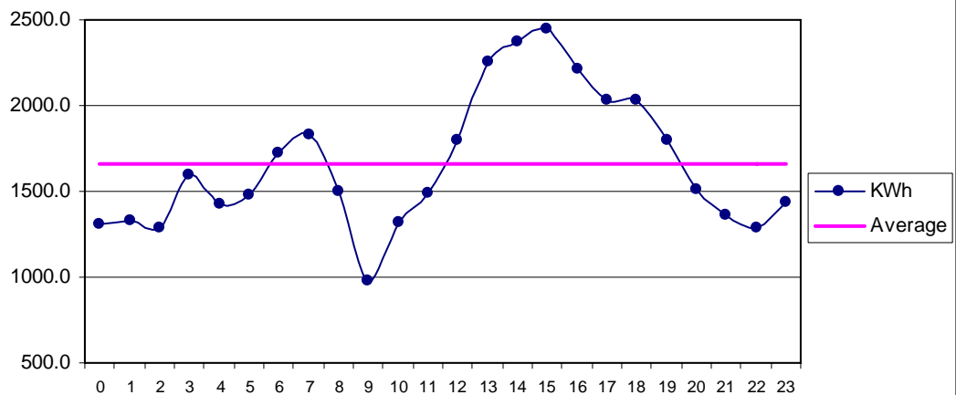
Fig 35 Ormara Dec: Diurnal Variation of Wind Genrated Electric Energy Output
