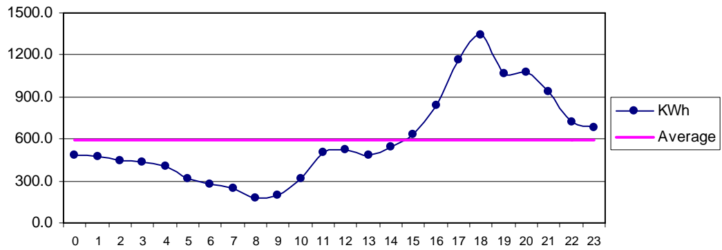
Fig 34 Nasirabad Nov: Diurnal Variation of Wind Genrated Electric Energy Output
