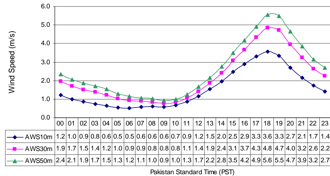
Diurnal Variation of Wind Speed at Nasirabad (Jun to Aug) in three Years
