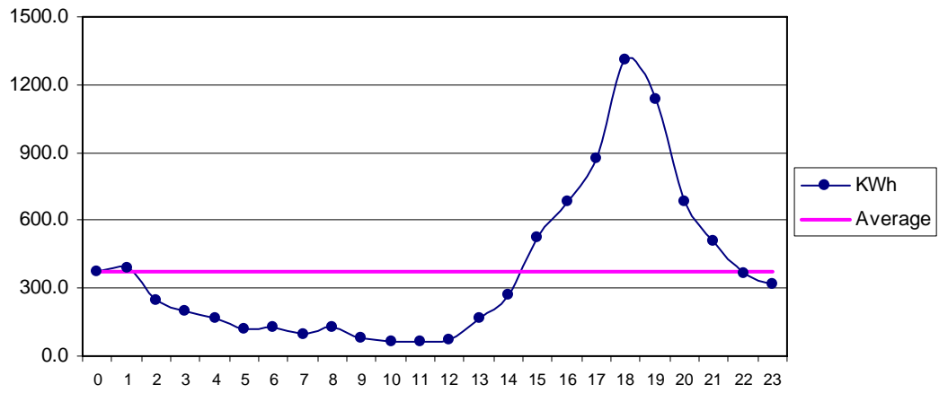
Fig 33 Nasirabad Oct: Diurnal Variation of Wind Genrated Electric Energy Output
