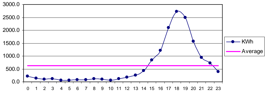
Fig 30 Nasirabad July: Diurnal Variation of Wind Genrated Electric Energy Output
