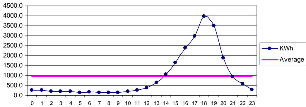
Fig 28 Nasirabad May: Diurnal Variation of Wind Genrated Electric Energy Output
