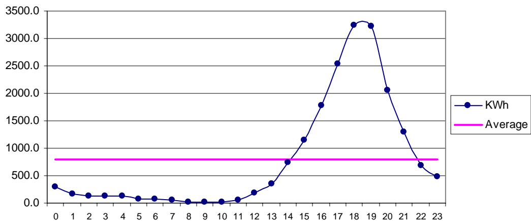
Fig 29 Nasirabad Jun: Diurnal Variation of Wind Genrated Electric Energy Output
