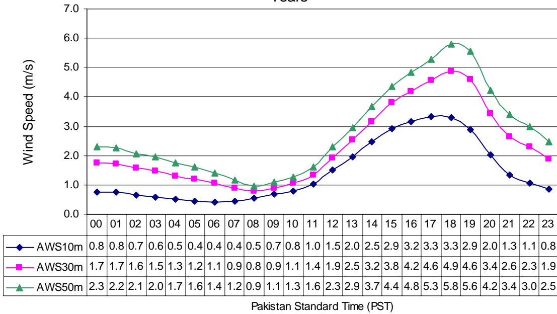
Diurnal Variation of Wind Speed at Nasirabad (Mar to May) in three Years
