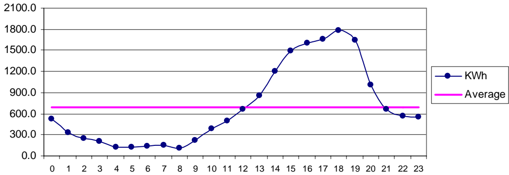
Fig 26 Nasirabad Mar: Diurnal Variation of Wind Genrated Electric Energy Output
