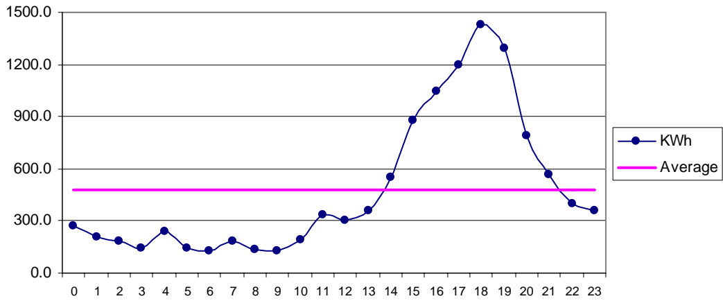
Fig 25 Nasirabad Feb: Diurnal Variation of Wind Genrated Electric Energy Output
