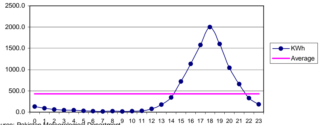
Fig 31 Nasirabad Aug: Diurnal Variation of Wind Genrated Electric Energy Output
