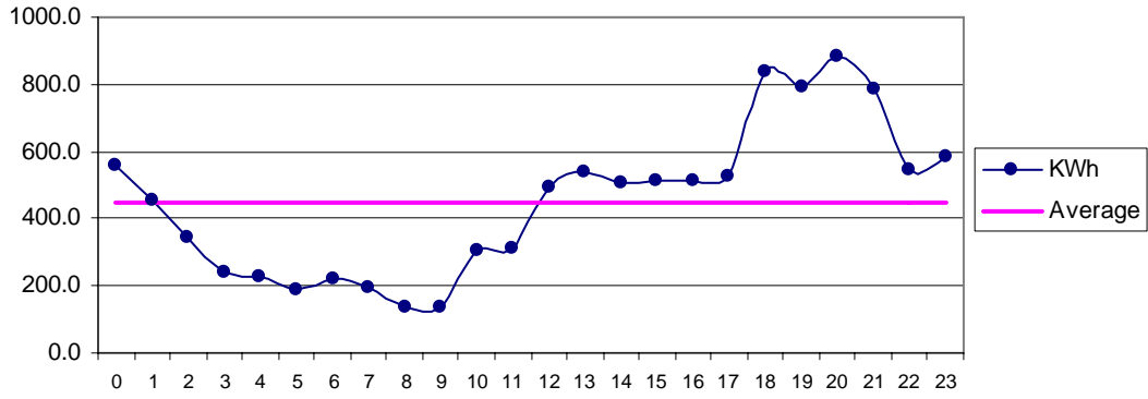
Fig 24 Nasirabad Jan: Diurnal Variation of Wind Genrated Electric Energy Output
