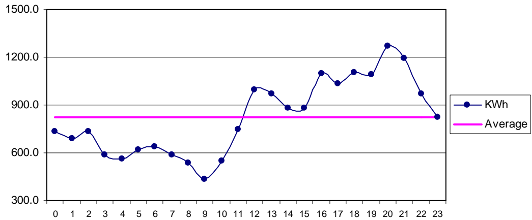
Fig 35 Nasirabad Dec: Diurnal Variation of Wind Genrated Electric Energy Output
