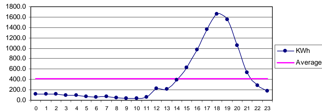
Fig 32 Nasirabad Sep: Diurnal Variation of Wind Genrated Electric Energy Output
