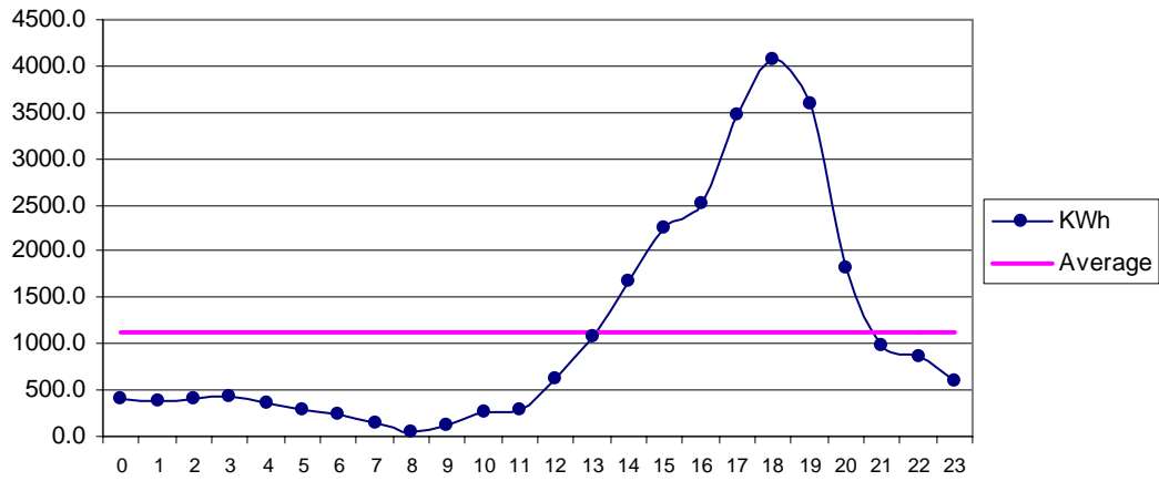
Fig 27 Nasirabad Apr: Diurnal Variation of Wind Genrated Electric Energy Output
