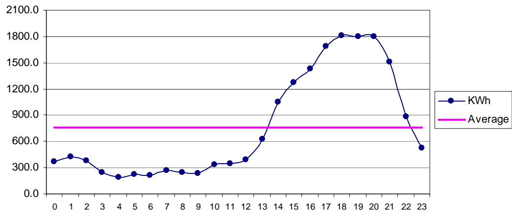
Fig 25 Mand Feb: Diurnal Variation of Wind Genrated Electric Energy Output
