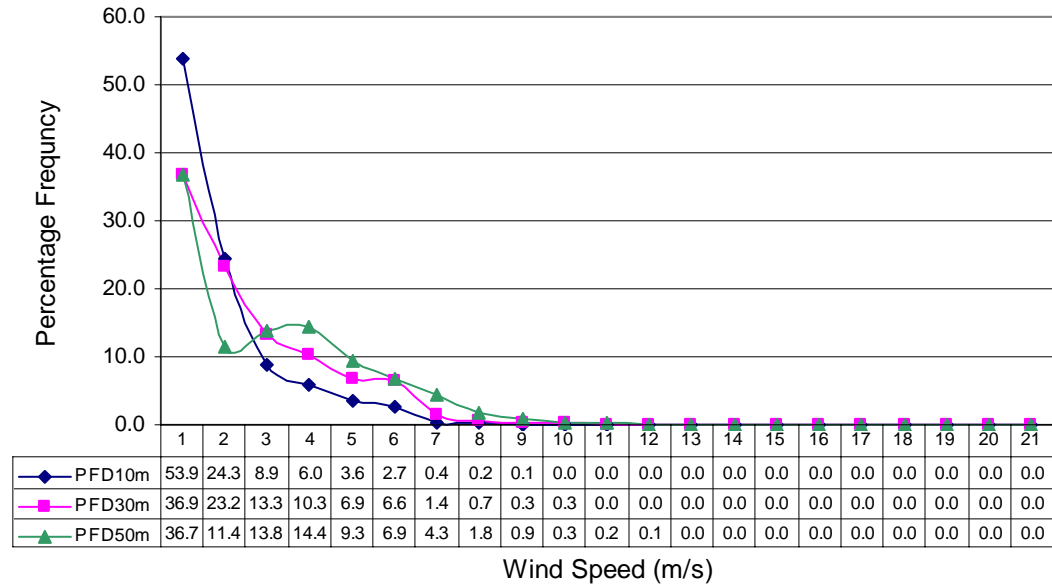
Percentage Wind Frequency Distribution at Mand (Dec to Feb) in three years
