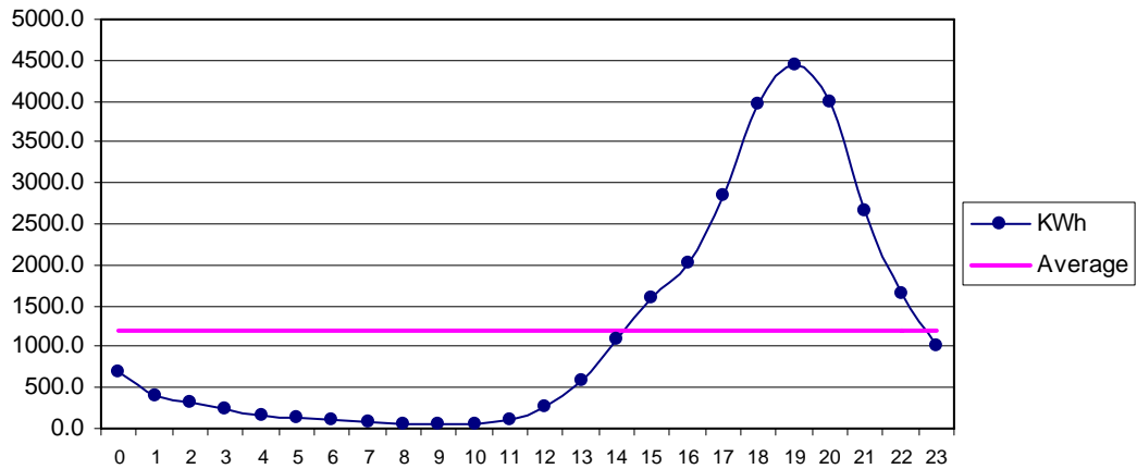
Fig 31 Mand Aug: Diurnal Variation of Wind Genrated Electric Energy Output
