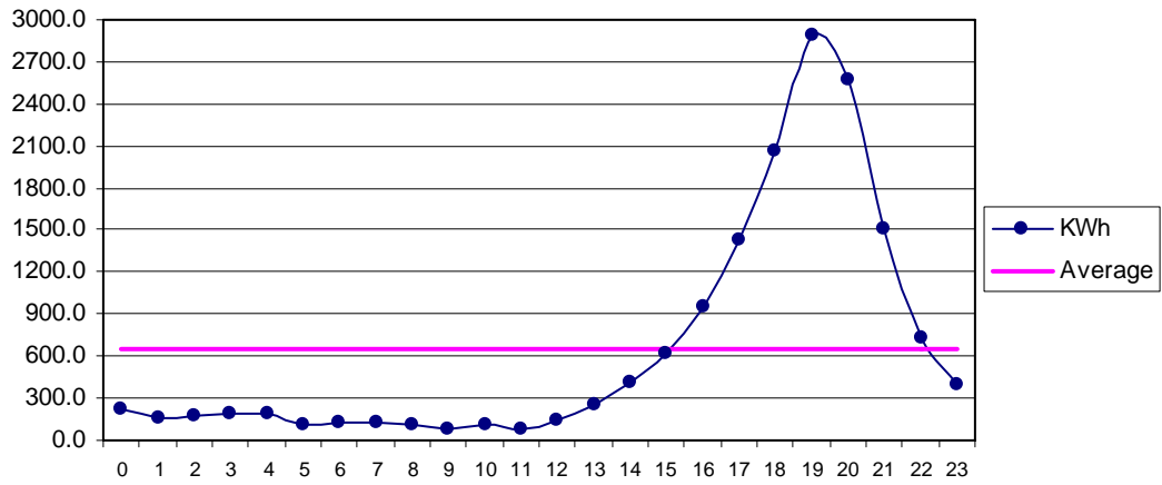
Fig 33 Mand Oct: Diurnal Variation of Wind Genrated Electric Energy Output
