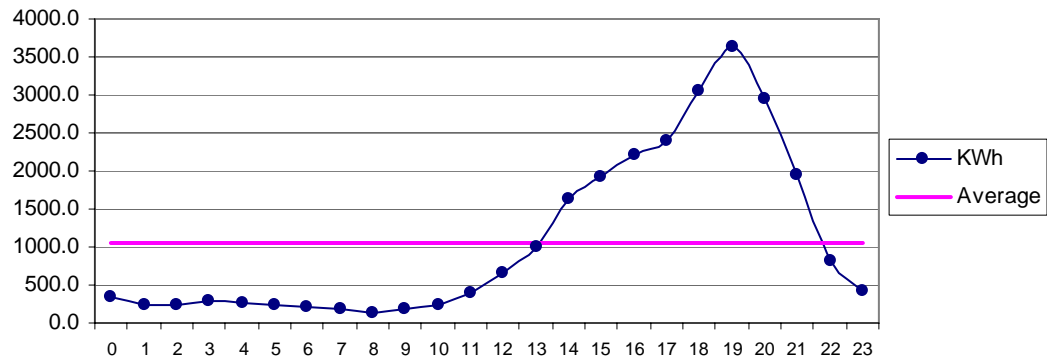
Fig 26 Mand Mar: Diurnal Variation of Wind Genrated Electric Energy Output
