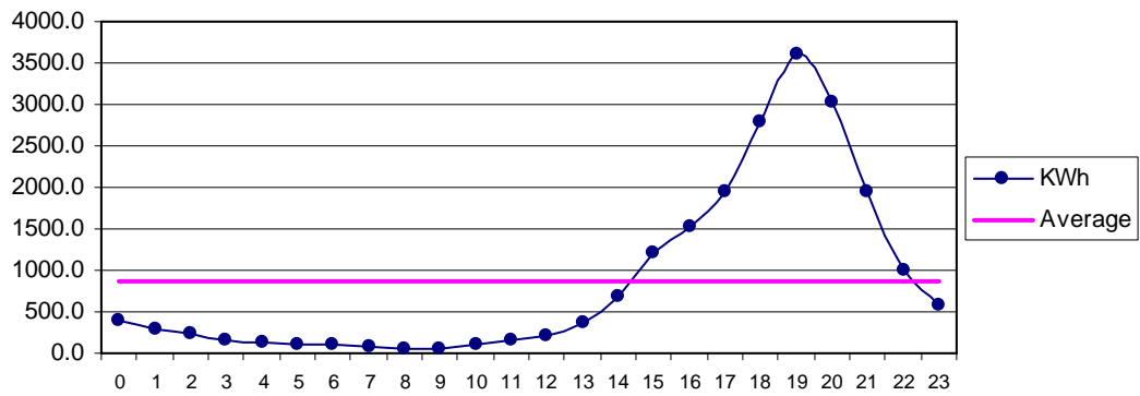
Fig 32 Mand Sep: Diurnal Variation of Wind Genrated Electric Energy Output
