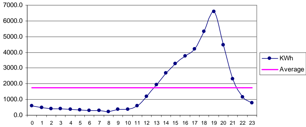
Fig 27 Mand Apr: Diurnal Variation of Wind Genrated Electric Energy Output
