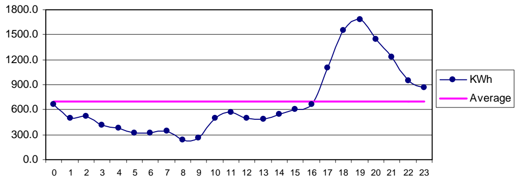
Fig 34 Mand Nov: Diurnal Variation of Wind Genrated Electric Energy Output
