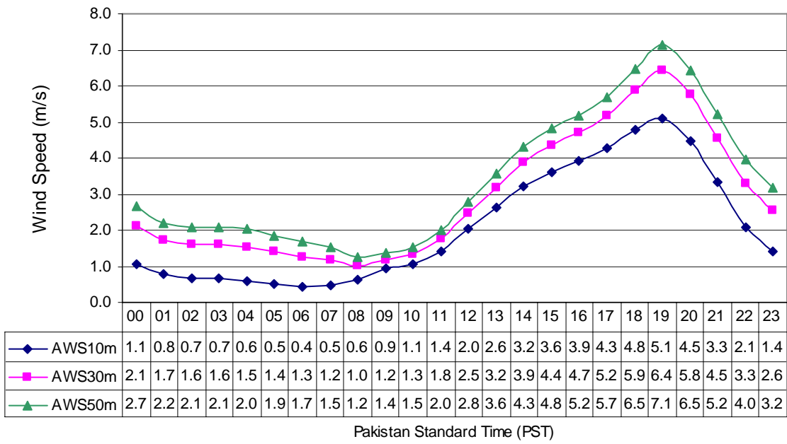
Diurnal Variation of Wind Speed at Mand (Mar to May) in three Years
