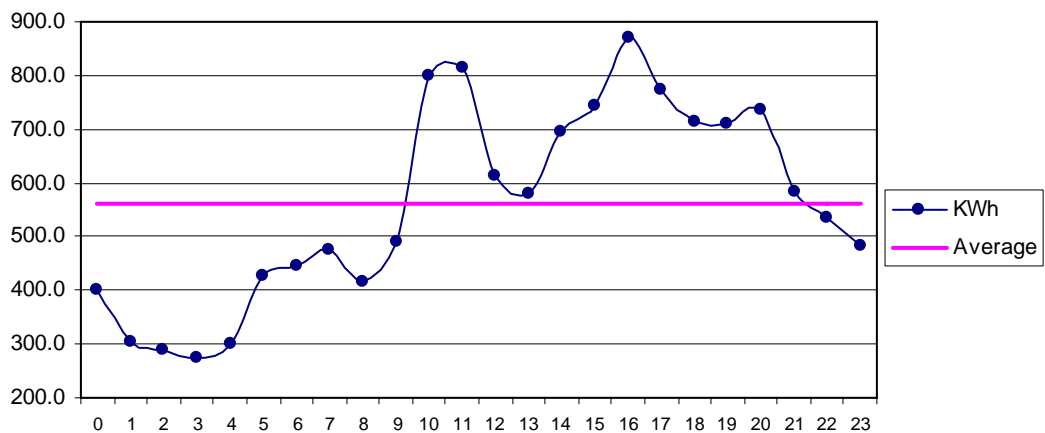
Fig 35 Mand Dec: Diurnal Variation of Wind Genrated Electric Energy Output
