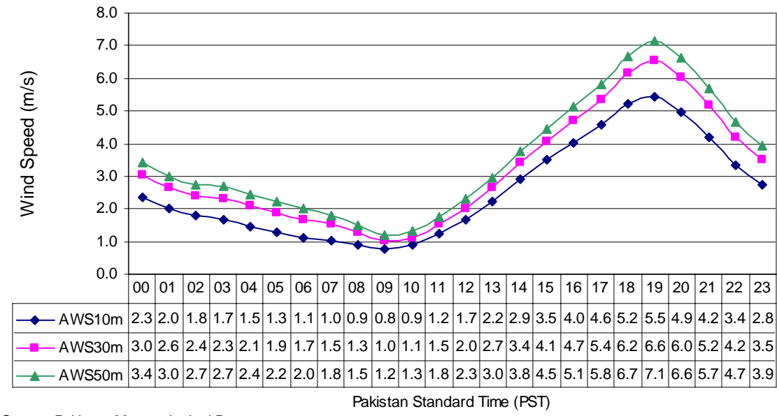
Diurnal Variation of Wind Speed at Mand (Jun to Aug) in three Years
