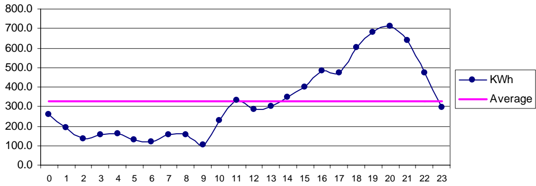
Fig 24 Mand Jan: Diurnal Variation of Wind Genrated Electric Energy Output
