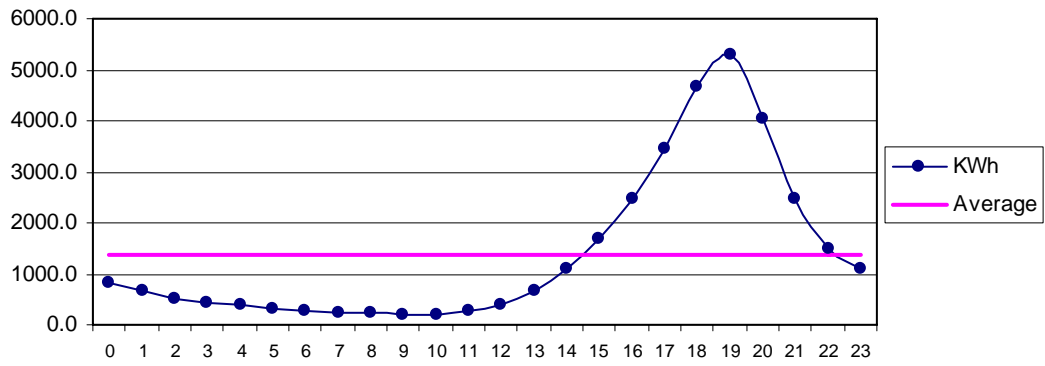
Fig 30 Mand July: Diurnal Variation of Wind Genrated Electric Energy Output
