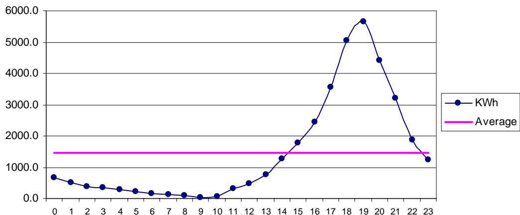
Fig 29 Mand Jun: Diurnal Variation of Wind Genrated Electric Energy Output
