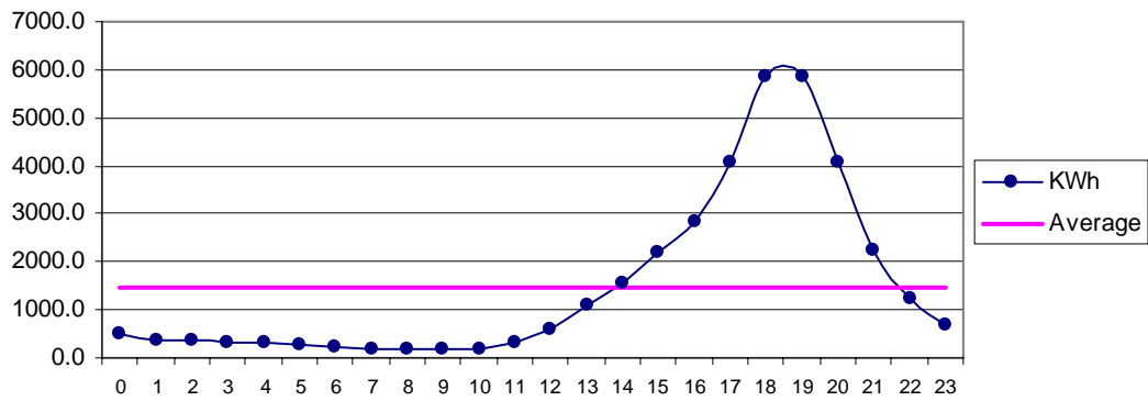
Fig 28 Mand May: Diurnal Variation of Wind Genrated Electric Energy Output
