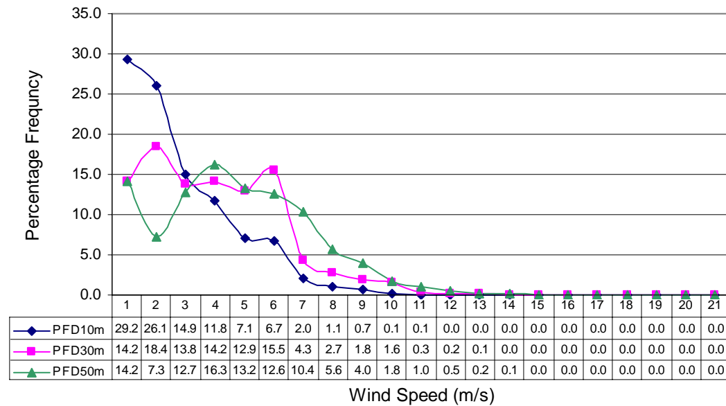
Percentage Wind Frequency Distribution at Managi (Dec to Feb) in three years
