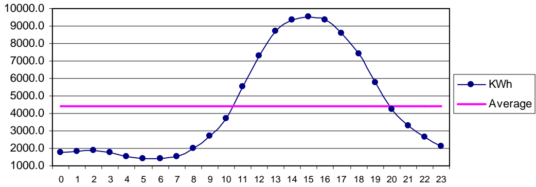
Fig 30 Managi July: Diurnal Variation of Wind Genrated Electric Energy Output
