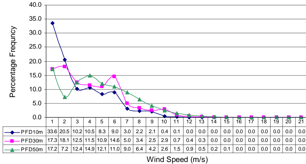
Percentage Wind Frequency Distribution at Managi (Sep to Nov) in three years
