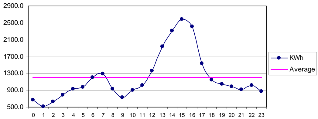
Fig 34 Managi Nov. Diurnal Variation of Wind Genrated Electric Energy Output
