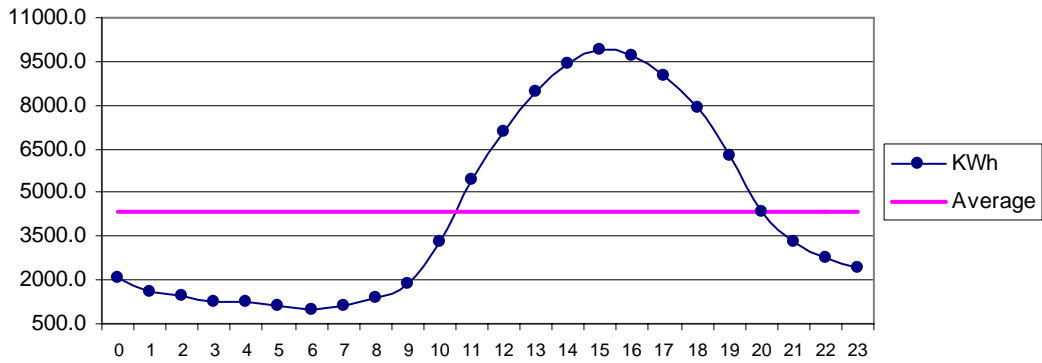
Fig 28 Managi May: Diurnal Variation of Wind Genrated Electric Energy Output
