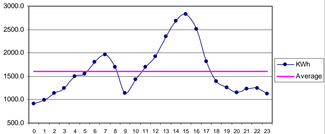
Fig 35 Managi Dec: Diurnal Variation of Wind Genrated Electric Energy Output
