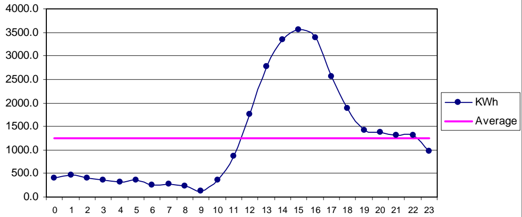
Fig 33 Managi Oct: Diurnal Variation of Wind Genrated Electric Energy Output
