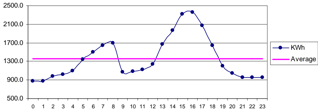
Fig 24 Managi Jan: Diurnal Variation of Wind Genrated Electric Energy Output
