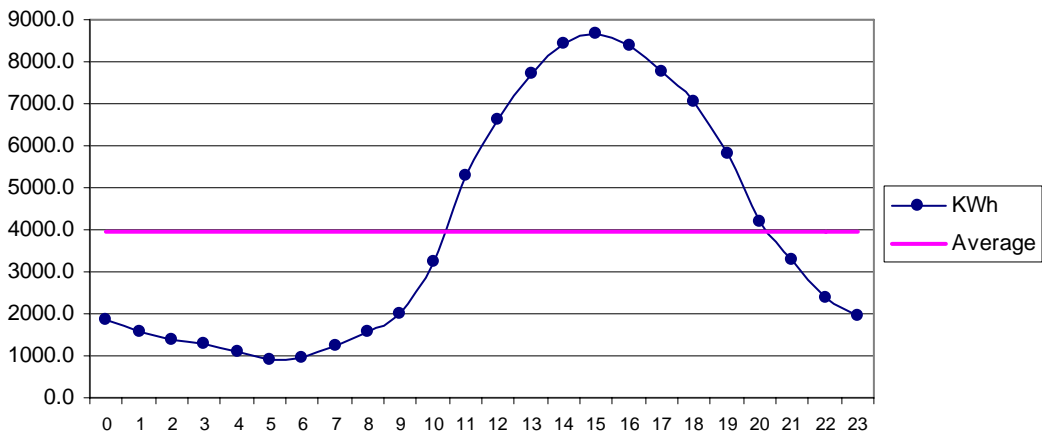
Fig 29 Managi Jun: Diurnal Variation of Wind Genrated Electric Energy Output
