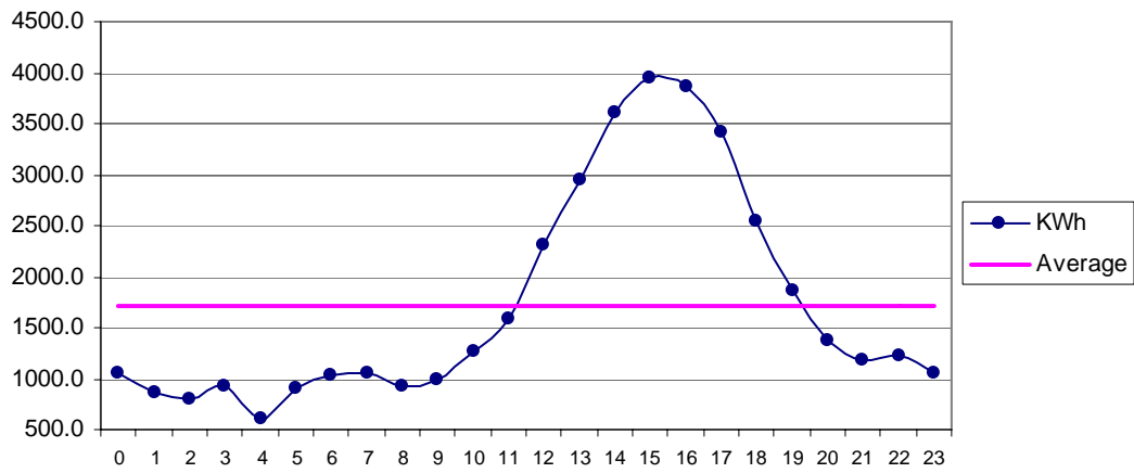
Fig 25 Managi Feb: Diurnal Variation of Wind Genrated Electric Energy Output
