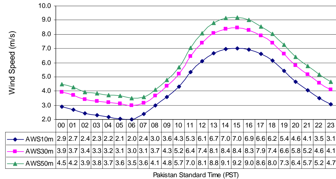
Diurnal Variation of Wind Speed at Managi (Jun to Aug) in three Years
