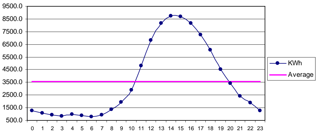
Fig 31 Managi Aug: Diurnal Variation of Wind Genrated Electric Energy Output
