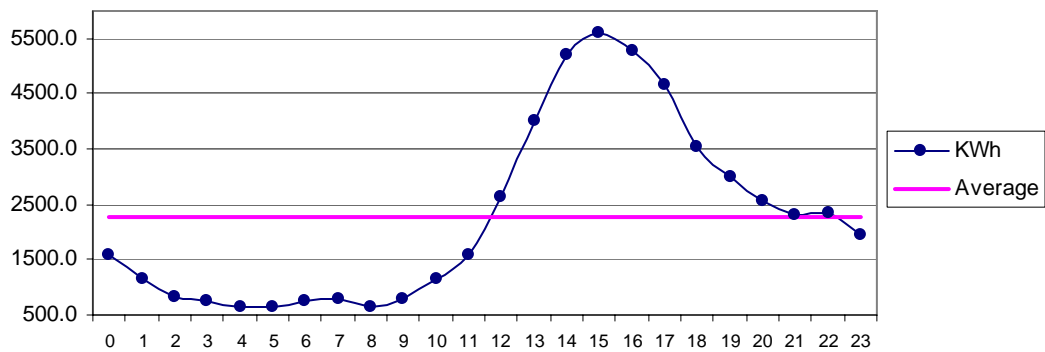
Fig 26 Managi Mar: Diurnal Variation of Wind Genrated Electric Energy Output
