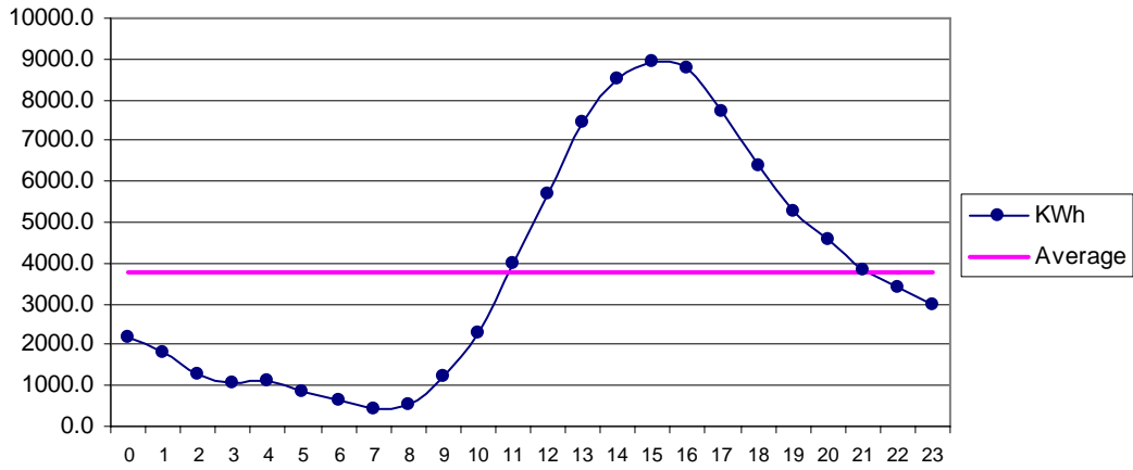
Fig 27 Managi Apr: Diurnal Variation of Wind Genrated Electric Energy Output
