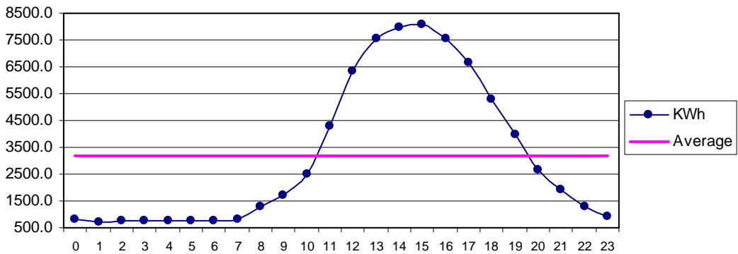
Fig 32 Managi Sep: Diurnal Variation of Wind Genrated Electric Energy Output
