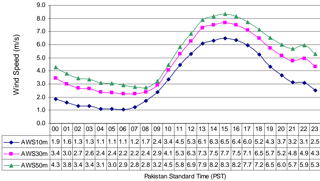
Diurnal Variation of Wind Speed at Managi (Mar to May) in three Years
