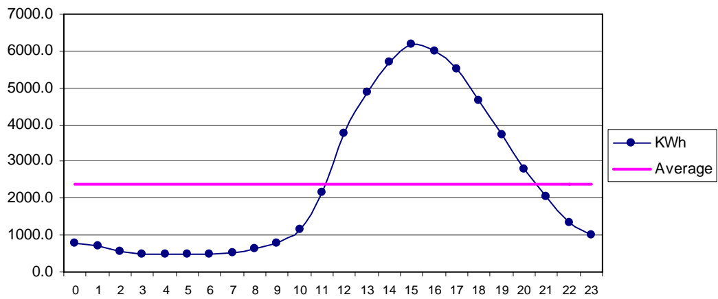
Fig 31 Makola Aug: Diurnal Variation of Wind Genrated Electric Energy Output
