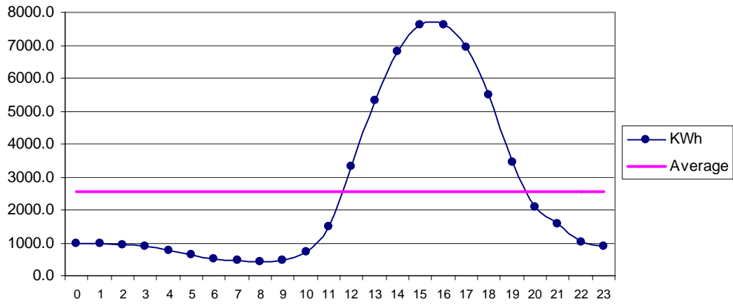
Fig 27 Makola Apr: Diurnal Variation of Wind Genrated Electric Energy Output
