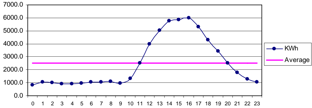
Fig 30 Makola July: Diurnal Variation of Wind Genrated Electric Energy Output
