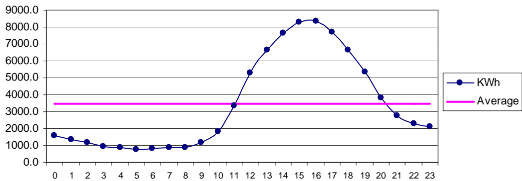
Fig 28 Makola May: Diurnal Variation of Wind Genrated Electric Energy Output
