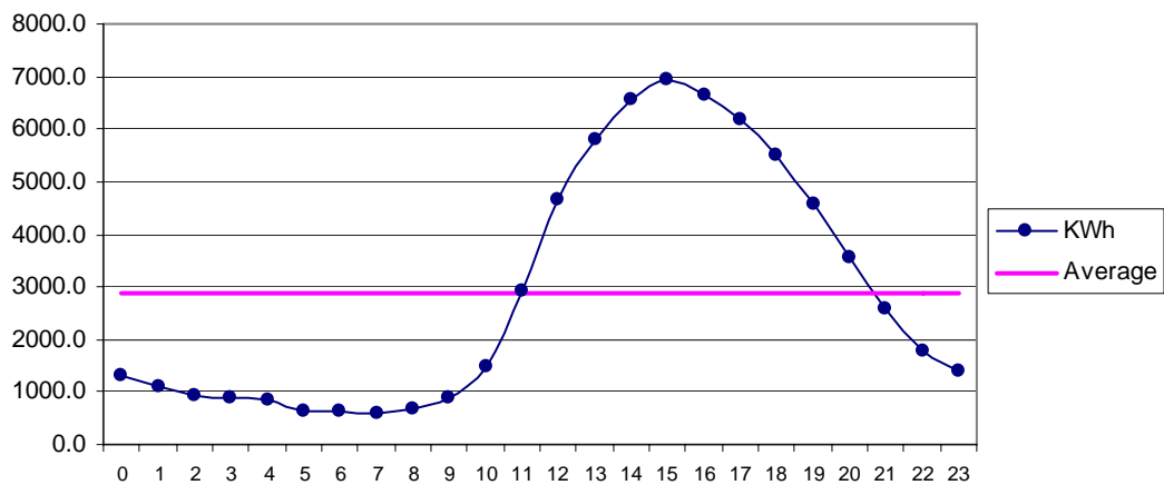
Fig 29 Makola Jun: Diurnal Variation of Wind Genrated Electric Energy Output
