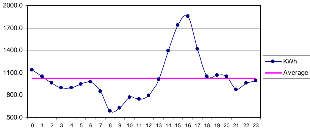
Fig 35 Makola Dec: Diurnal Variation of Wind Genrated Electric Energy Output
