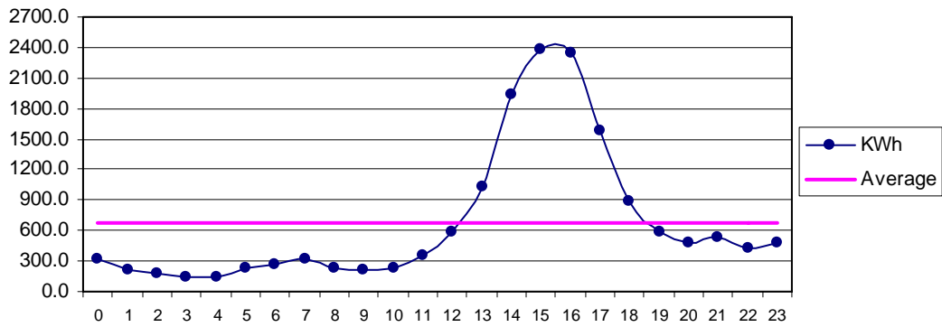
Fig 34 Makola Nov: Diurnal Variation of Wind Genrated Electric Energy Output
