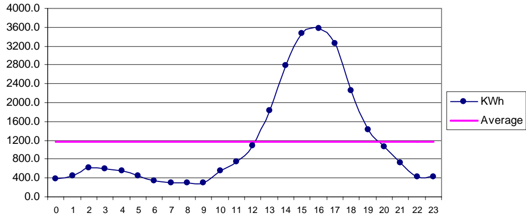
Fig 25 Makola Feb: Diurnal Variation of Wind Genrated Electric Energy Output
