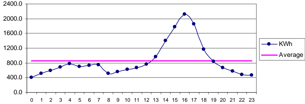
Fig 24 Makola Jan: Diurnal Variation of Wind Genrated Electric Energy Output
