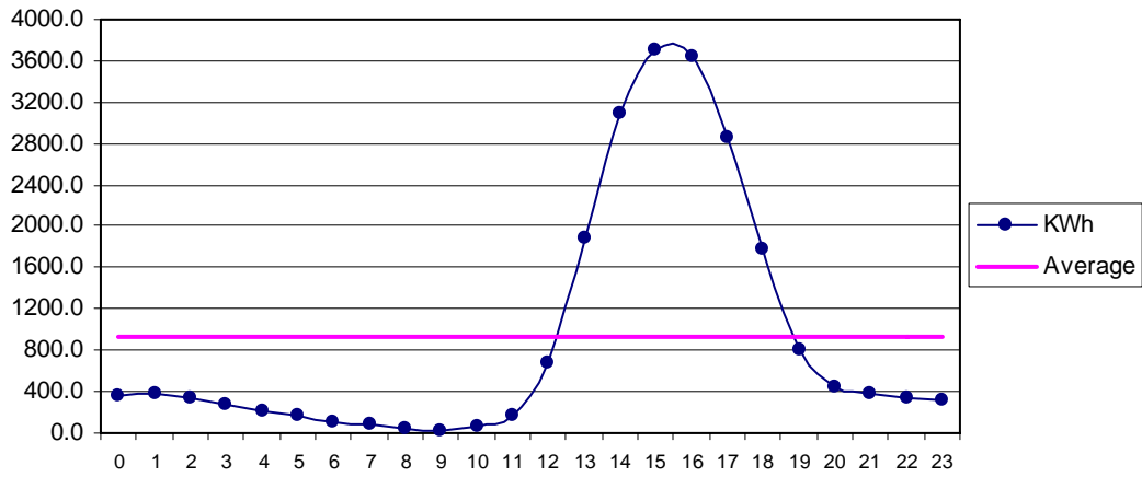
Fig 33 Makola Oct: Diurnal Variation of Wind Genrated Electric Energy Output
