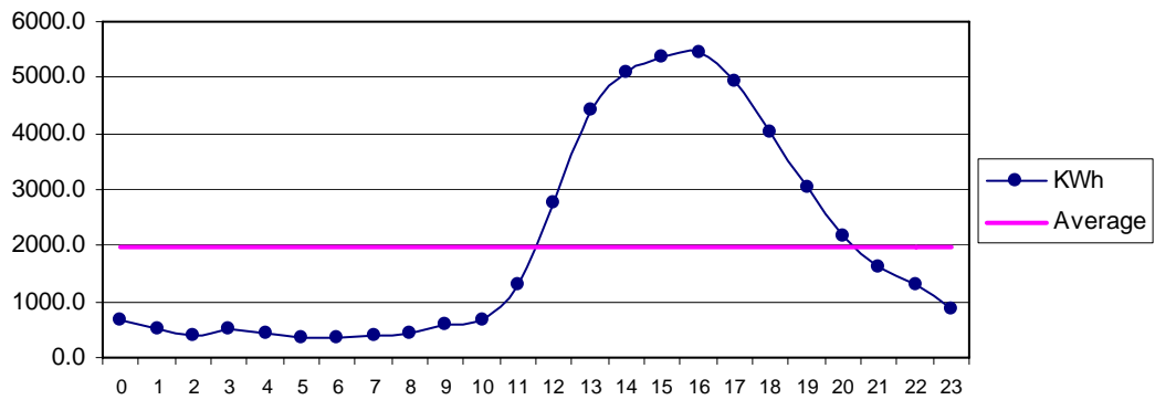
Fig 32 Makola Sep: Diurnal Variation of Wind Genrated Electric Energy Output
