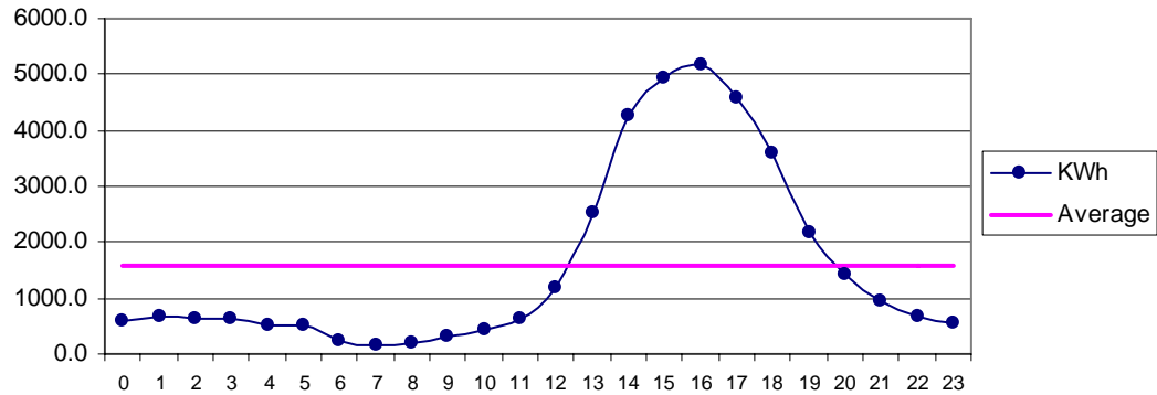
Fig 26 Makola Mar: Diurnal Variation of Wind Genrated Electric Energy Output
