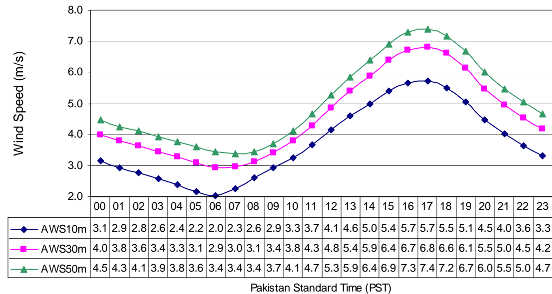
Fig-5 Diurnal Variation of Wind Speed at Jiwani (Jun to Aug) in three Years
