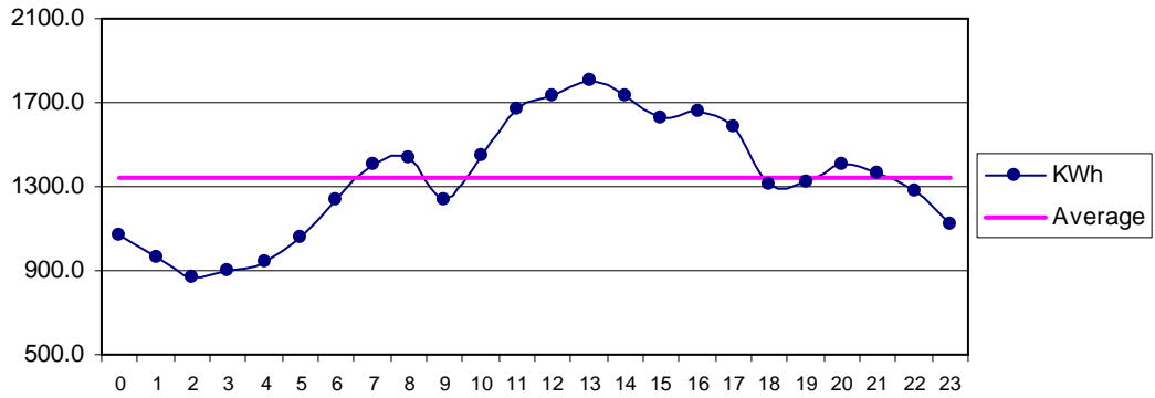
Fig 34 Jiwani Nov: Diurnal Variation of Wind Genrated Electric Energy Output
