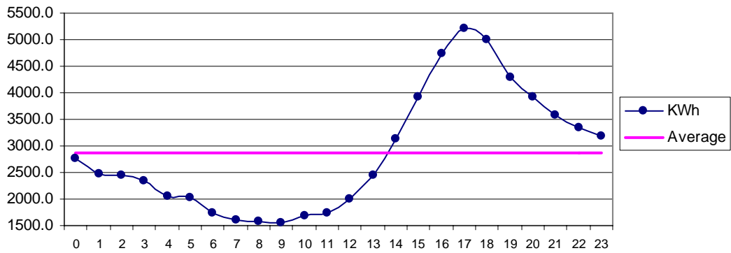
Fig 26 Jiwani Mar: Diurnal Variation of Wind Genrated Electric Energy Output
