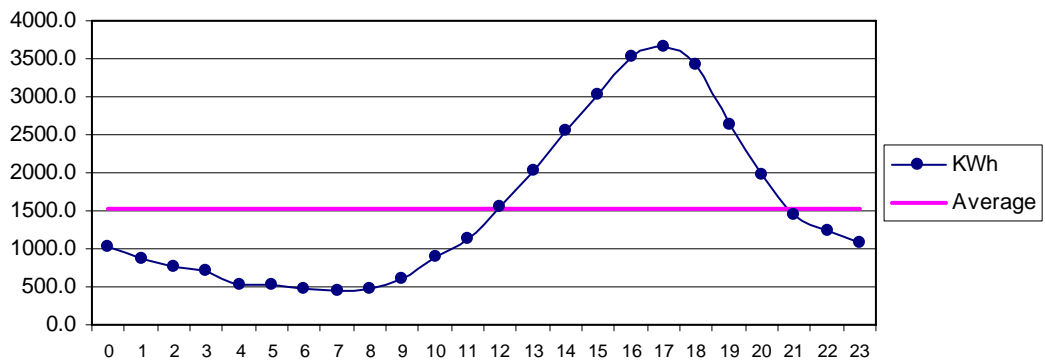
Fig 32 Jiwani Sep: Diurnal Variation of Wind Genrated Electric Energy Output
