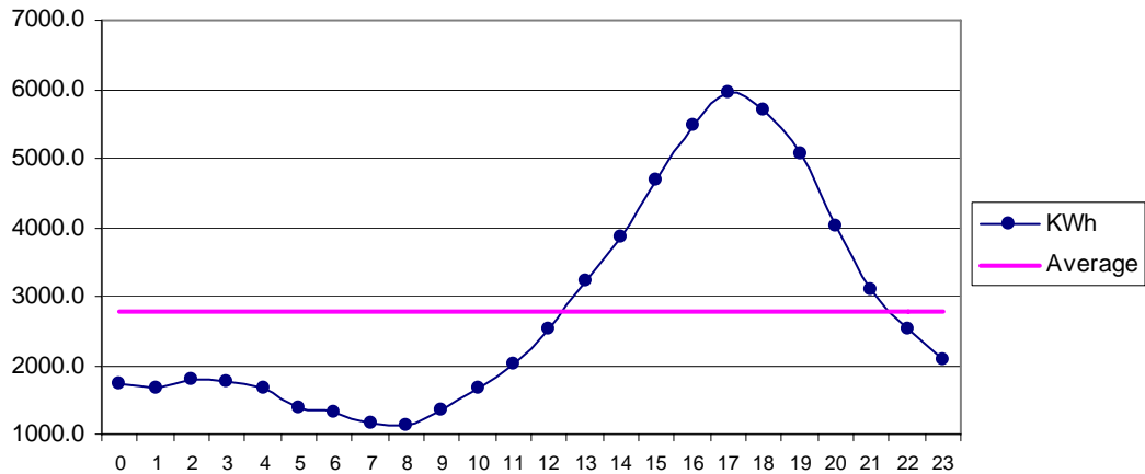
Fig 29 Jiwani Jun: Diurnal Variation of Wind Genrated Electric Energy Output
