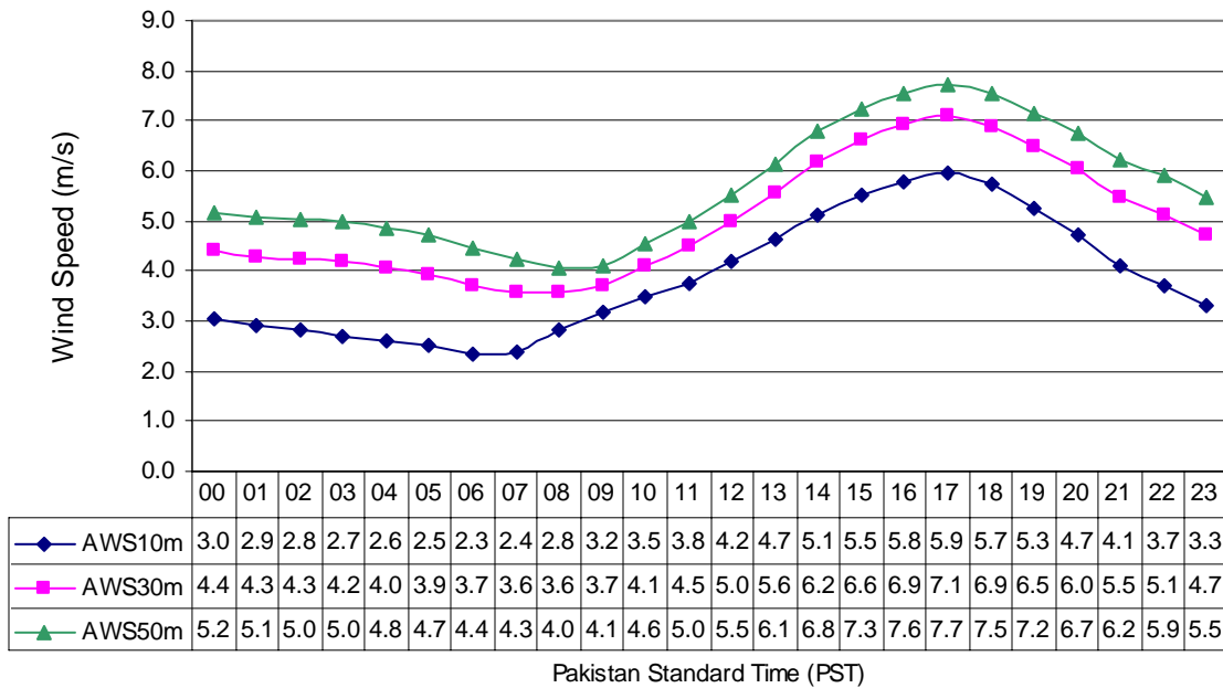
Fig-4 Diurnal Variation of Wind Speed at Jiwani (Mar to May) in three Years
