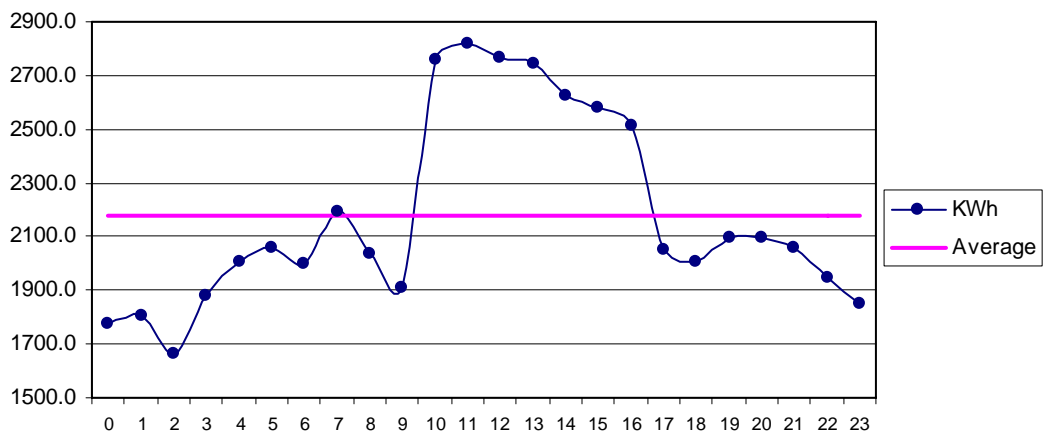
Fig 35 Jiwani Dec: Diurnal Variation of Wind Genrated Electric Energy Output
