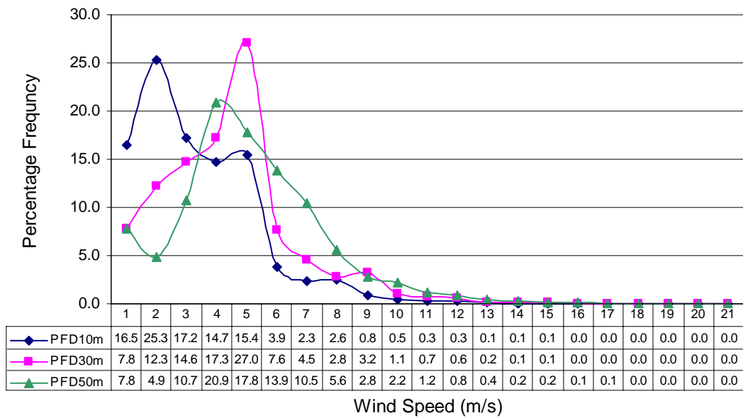
Percentage Wind Frequency Distribution at Jiwani (Dec to Feb) in three years
