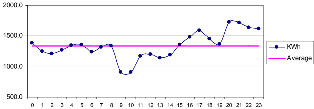
Fig 24 Jiwani Jan: Diurnal Variation of Wind Genrated Electric Energy Output
