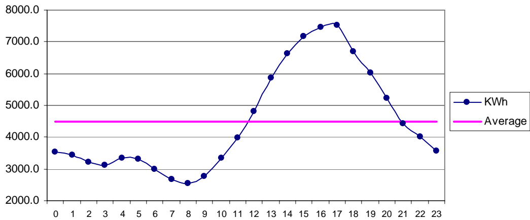
Fig 27 Jiwani Apr: Diurnal Variation of Wind Genrated Electric Energy Output
