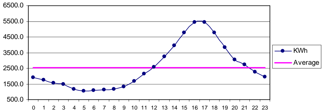
Fig 30 Jiwani July: Diurnal Variation of Wind Genrated Electric Energy Output
