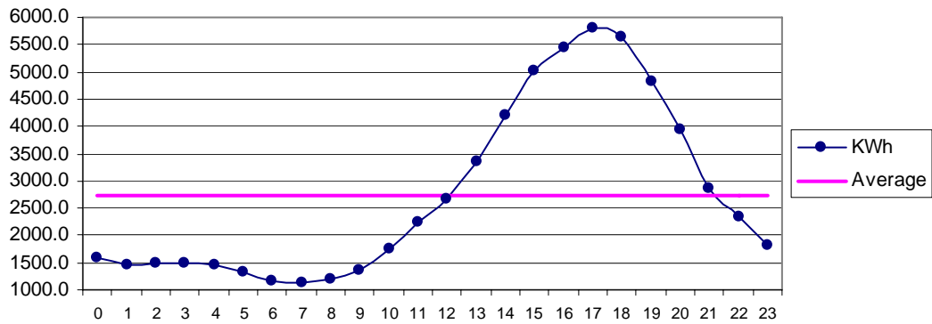
Fig 28 Jiwani May: Diurnal Variation of Wind Genrated Electric Energy Output
