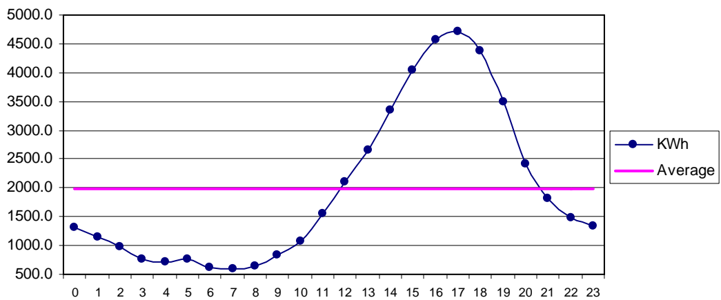
Fig 31 Jiwani Aug: Diurnal Variation of Wind Genrated Electric Energy Output
