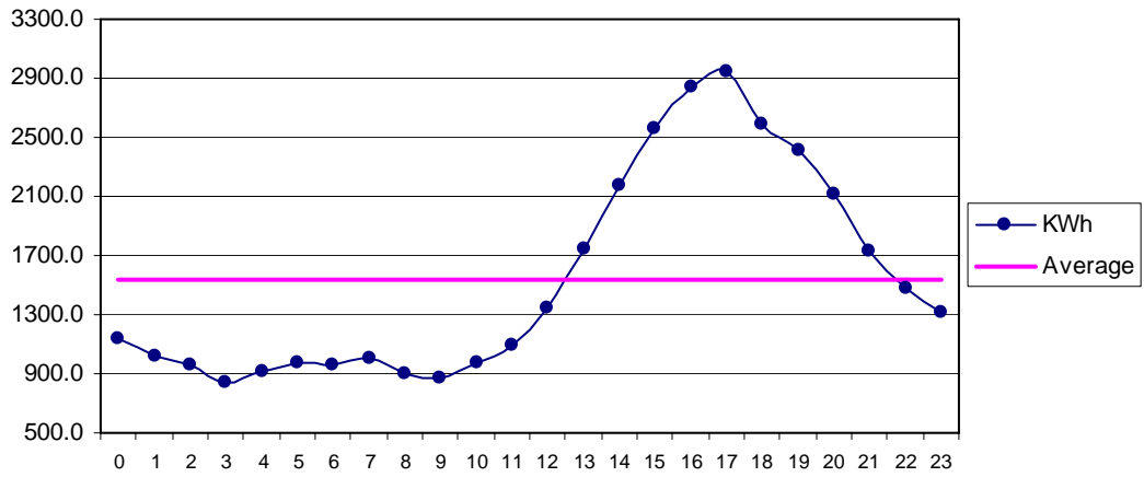
Fig 33 Jiwani Oct: Diurnal Variation of Wind Genrated Electric Energy Output
