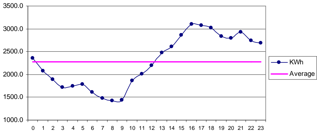
Fig 25 Jiwani Feb: Diurnal Variation of Wind Genrated Electric Energy Output
