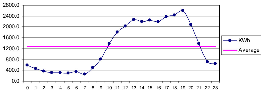
Fig 34 Hoshab Nov: Diurnal Variation of Wind Genrated Electric Energy Output
