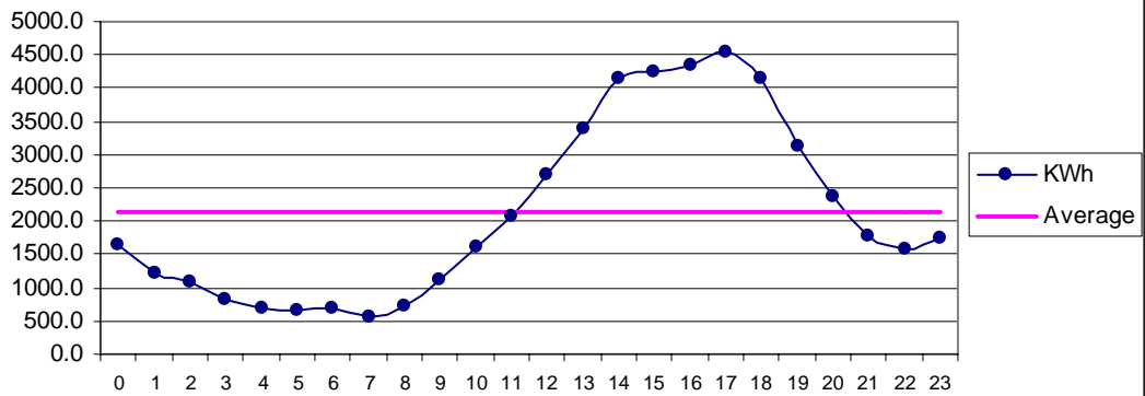
Fig 26 Hoshab Mar: Diurnal Variation of Wind Genrated Electric Energy Output
