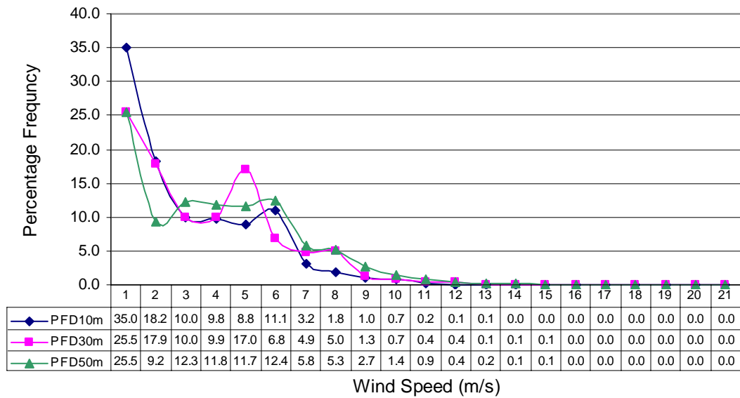
Percentage Wind Frequency Distribution at Hoshab (Sep to Nov) in three years
