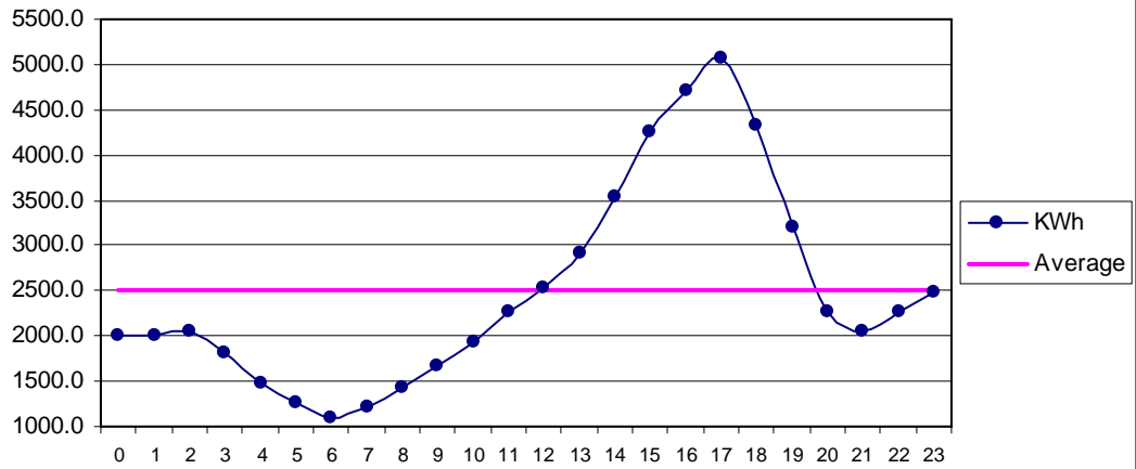
Fig 31 Hoshab Aug: Diurnal Variation of Wind Genrated Electric Energy Output
