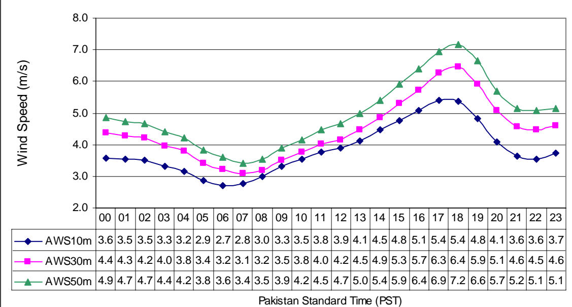
Diurnal Variation of Wind Speed at Hoshab (Jun to Aug) in three Years
