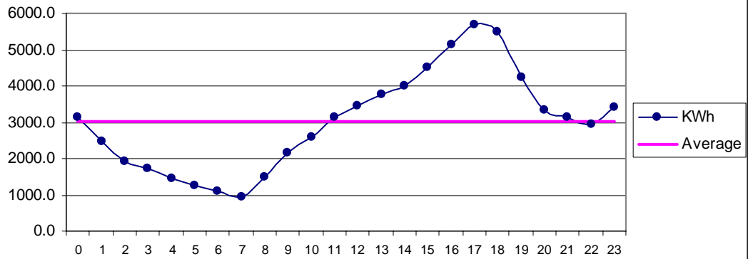
Fig 28 Hoshab May: Diurnal Variation of Wind Genrated Electric Energy Output
