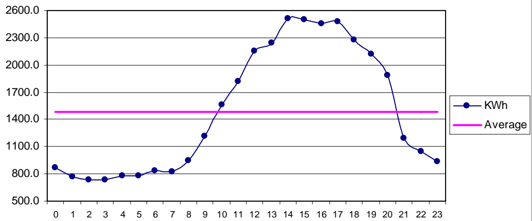
Fig 35 Hoshab Dec: Diurnal Variation of Wind Genrated Electric Energy Output
