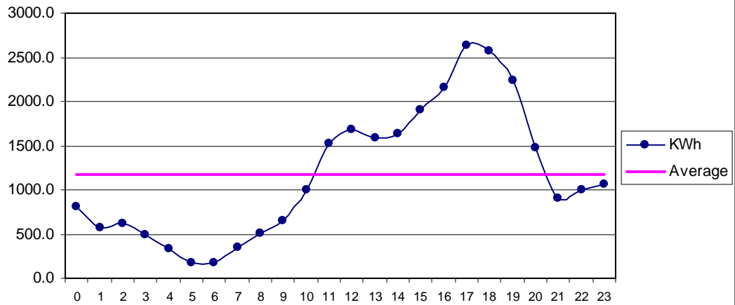
Fig 33 Hoshab Oct: Diurnal Variation of Wind Genrated Electric Energy Output
