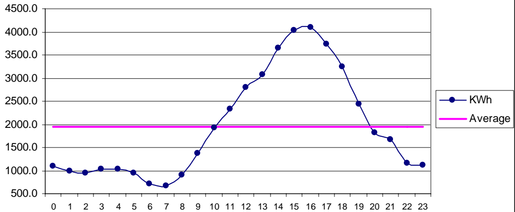
Fig 25 Hoshab Feb: Diurnal Variation of Wind Genrated Electric Energy Output
