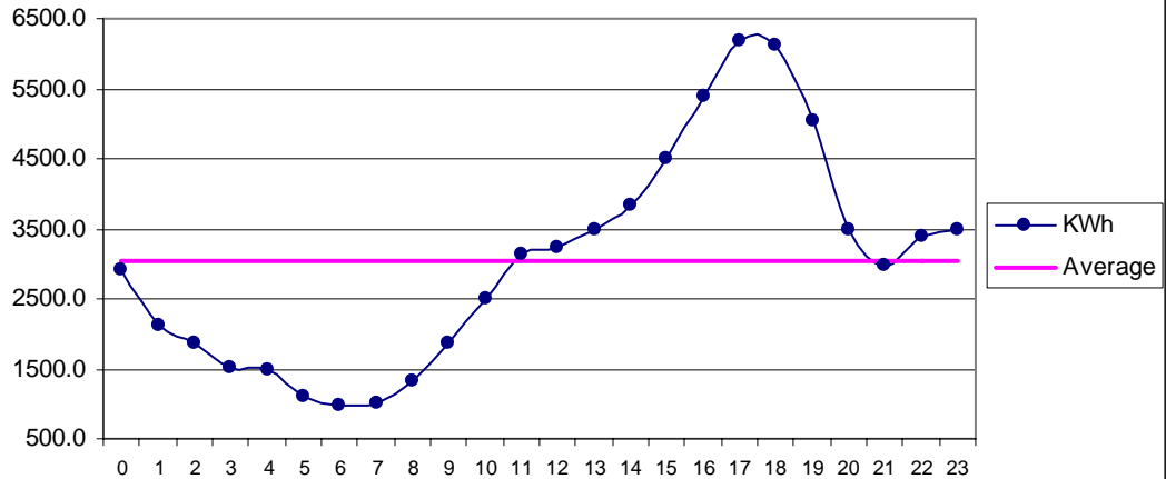
Fig 29 Hoshab Jun: Diurnal Variation of Wind Genrated Electric Energy Output
