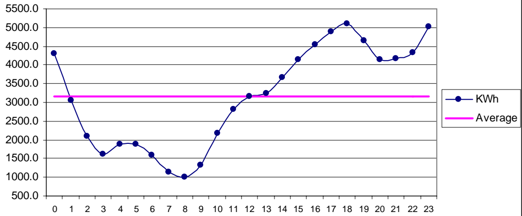
Fig 27 Hoshab Apr: Diurnal Variation of Wind Genrated Electric Energy Output
