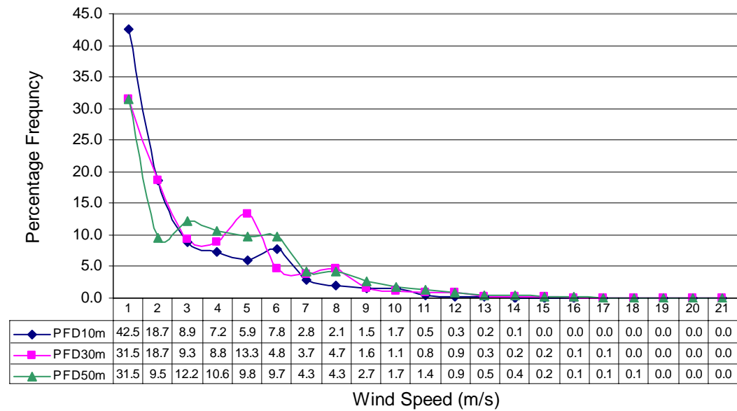
Percentage Wind Frequency Distribution at Hoshab (Dec to Feb) in three years
