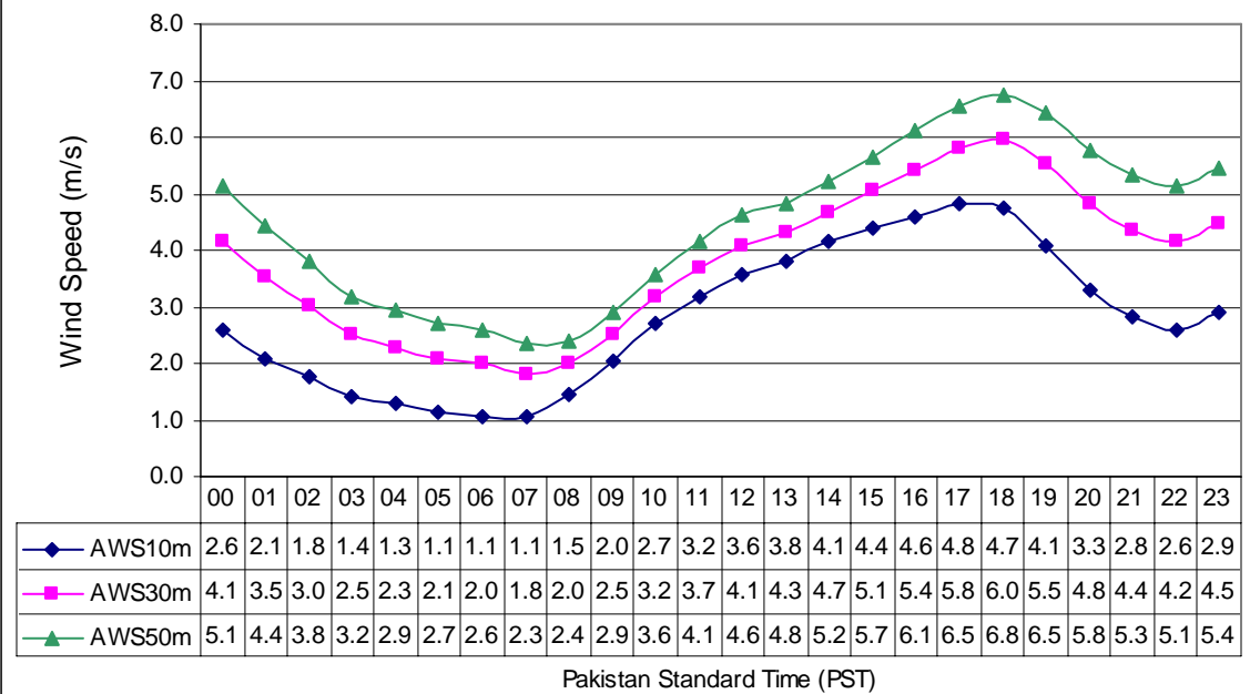
Diurnal Variation of Wind Speed at Hoshab (Mar to May) in three Years
