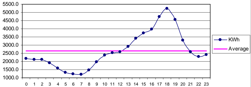
Fig 30 Hoshab July: Diurnal Variation of Wind Genrated Electric Energy Output
