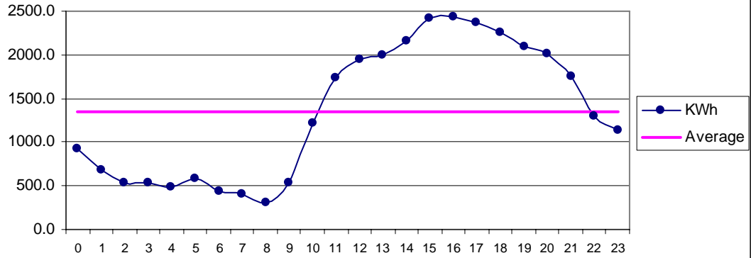
Fig 24 Hoshab Jan: Diurnal Variation of Wind Genrated Electric Energy Output
