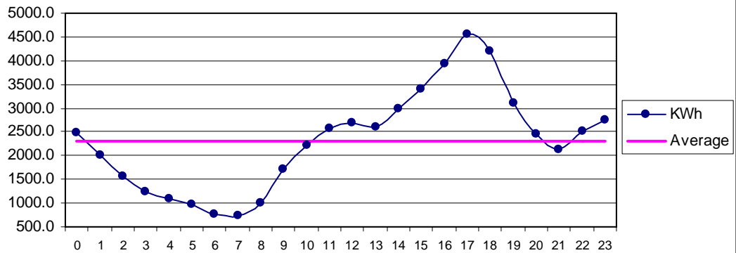
Fig 32 Hoshab Sep: Diurnal Variation of Wind Genrated Electric Energy Output
