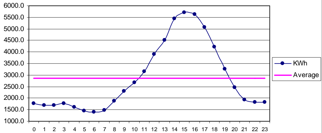
Fig 31 Gawadar Aug: Diurnal Variation of Wind Genrated Electric Energy Output
