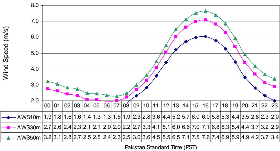
Fig-5 Diurnal Variation of Wind Speed at Gawadar (Jun to Aug) in three Years
