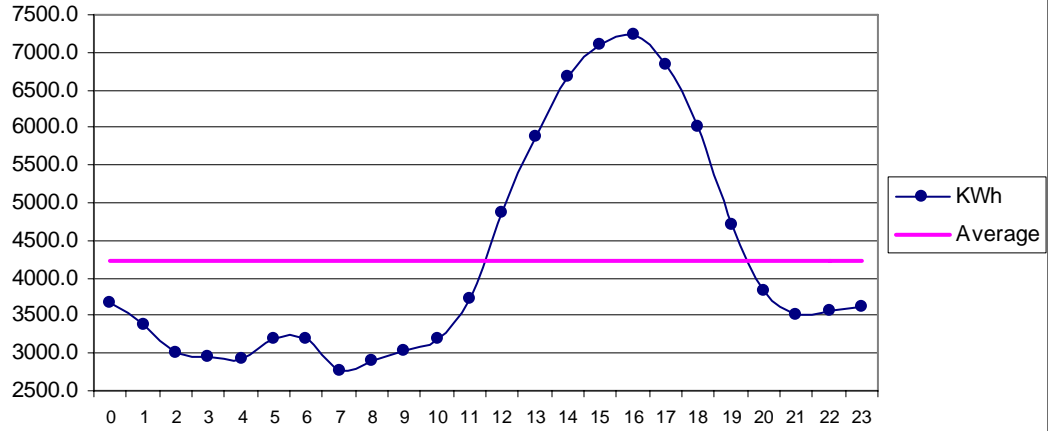
Fig 27 Gawadar Apr: Diurnal Variation of Wind Genrated Electric Energy Output
