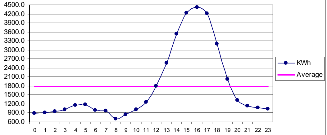
Fig 33 Gawadar Oct: Diurnal Variation of Wind Genrated Electric Energy Output
