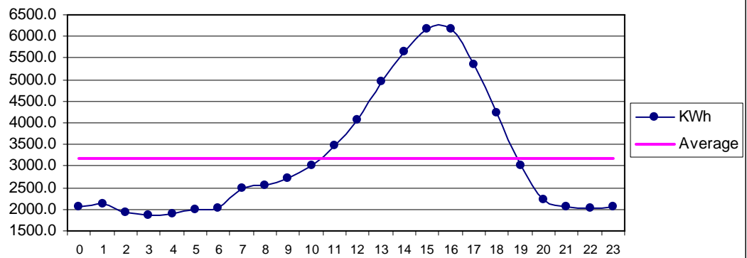
Fig 32 Gawadar Sep: Diurnal Variation of Wind Genrated Electric Energy Output
