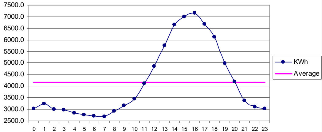
Fig 29 Gawadar Jun: Diurnal Variation of Wind Genrated Electric Energy Output
