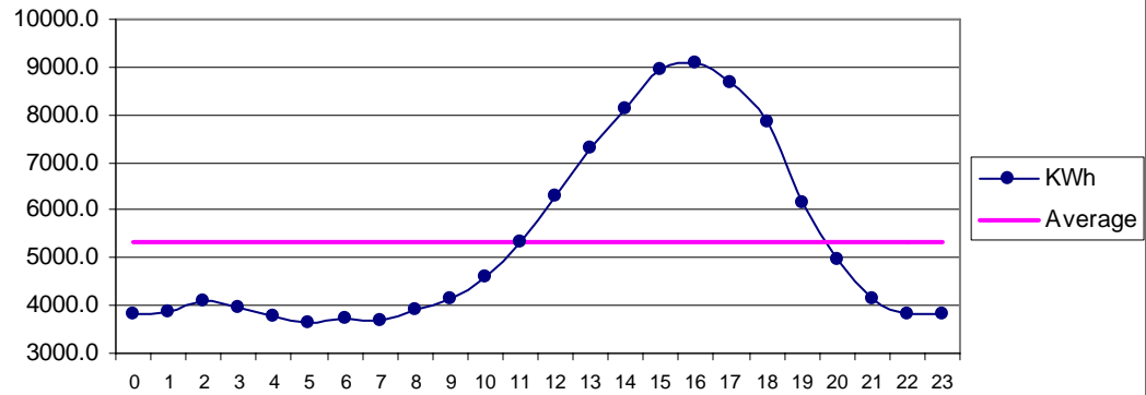
Fig 28 Gawadar May: Diurnal Variation of Wind Genrated Electric Energy Output
