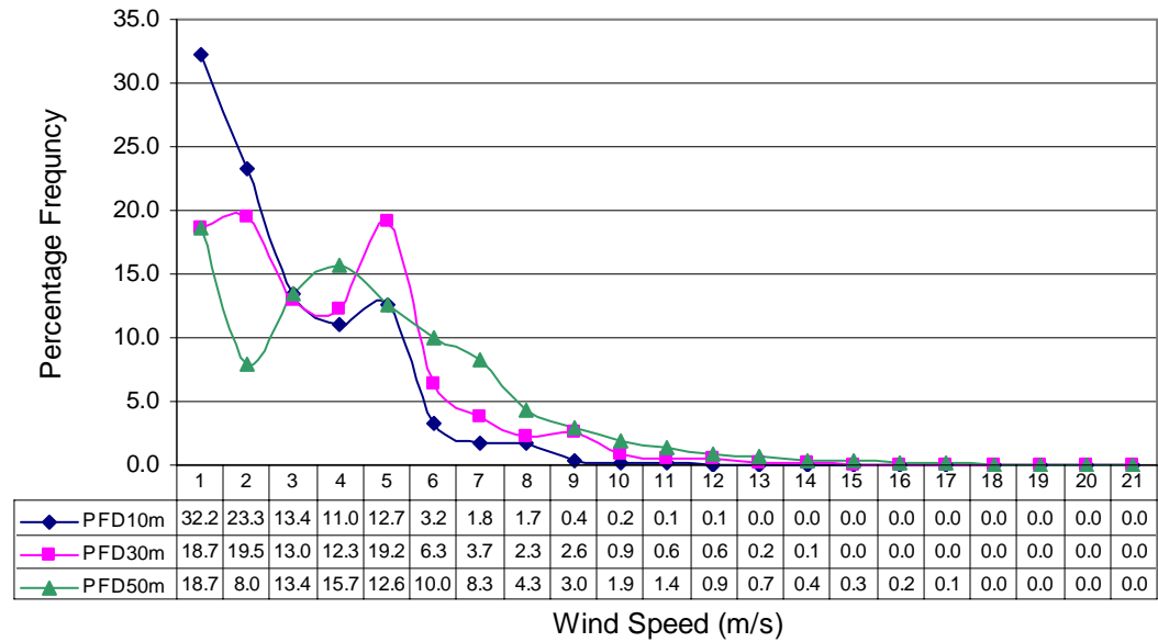
Percentage Wind Frequency Distribution at Gawadar (Dec to Feb) in three years
