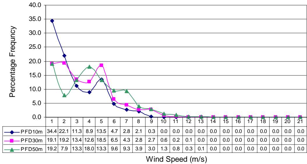
Percentage Wind Frequency Distribution at Gawadar (Sep to Nov) in three years
