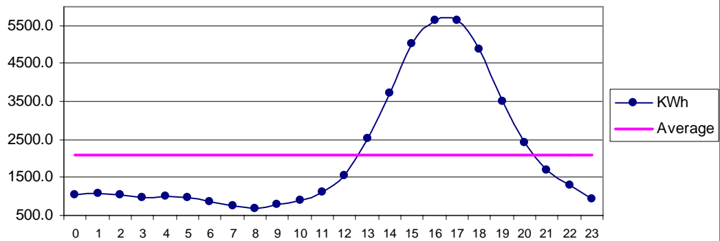
Fig 26 Gawadar Mar: Diurnal Variation of Wind Genrated Electric Energy Output
