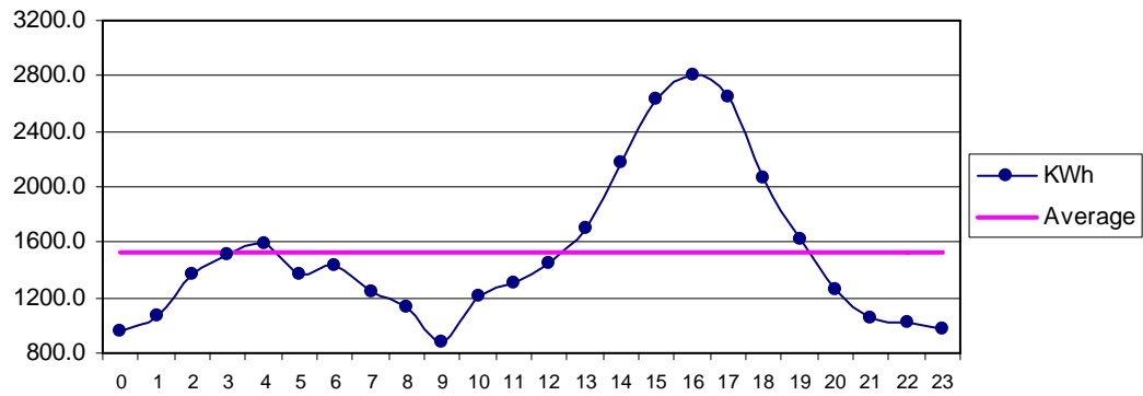
Fig 34 Gawadar Nov: Diurnal Variation of Wind Genrated Electric Energy Output
