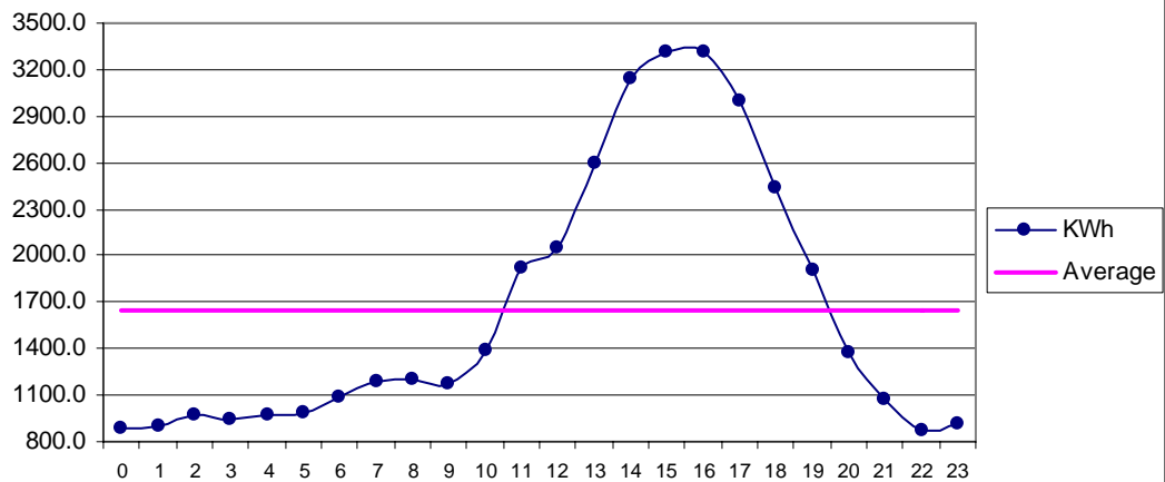
Fig 25 Gawadar Feb: Diurnal Variation of Wind Genrated Electric Energy Output
