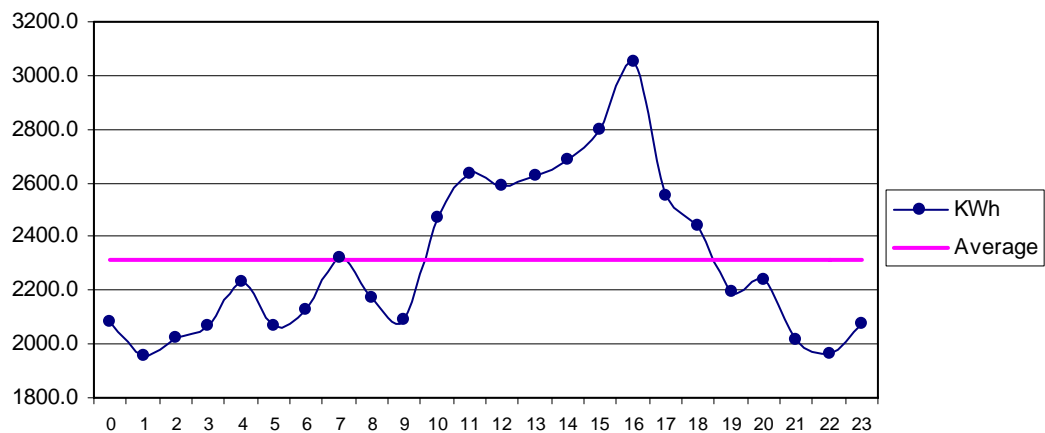
Fig 35 Gawadar Dec: Diurnal Variation of Wind Genrated Electric Energy Output
