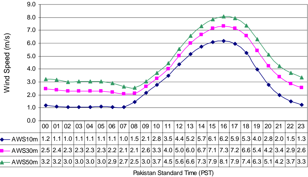
Fig-4 Diurnal Variation of Wind Speed at Gawadar (Mar to May) in three Years
