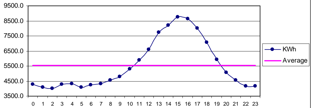
Fig 30 Gawadar July: Diurnal Variation of Wind Genrated Electric Energy Output
