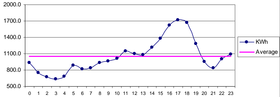
Fig 24 Gawadar Jan: Diurnal Variation of Wind Genrated Electric Energy Output
