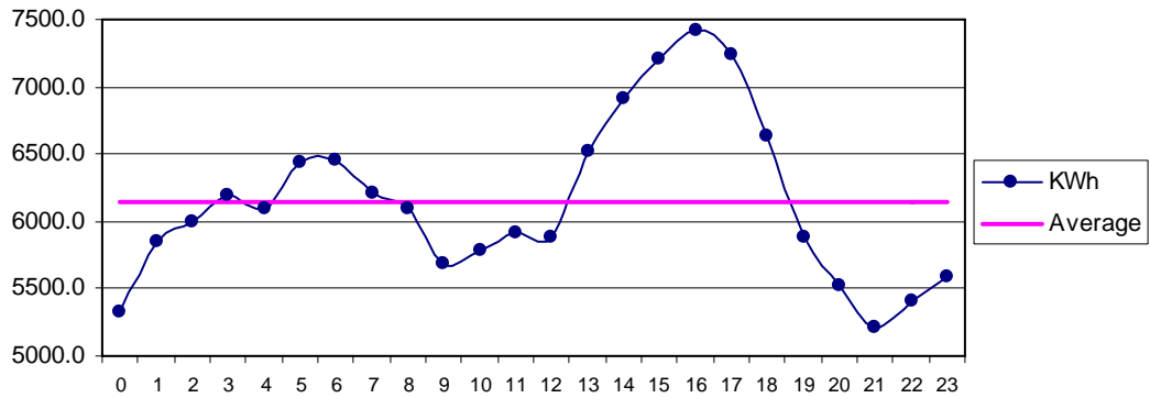
Fig 30 Gaddani July: Diurnal Variation of Wind Genrated Electric Energy Output
