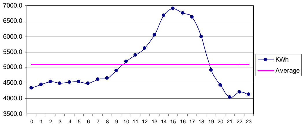
Fig 31 Gaddani Aug: Diurnal Variation of Wind Genrated Electric Energy Output
