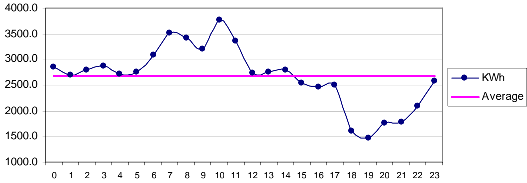
Fig 24 Gaddani Jan: Diurnal Variation of Wind Genrated Electric Energy Output
