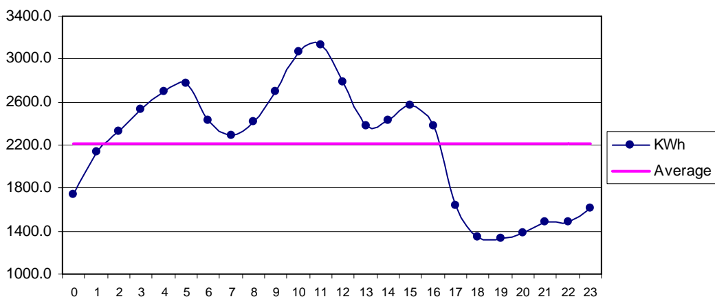
Fig 35 Gaddani Dec: Diurnal Variation of Wind Genrated Electric Energy Output
