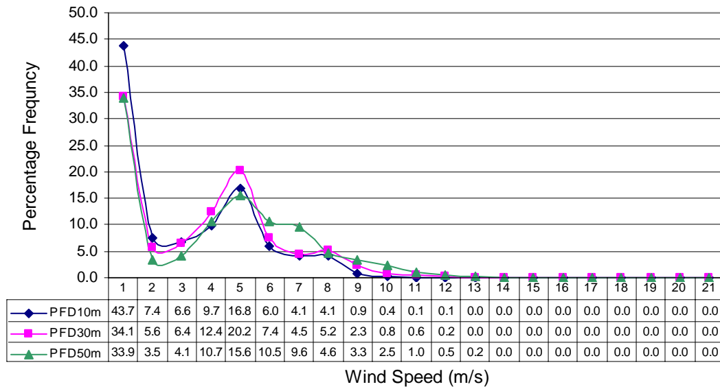
Percentage Wind Frequency Distribution at Gaddani (Sep to Nov) in three years
