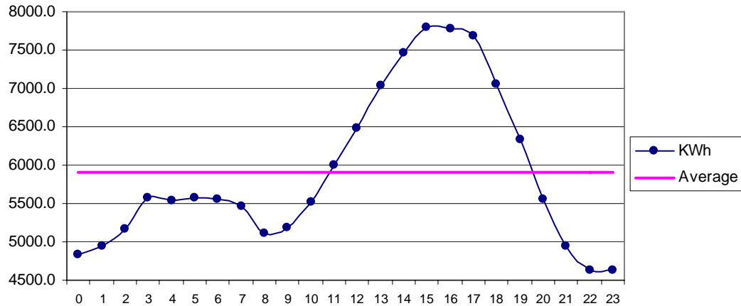
Fig 29 Gaddani Jun: Diurnal Variation of Wind Genrated Electric Energy Output
