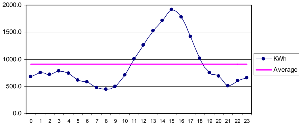
Fig 33 Gaddani Oct: Diurnal Variation of Wind Genrated Electric Energy Output
