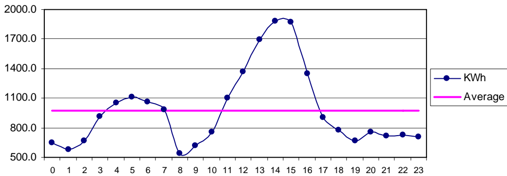
Fig 34 Gaddani Nov: Diurnal Variation of Wind Genrated Electric Energy Output
