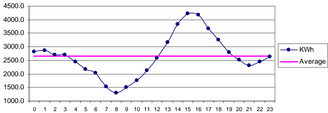
Fig 26 Gaddani Mar: Diurnal Variation of Wind Genrated Electric Energy Output
