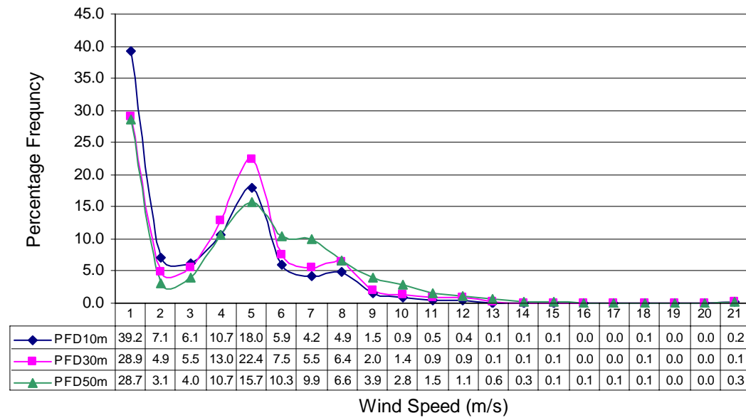
Percentage Wind Frequency Distribution at Gaddani (Dec to Feb) in three years
