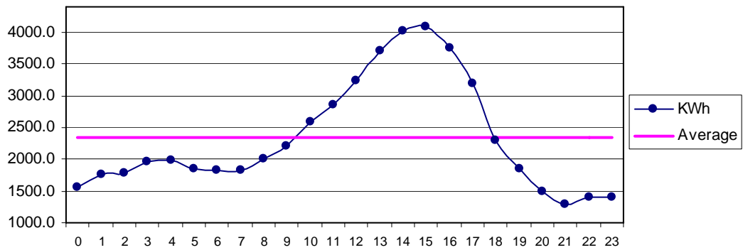
Fig 32 Gaddani Sep: Diurnal Variation of Wind Genrated Electric Energy Output
