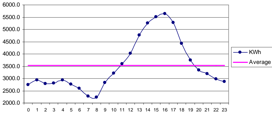
Fig 27 Gaddani Apr: Diurnal Variation of Wind Genrated Electric Energy Output
