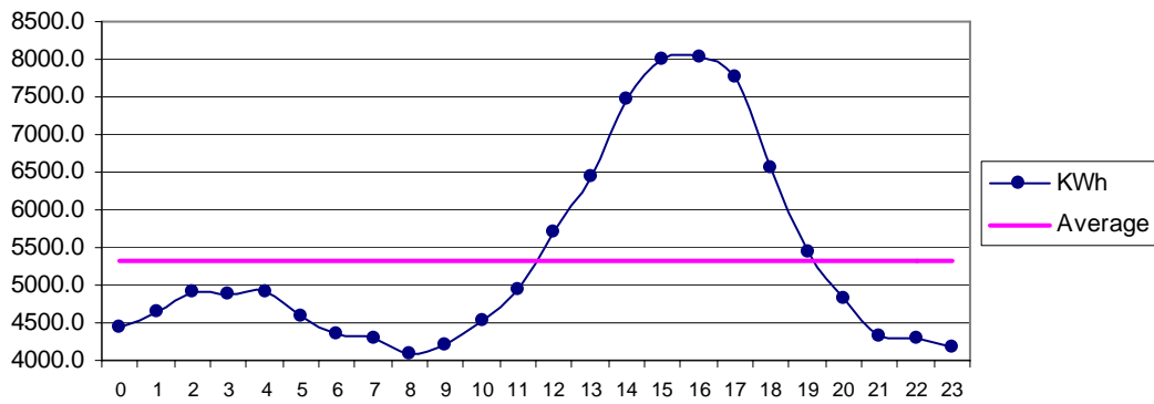
Fig 28 Gaddani May: Diurnal Variation of Wind Genrated Electric Energy Output
