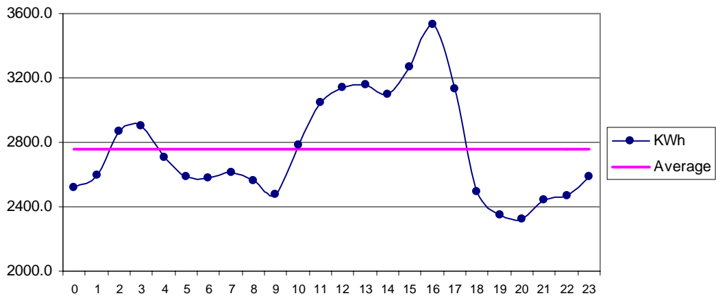
Fig 25 Gaddani Feb: Diurnal Variation of Wind Genrated Electric Energy Output
