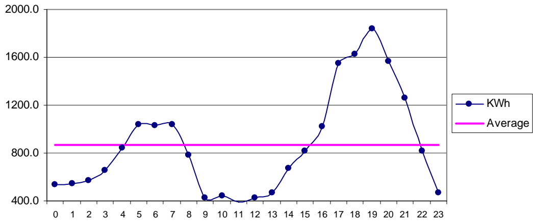
Fig 25 Bella Feb: Diurnal Variation of Wind Genrated Electric Energy Output
