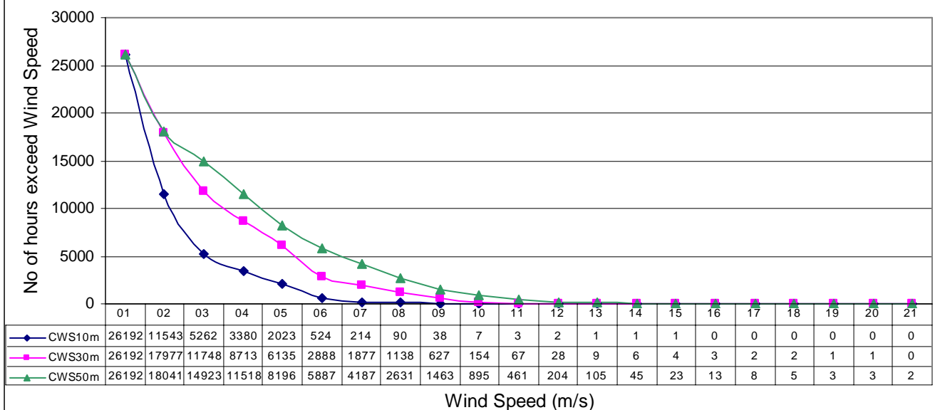
Comulative Wind Speed Distribution at Bella in three years
