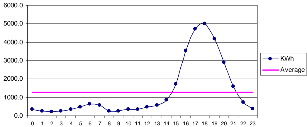
Fig 27 Bella Apr: Diurnal Variation of Wind Genrated Electric Energy Output
