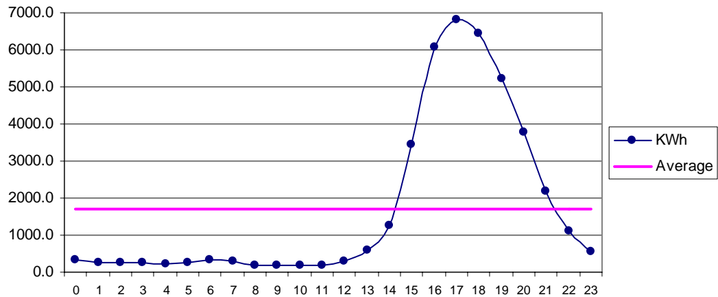
Fig 29 Bella Jun: Diurnal Variation of Wind Genrated Electric Energy Output
