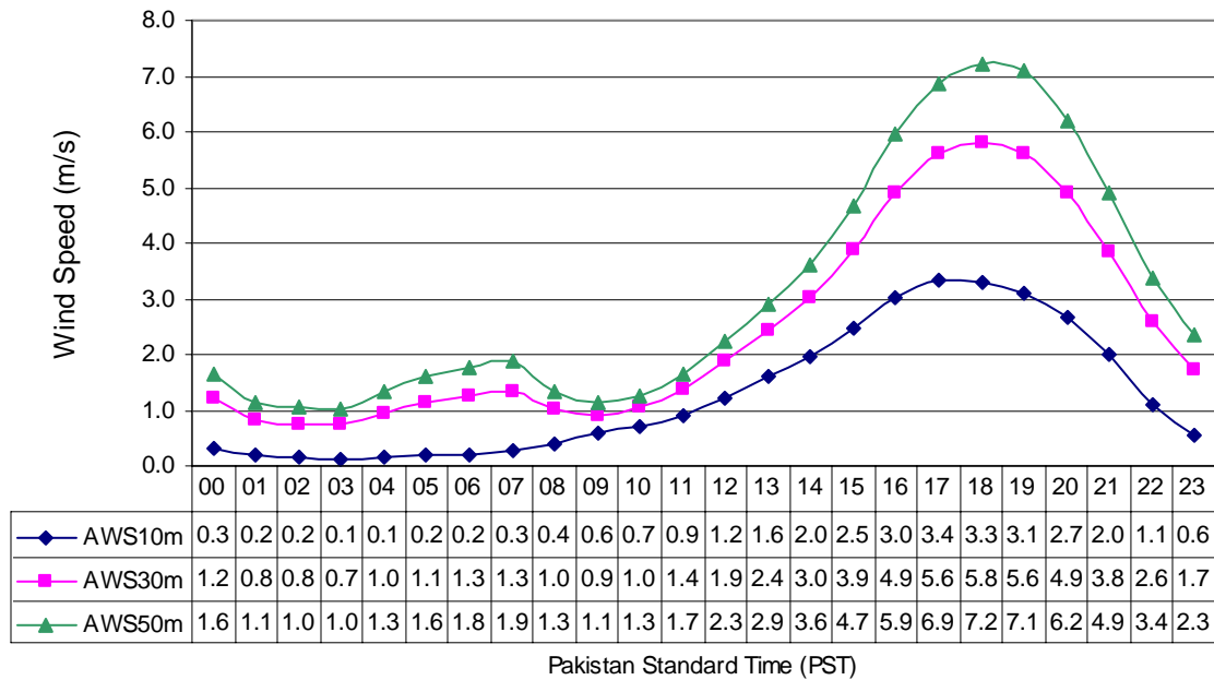
Diurnal Variation of Wind Speed at Bella (Mar to May) in three Years
