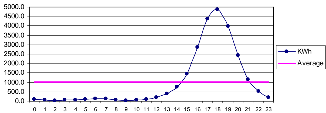
Fig 32 Bella Sep: Diurnal Variation of Wind Genrated Electric Energy Output
