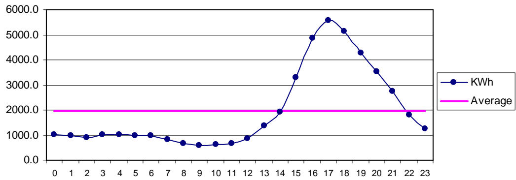
Fig 30 Bella July: Diurnal Variation of Wind Genrated Electric Energy Output
