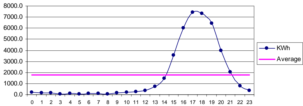
Fig 28 Bella May: Diurnal Variation of Wind Genrated Electric Energy Output
