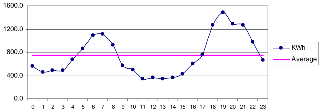
Fig 24 Bella Jan: Diurnal Variation of Wind Genrated Electric Energy Output
