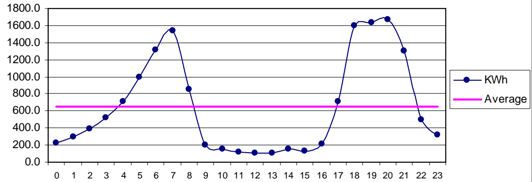
Fig 34 Bella Nov: Diurnal Variation of Wind Genrated Electric Energy Output
