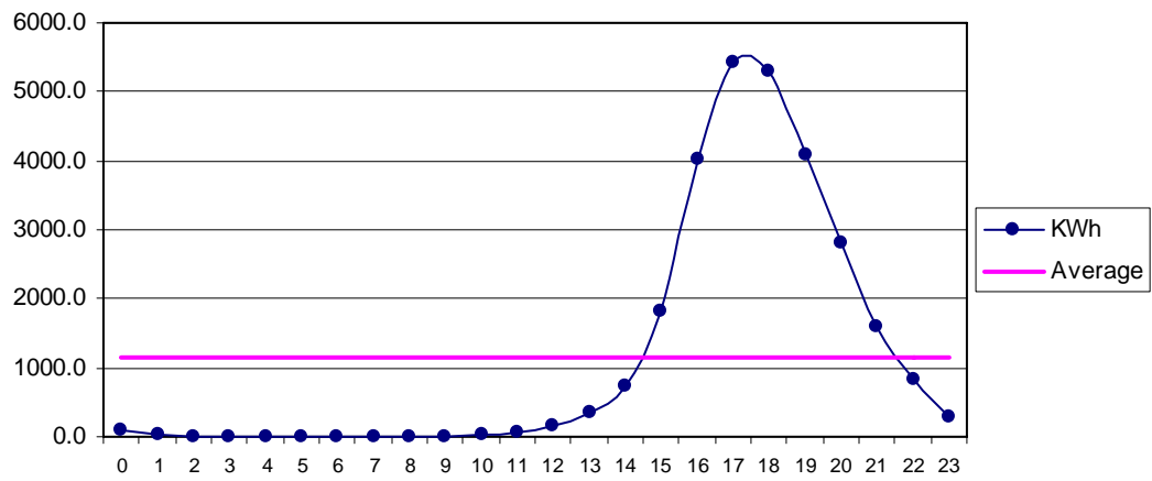
Fig 31 Bella Aug: Diurnal Variation of Wind Genrated Electric Energy Output
