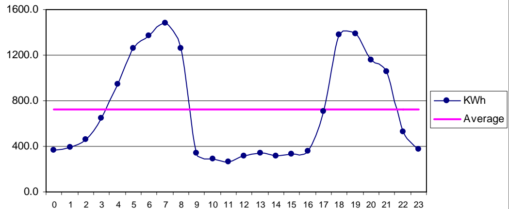
Fig 35 Bella Dec: Diurnal Variation of Wind Genrated Electric Energy Output
