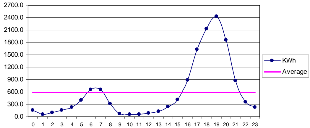
Fig 33 Bella Oct: Diurnal Variation of Wind Genrated Electric Energy Output
