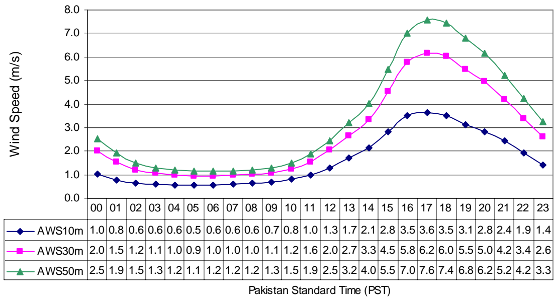
Diurnal Variation of Wind Speed at Bella (Jun to Aug) in three Years
