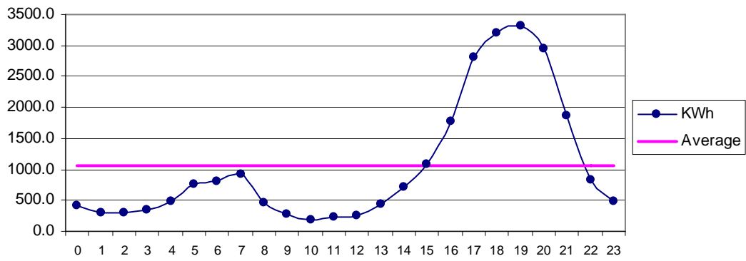
Fig 26 Bella Mar: Diurnal Variation of Wind Genrated Electric Energy Output
