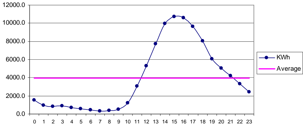
Fig 27 Aghore Apr: Diurnal Variation of Wind Genrated Electric Energy Output
