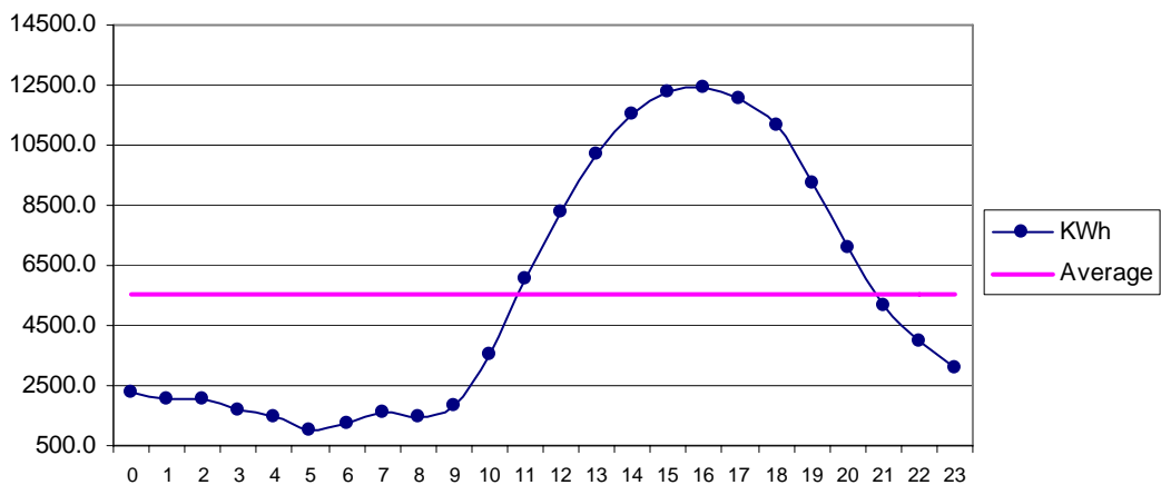
Fig 29 Aghore Jun: Diurnal Variation of Wind Genrated Electric Energy Output
