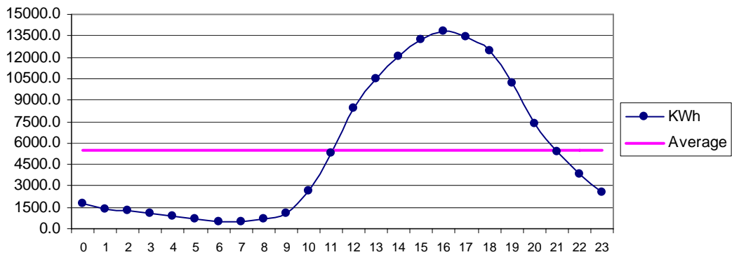
Fig 28 Aghore May: Diurnal Variation of Wind Genrated Electric Energy Output
