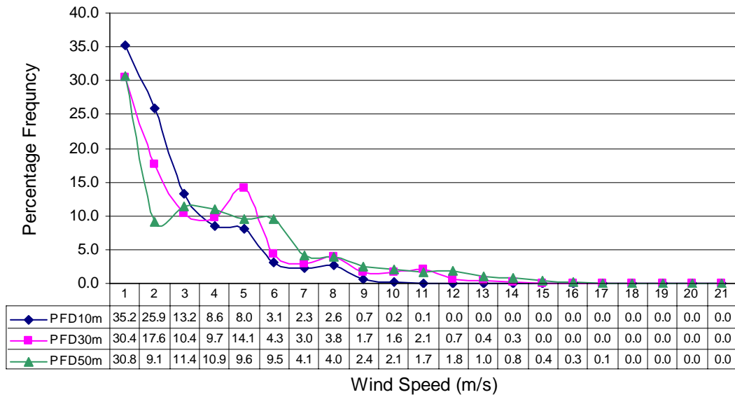
Percentage Wind Frequency Distribution at Aghore (Sep to Nov) in three years
