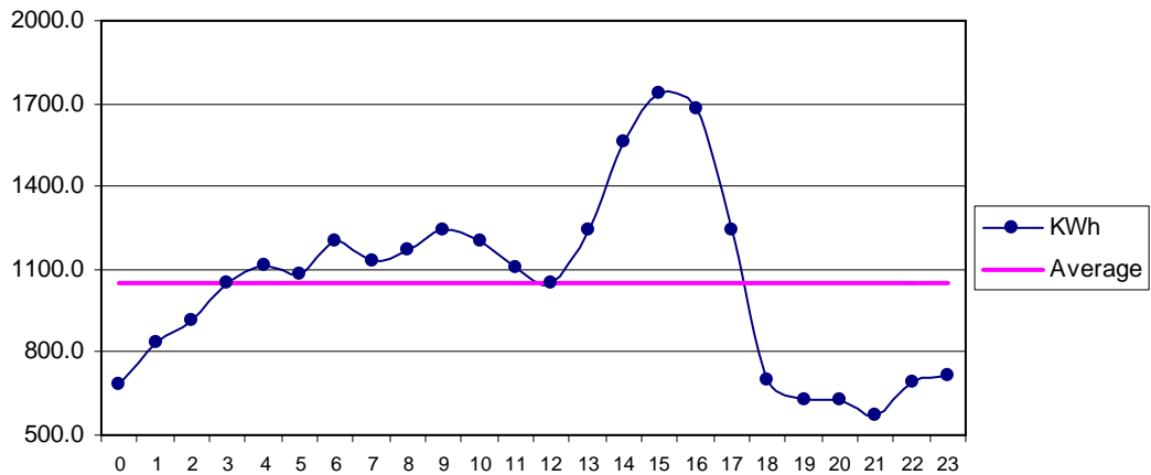
Fig 35 Aghore Dec: Diurnal Variation of Wind Genrated Electric Energy Output
