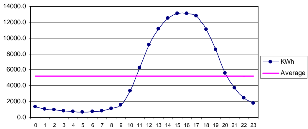
Fig 31 Aghore Aug: Diurnal Variation of Wind Genrated Electric Energy Output
