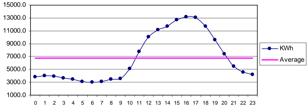
Fig 30 Aghore July: Diurnal Variation of Wind Genrated Electric Energy Output
