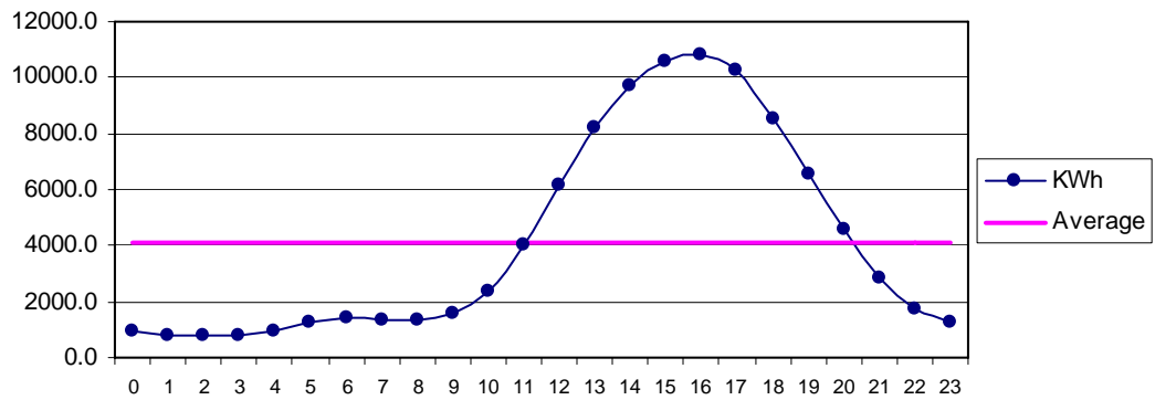
Fig 32 Aghore Sep: Diurnal Variation of Wind Genrated Electric Energy Output
