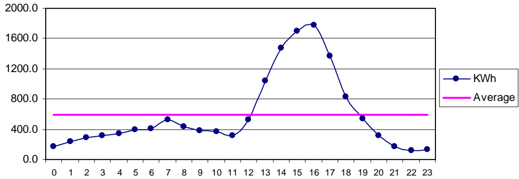
Fig 35 Aghore Dec: Diurnal Variation of Wind Genrated Electric Energy Output
