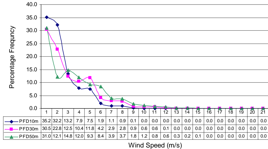
Percentage Wind Frequency Distribution at Aghore (Dec to Feb) in three years
