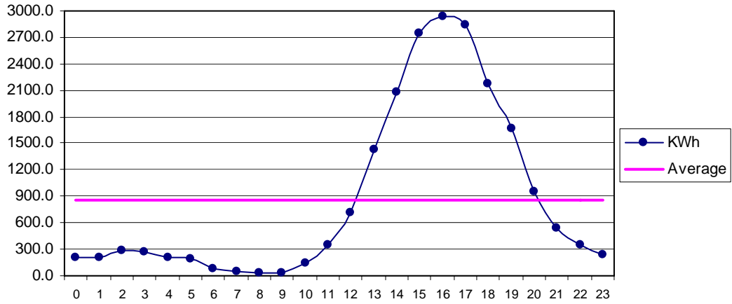
Fig 33 Aghore Oct: Diurnal Variation of Wind Genrated Electric Energy Output
