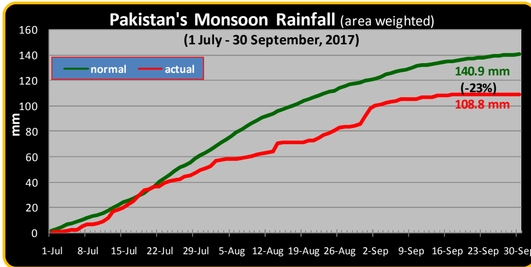
Fig-1: Country cumulative daily actual & normal rainfall
