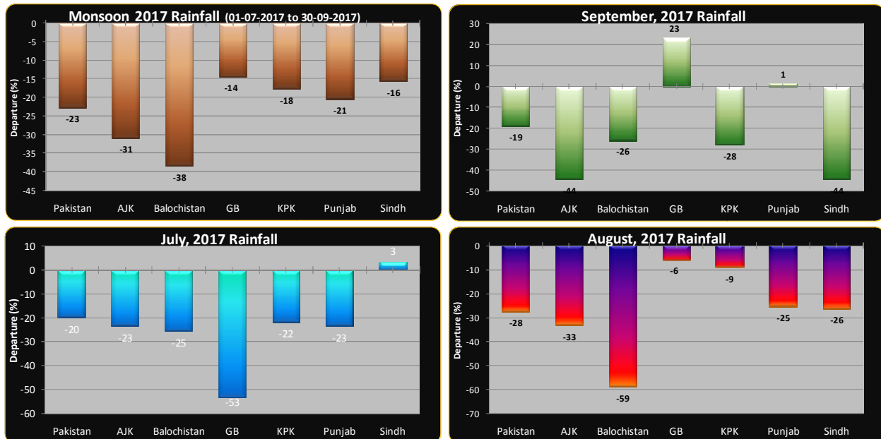
Fig-2: Country's seasonal & monthly rainfall
