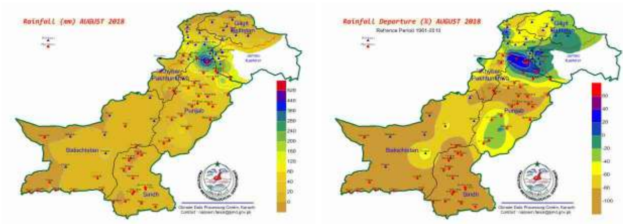
Fig-5: Spatial distribution of August rainfall (actual & percentage departure)
