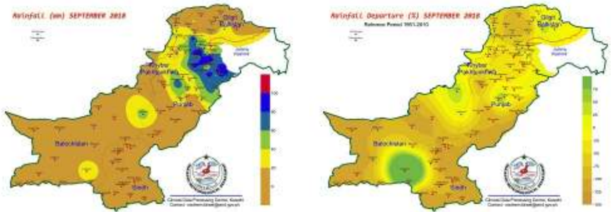
Fig-4: Spatial distribution of September rainfall (actual & percentage departure)
