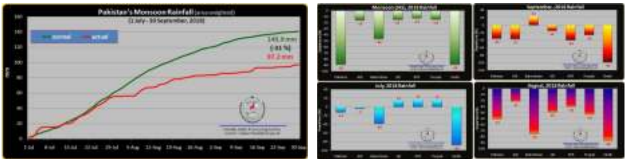
Fig-1: Country season cumulative rainfall (left) & distribution of seasonal & monthly rainfall (right)
