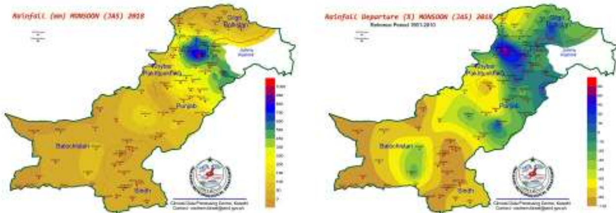
Fig-3: Spatial distribution of Monsoon season rainfall (actual & percentage departure)
