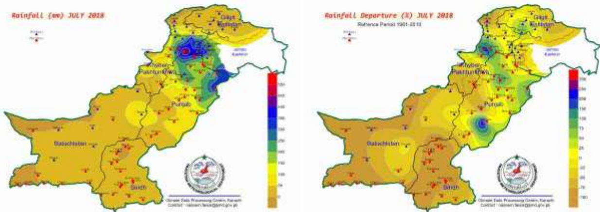
Fig-6: Spatial distribution of July rainfall (actual & percentage departure)
